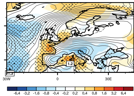
ModE-Sim
