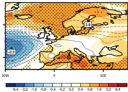
ModE-Sim
