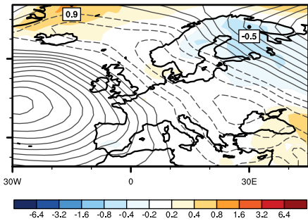
ModE-Sim
