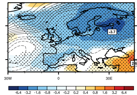
ModE-RAClim
