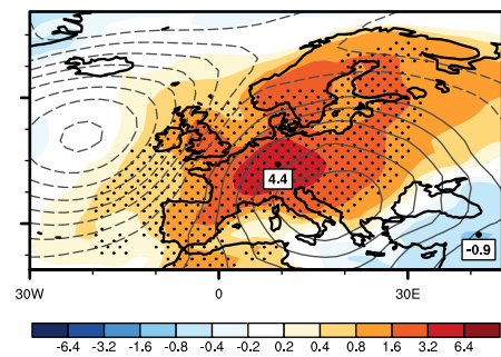
ModE-RAClim
