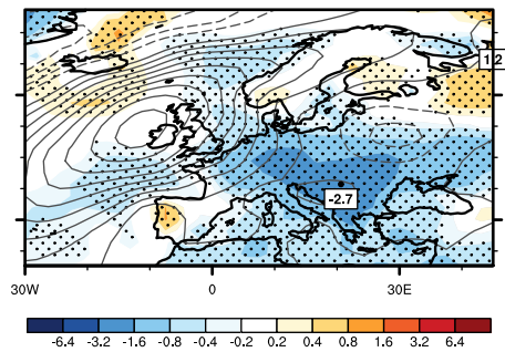
ModE-RAClim
