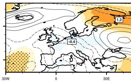
ModE-Sim
