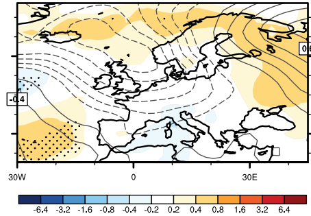
ModE-Sim
