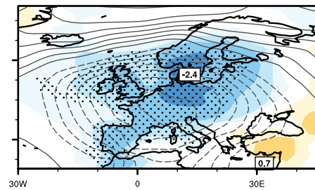
ModE-RAClim
