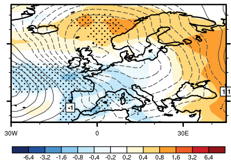
ModE-Sim
