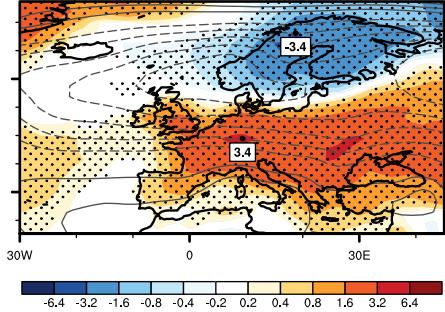
ModE-RAClim
