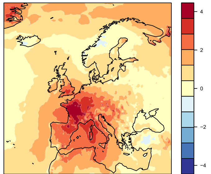
JJA temperature anomaly (K)
