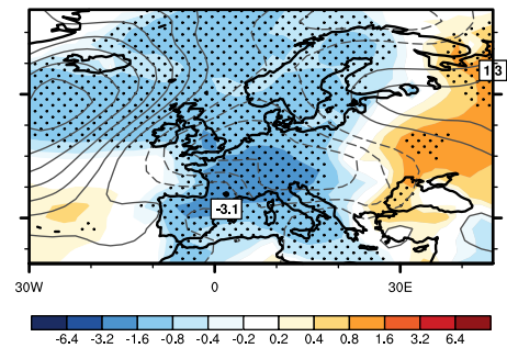
ModE-RAClim
