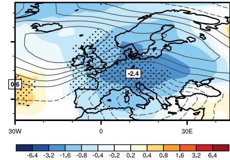
ModE-RAClim
