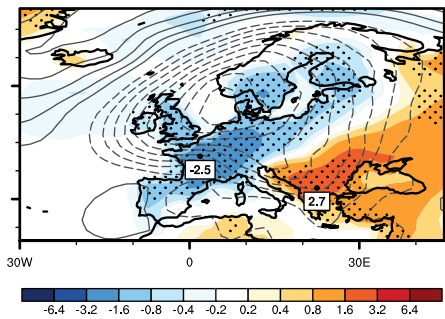
ModE-RAClim
