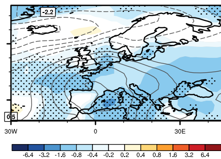
ModE-Sim
