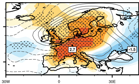
ModE-RAClim
