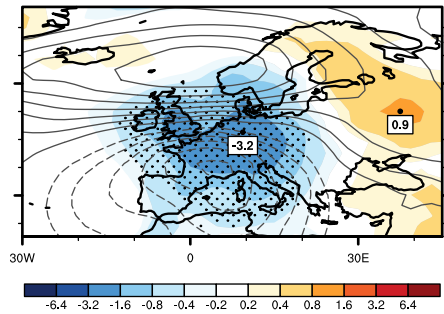
ModE-RAClim
