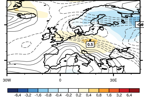
ModE-Sim
