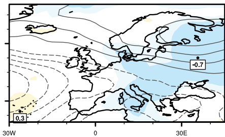
ModE-Sim
