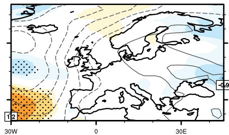
ModE-Sim
