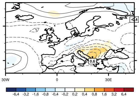
ModE-Sim
