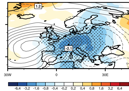
ModE-RAClim
