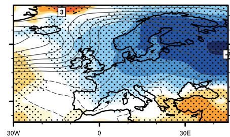
ModE-RAClim
