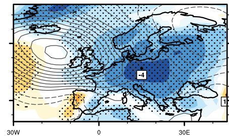
ModE-RAClim
