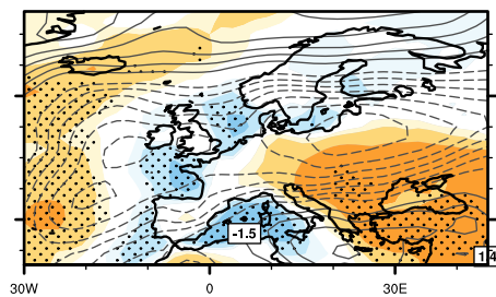
ModE-Sim
