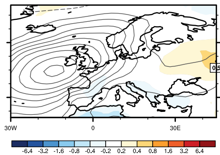
ModE-Sim
