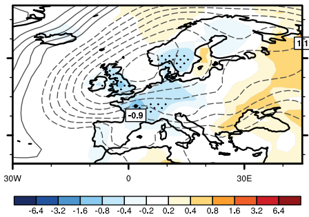
ModE-RAClim
