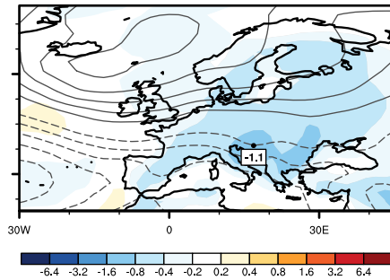
ModE-Sim
