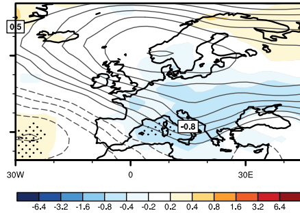
ModE-Sim
