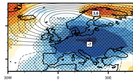
ModE-RAClim
