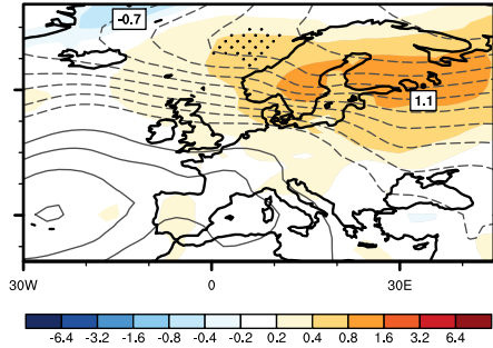
ModE-Sim
