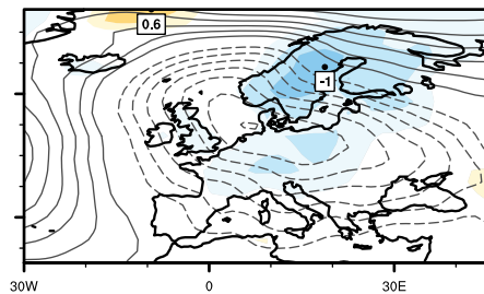
ModE-Sim
