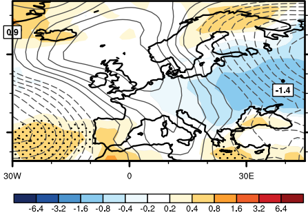
ModE-Sim
