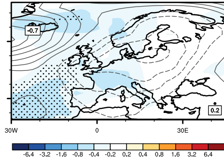
ModE-Sim
