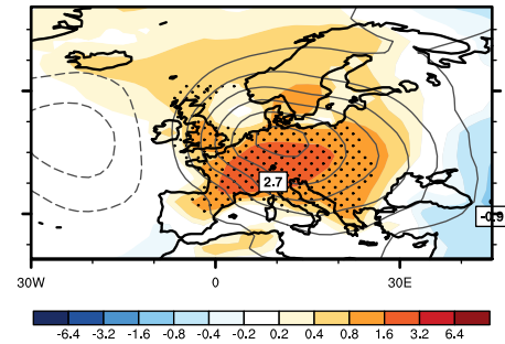
ModE-RAClim
