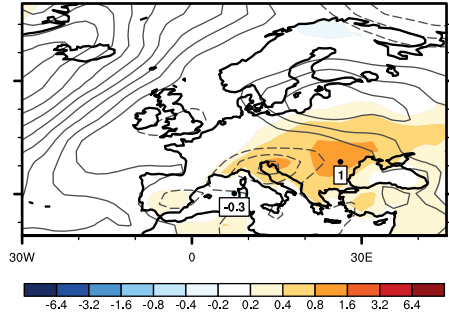
ModE-Sim
