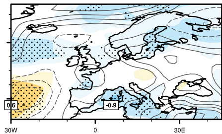
ModE-Sim
