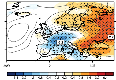
ModE-RAClim
