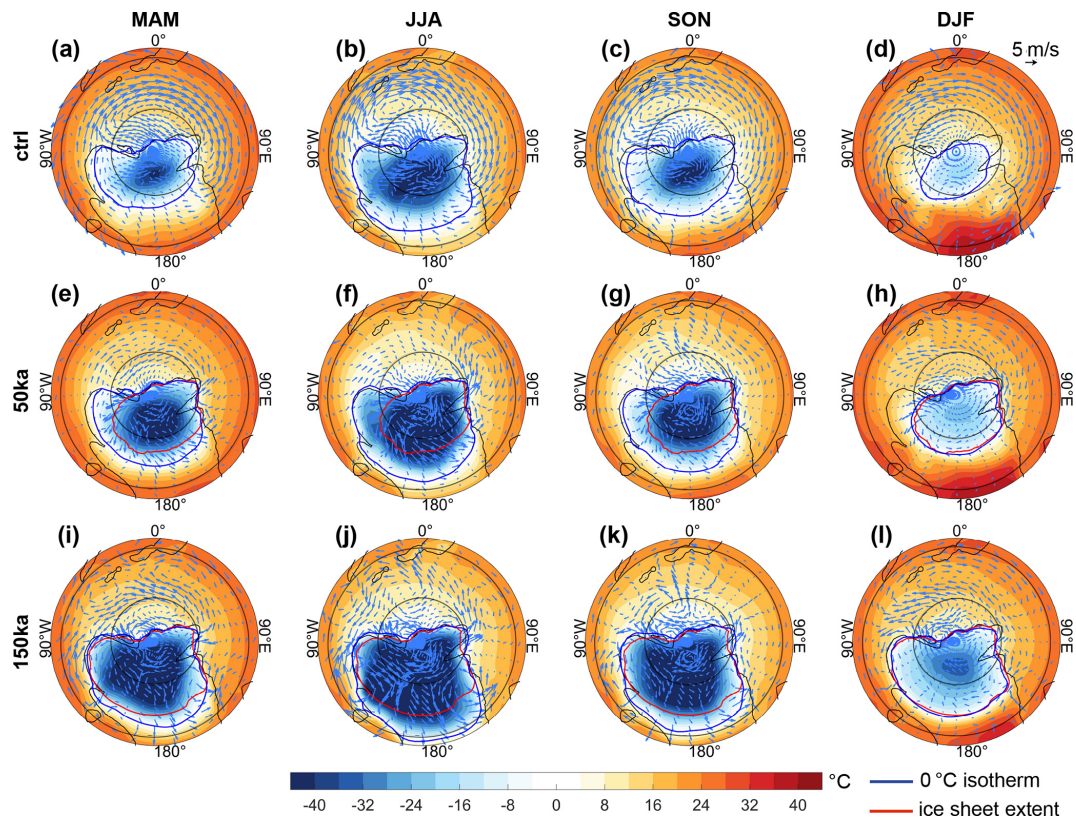
Figure 4. Surface wind field and temperature. (a–d) Surface wind field and surface temperature from the equilibrium of the CTRL for March, April, May (MAM); austral winter (June, July, and August; JJA); September, October, November (SON); and austral summer (December, January, and February; DJF). Two snapshots from the coupled framework simulation are shown in (e–h) 50 ka, (i–l) 150 ka. Note that in (e–h) and (i–l), the surface wind is shown as the difference from the CTRL. The 0 °C isotherm and ice-sheet extent are indicated by the blue and red contours, respectively. Latitude is shown at 30° intervals.
