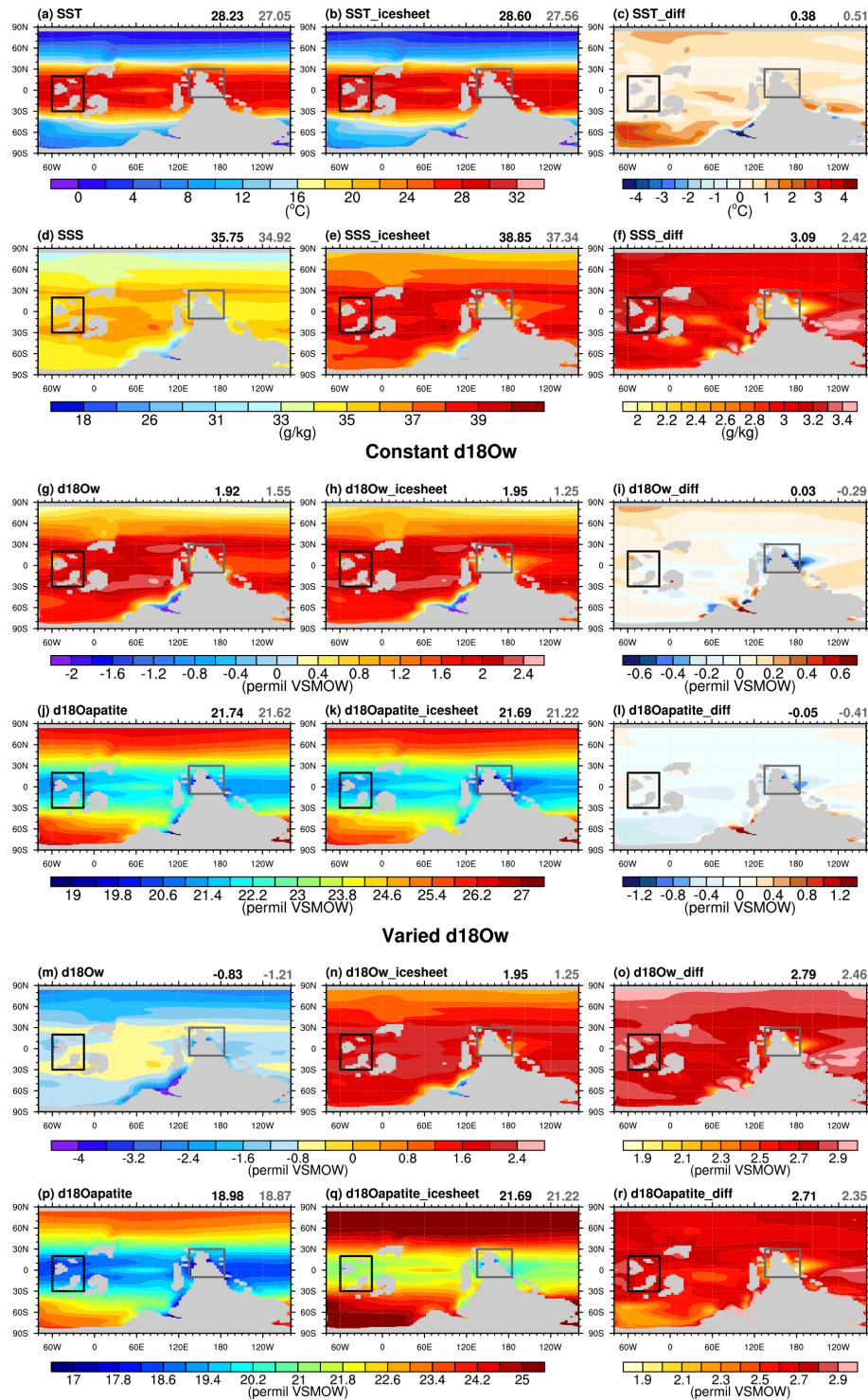
Figure B1. Simulated and calculated effects of land-ice growth on low-latitude oxygen-isotope records. Left, middle, and right columns show the case CTRL, the coupled ice-sheet experiment, and their differences, respectively. Rows 1 and 2 show simulated SST (a–c) and SSS (d–f). In the coupled ice-sheet experiment, SSS has been corrected for the global salinity increase expected from the transfer of seawater to land ice based on salt conservation. Rows 3 and 4 show the calculated surface \delta^{18}\text{O}_w (g–i) and \delta^{18}\text{O}_{\text{apelite}} (j–l), assuming a fixed background seawater oxygen-isotope composition, \delta^{18}\text{O}_0 , between the two experiments. Rows 5 and 6 show the same calculations for \delta^{18}\text{O}_w (m–o) and \delta^{18}\text{O}_{\text{apelite}} (p–r), but allowing \delta^{18}\text{O}_0 to vary with land-ice volume. The black and dark-gray boxes denote low-latitude regions corresponding to possible Ordovician oxygen-isotope records from Laurentia, including the Anticosti Island region, and Gondwana, including Australia, respectively. The black and dark-gray numbers in the upper-right corner of each panel indicate the area-weighted mean values within the black and dark-gray boxes, respectively.
