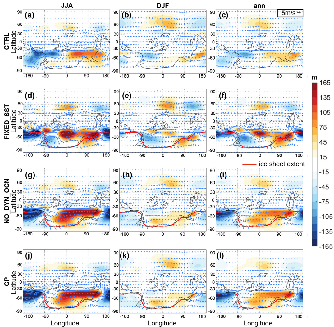
Figure 6. Structure of the stationary waves. (a–c) 500 hPa geopotential height and wind field from the CTRL, with zonal average subtracted. (d–f) as (a–c), but for the prescribed-SST experiment results. And (g–i) for the case NO_DYN_OCN, (j–l) for the coupled experiment.
