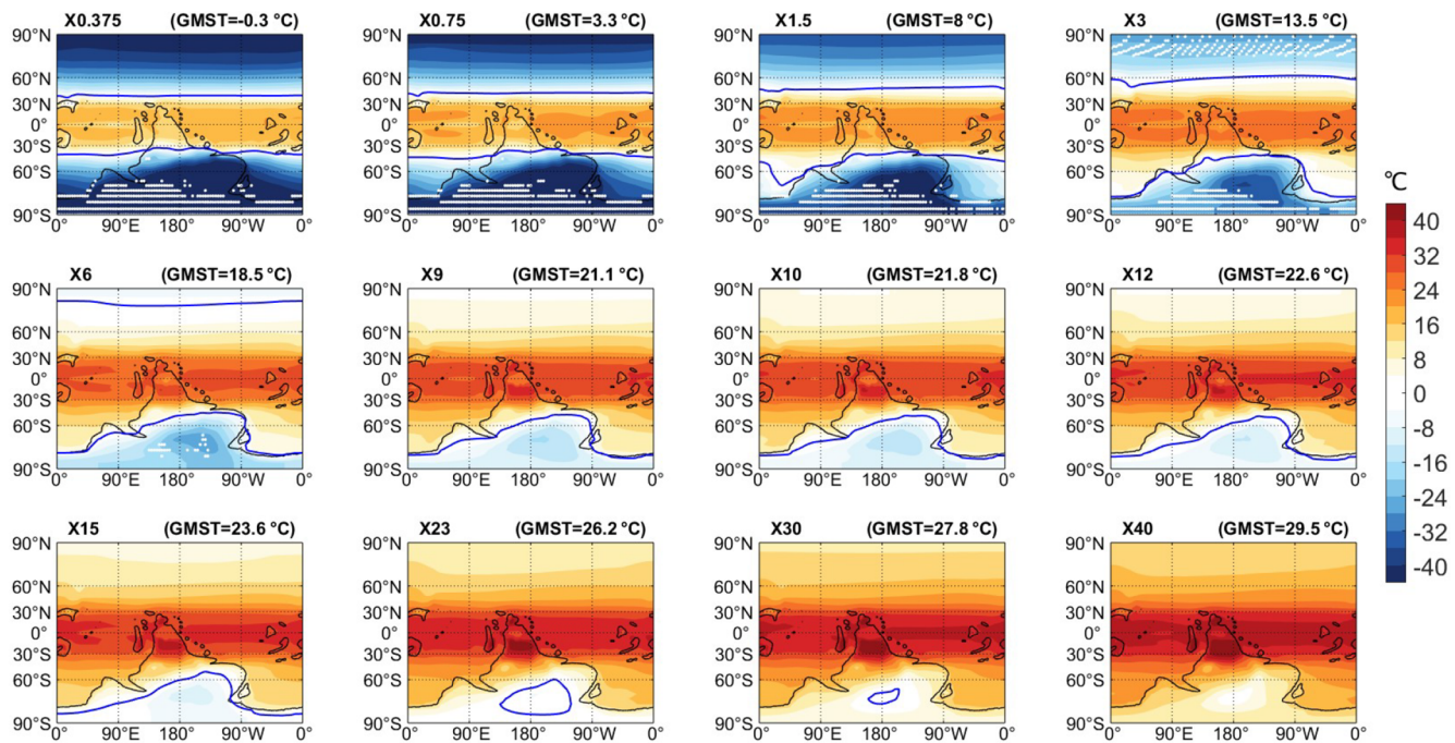
Figure C1. Late Ordovician climate sensitivity to CO 2 . Annual mean surface temperature under different PAL CO 2 conditions. White dots represent the extent of the cryosphere: sea ice is defined based on the annual mean sea ice fraction (indicating perennial ice), while land ice is defined as areas where the annual mean water-equivalent snow depth exceeds 1 m, representing potential regions for continental ice development. The results show that, in the uncoupled ice sheet scenario, a CO 2 level of 6 PAL marks the threshold for initiating continental ice formation, whereas only when greenhouse gas concentrations drop sufficiently low ( \sim 1 PAL) can land ice marginally extend to around 60° S. The development of sea ice in the SH ocean lags that of land ice. The blue solid lines represent the 0°C.
