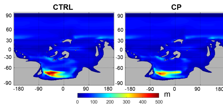
Figure C6. Comparison of mixed-layer depth between the CTRL and CP experiments. Shading indicates mixed-layer depth (m).
