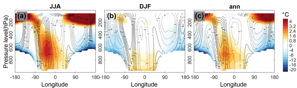
Figure 7. Difference in air temperature (color shading) and meridional wind (contours) along 65°S between the coupled and the control experiments. Solid and dashed contours indicate northerly and southerly wind anomalies, respectively. Note that the color scale is different when showing positive and negative temperature differences.
