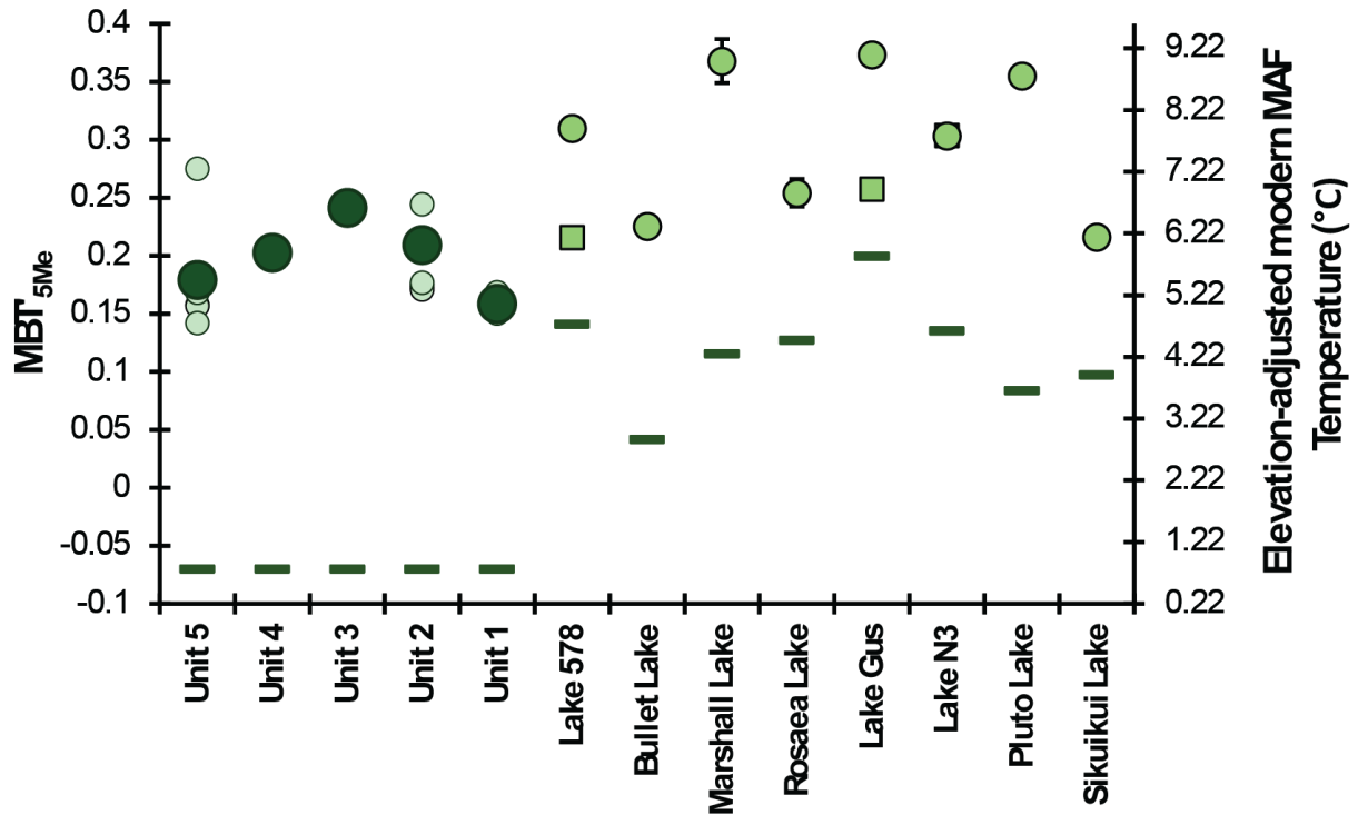
Figure S11. MBT' 5Me distributions in Camp Century units and in western Greenland Holocene Lake sediments (circles and squares; left y-axis), compared to modern months above freezing (MAF) temperature (lines; right y-axis). A: Camp Century MBT' 5Me values and temperature. Light green circles: individual samples; dark green circles: mean value for each Unit, dark green line: modern MAF temperature. Uncertainties include standard error of the mean (SEM) of each sample; all error bars are smaller than the plotted symbols. B: MBT' 5Me distributions in western Greenland Holocene Lake sediments (Acharya et al., 2026; Cluett et al., 2023; Schneider et al., 2024; Thomas et al., 2018). Circle: mean values spanning the warmest two millennia from 11.7 to 5 ka, square: mean value of the late 20th century sample from each lake dataset (not available for Bullet Lake, Marshall Lake, Rosaea Lake, Pluto Lake, and Sikuikui Lake), dark green line: modern MAF temperature at these sites. The y-axis scales are directly calculated from one another using the MBT' 5Me -temperature calibration (Otiniano et al., 2024).
