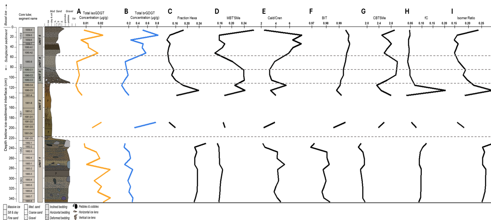
Figure S5. Downcore pattern of GDGTs and their indices in Camp Century, northwestern Greenland. (A) Concentrations of total isoprenoid (iso) GDGTs. (B) Concentrations of total branched (br) GDGTs. (C) Fractional abundance of hexamethylated brGDGTs. (D) MBT' 5Me index. (E) Ratio of caldarchaeol to crenarchaeol (Blaga et al., 2009). (F) Ratio of branched to isoprenoid tetraether (G) CBT 5Me index. (H) fC index. (I) Isomer Ratio.
