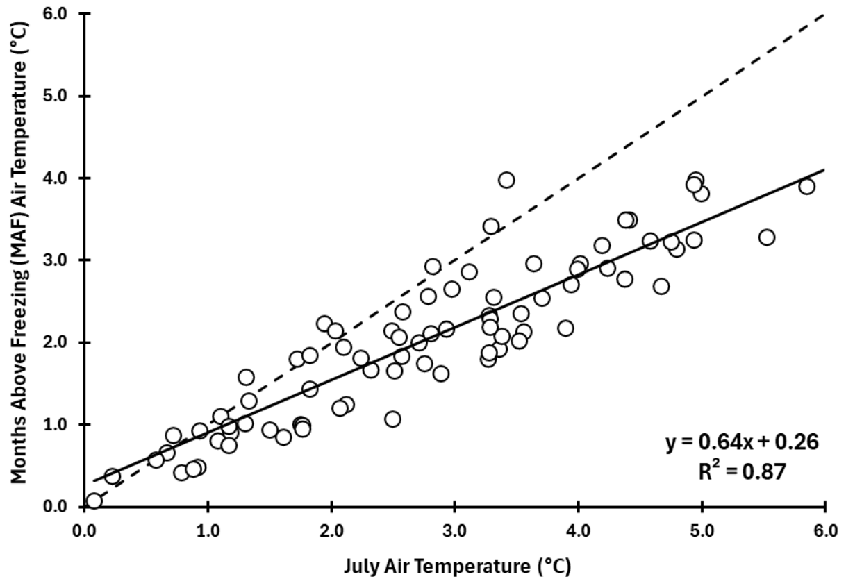
Figure S2. Linear relationship between July air temperature and months above freezing (MAF) at Pituffik Base Station based on ERA5 reanalysis data (Hersbach et al., 2020).
