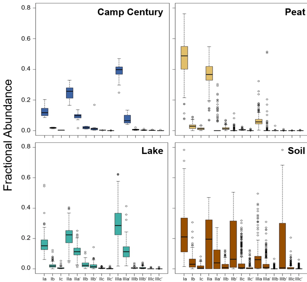
Figure S4. Fractional abundance of brGDGTs at Camp Century and modern brGDGTs in high-latitude areas. Box plots: bold lines: median, boxes: interquartile range, whiskers: 5 th and 95 th percentiles, dots: outliers. (De Jonge et al., 2015; De Jonge et al., 2021; De Jonge et al., 2019; Dearing Crampton-Flood et al., 2020; Ding et al., 2018; Dugerdil et al., 2021; Guo et al., 2020; Halffman et al., 2022; Kusch et al., 2019; Martínez-Sosa et al., 2021; Naafs et al., 2017a; Naafs et al., 2017b; Raberg et al., 2024; Raberg et al., 2021; Wang et al., 2020; Zhao et al., 2021). GDGTs are numbered as in Hopmans et al. (2016) and De Jonge et al. (2014).
