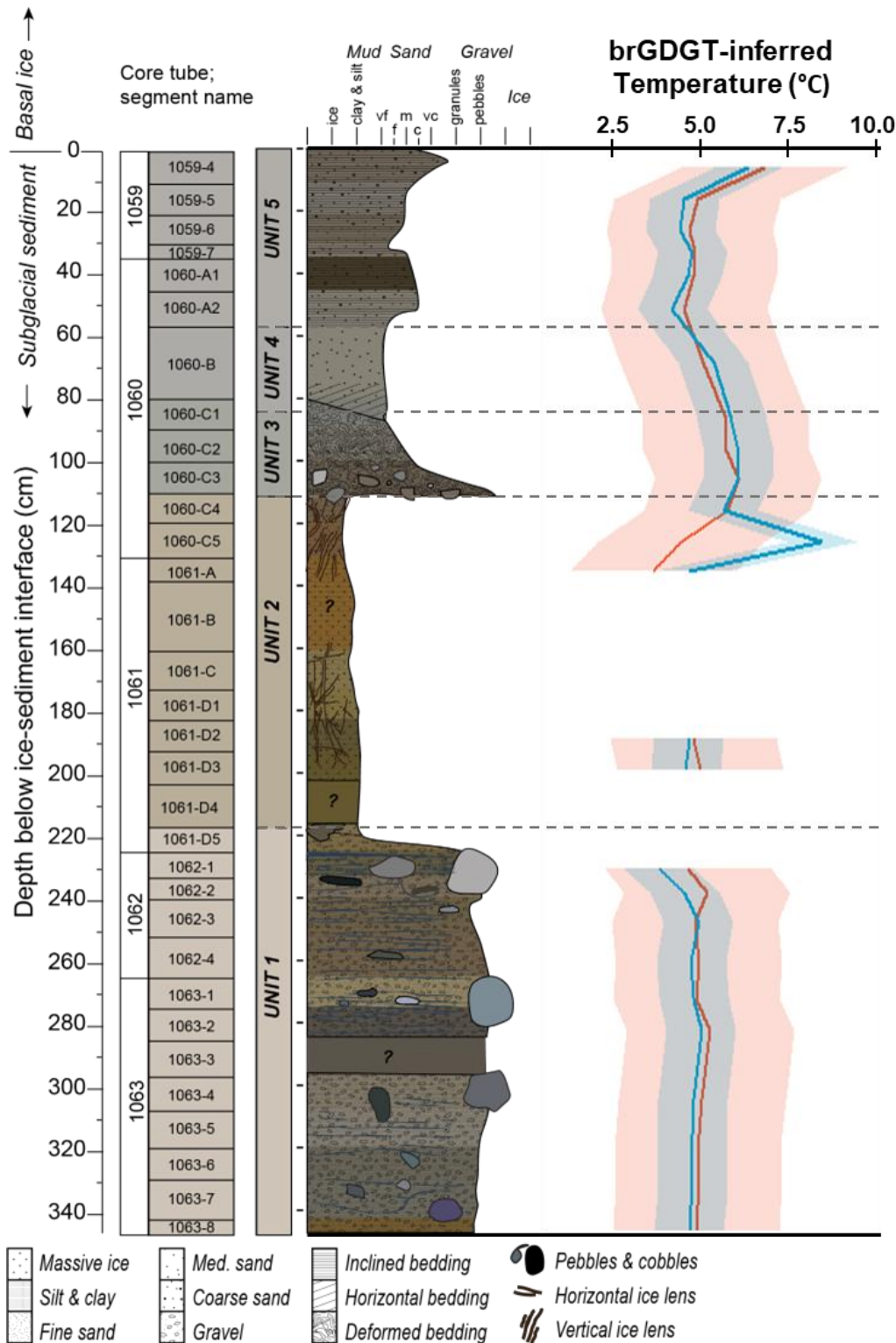
Figure S1. Reconstructed months above freezing (MAF) temperatures in Camp Century, northwestern Greenland using high-latitude lacustrine calibrations: Raberg et al. (2021) (red), and Otiniano et al. (2024) (blue). Missing points indicate samples with GDGT abundances below instrumental detection limits. Shading indicates uncertainties associated with the temperature calibration errors.
