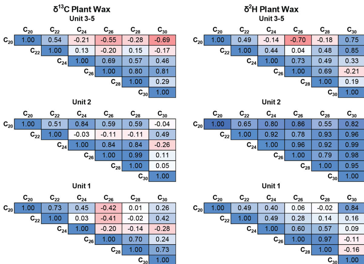
Figure S7. Correlation matrix of \delta^{13}\text{C} and \delta^2\text{H} across n -alkanoic acid chain lengths in different stratigraphic units.
