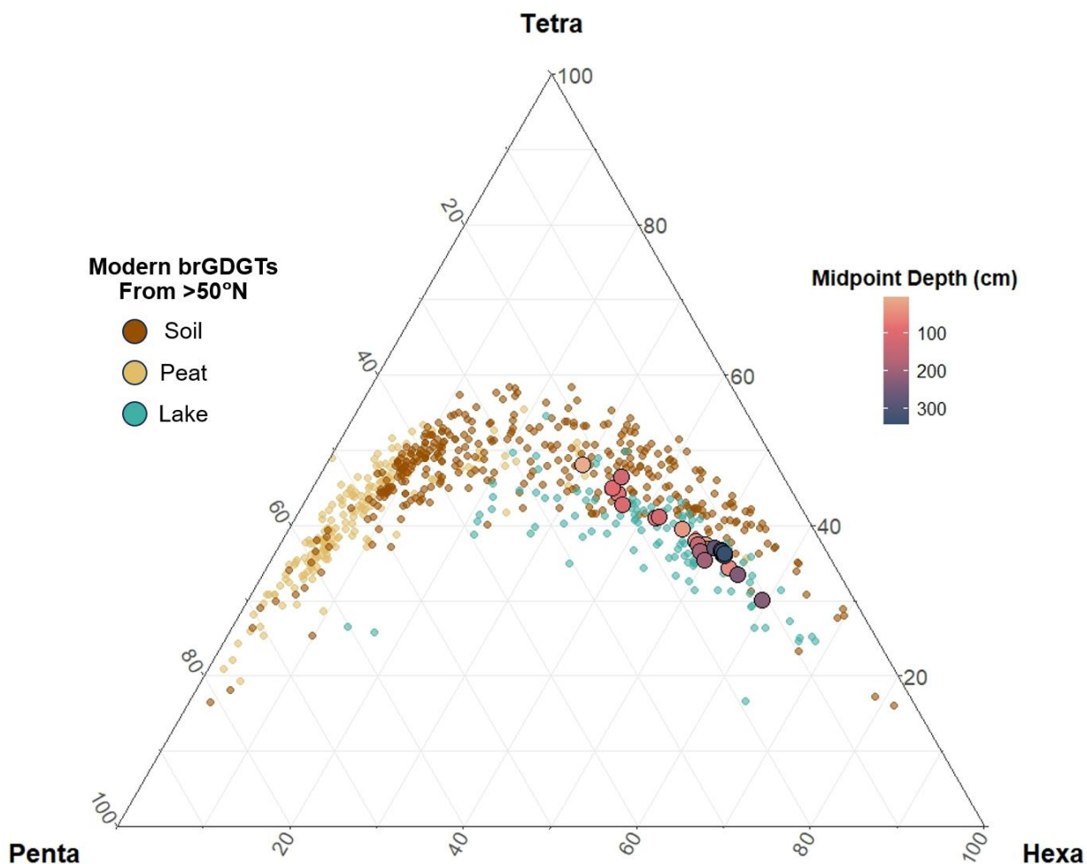
Figure S3. Ternary diagram of brGDGTs at Camp Century, large dots colored by different stratigraphic units, compared to brGDGTs from modern soil, peat and lake sources in high-latitude areas (De Jonge et al., 2015; De Jonge et al., 2021; De Jonge et al., 2019; Dearing Crampton-Flood et al., 2020; Ding et al., 2018; Dugerdil et al., 2021; Guo et al., 2020; Halffman et al., 2022; Kusch et al., 2019; Martínez-Sosa et al., 2021; Naafs et al., 2017a; Naafs et al., 2017b; Raberg et al., 2024; Raberg et al., 2021; Wang et al., 2020; Zhao et al., 2021). Tetra: tetramethylated brGDGTs, penta: pentamethylated brGDGTs, hexa: hexamethylated brGDGTs. GDGTs are numbered as in Hopmans et al. (2016) and De Jonge et al. (2014).
