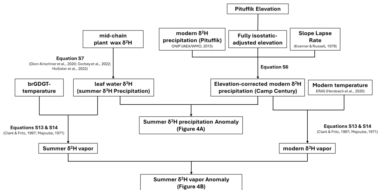
Figure S13. Schematic overview of the analytical framework used to reconstruct summer \delta^2\text{H} precipitation and summer \delta^2\text{H} vapor values and anomalies at Camp Century
