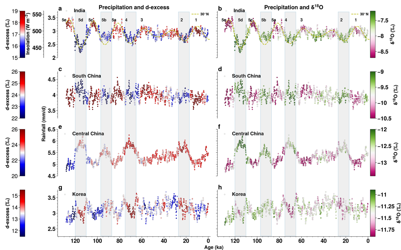
Figure 9. Simulated annual mean variations in precipitation (dots) for the last 130 ka from an orbitally forced transient simulation conducted with iCESM1.2 for India (a, b), South China (c, d), central China (e, f), and Korea (g, h) (see selected region boxes in Fig. 8). Colors of dots show precipitation- \delta^{18}\text{O} (pink to green, right panel) and d-excess (blue to red, left panel) changes. Low insolation periods are marked by gray bars. The marine isotope stage (MIS) is indicated above the top panel curves.
