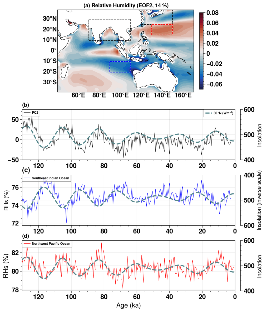
Figure 7. Second empirical orthogonal function (EOF2, a ) and corresponding principal component (PC2, b ) for the summer mean surface relative humidity for the 130 ka transient simulation on iCESM1.2. Temporal evolution of surface relative humidity over oceanic source regions, Southeast Indian Ocean: blue curve ( c ) over blue dashed box ( a ); and Northwest Pacific Ocean: red curve ( d ) over red dashed box ( a ). The black dashed boxes in panel ( a ) represent the South Asian summer monsoon and the eastern extent of the EASM region. The dashed curve represents summer insolation at 30° N.
