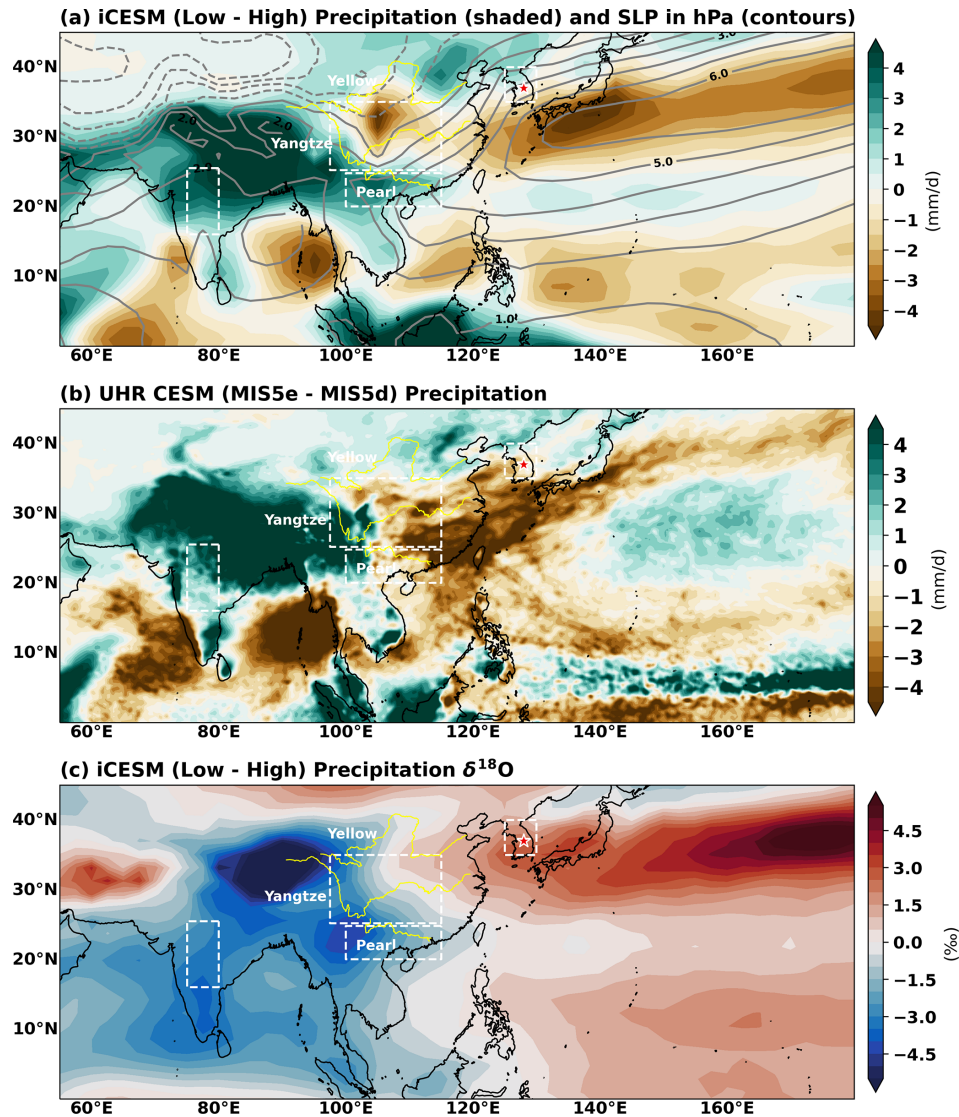
Figure 4. Difference between precession minimum (Low) and maximum (High). Composites of summer mean precipitation (shaded) and sea level pressure (SLP, contour), from iCESM1.2 (a). Same as panel (a) with CESM Ultra High Resolution (UHR) simulation for MIS5e and 5d (b), and summer mean precipitation- \delta^{18}\text{O} , from iCESM1.2 (c). The dashed boxes shown are used to extract 130 ka time series from the model simulations: India, central China, South China, and Korea (left to right in increasing longitude order). The yellow curves on the map indicate major rivers in China. The red star represents the Korean cave region.
