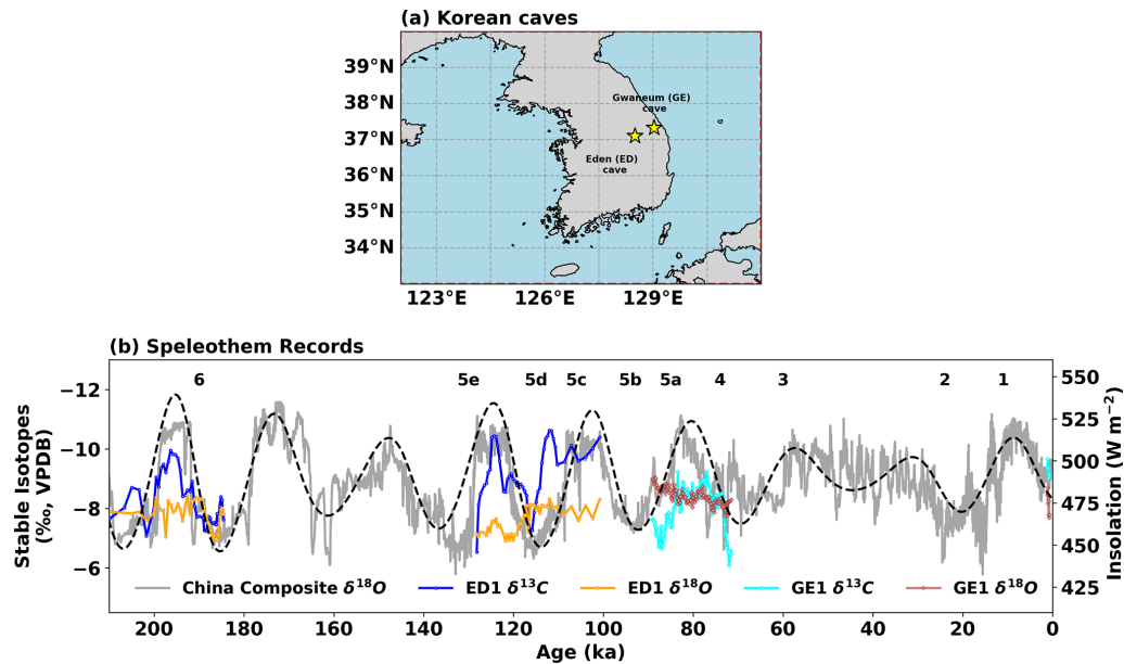
Figure 2. Korean Peninsula (red box, Fig. 1) with Korea cave locations (a). Speleothem stable isotope records ( \delta^{13}\text{C} and \delta^{18}\text{O} ) from Korean caves (Gwaneum (GE) cave and Eden (ED) cave) stalagmites (GE1 and ED1) and the Chinese caves composite- \delta^{18}\text{O} record comparison (b). The marine isotope stage (MIS) is indicated above the curves in panel (b). The black dashed curve in panel (b) represents summer insolation at 30° N.
