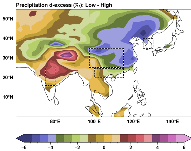
Figure 8. Precipitation d-excess for Low ( P_{\min} )–High ( P_{\max} ) precession conditions. Black dashed boxes represent regions: India, Central China, South China, and Korea (left to right), used for extracting the time series from the iCESM1.2 simulations.
