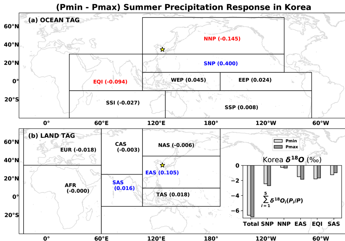
Figure 5. Differences in average summer (June–August) precipitation ( \text{mm d}^{-1} ) on the Korean Peninsula between P_{\min} and P_{\max} from various moisture sources over (a) ocean and (b) land. Colored text refers to the major contributors (mean-state) to the Korean Peninsula (blue-positive and red-negative for P_{\min}-P_{\max} ), as shown in Table S2, which was considered in the total calculations. Inset plot (lower right): the summer precipitation-weighted \delta^{18}\text{O} in Korea from major and nearby source contributors from Land (EAS, SAS) and the Ocean (SNP, NNP, EQI). Korea is marked by a yellow star. See the Supplement for the acronyms.
