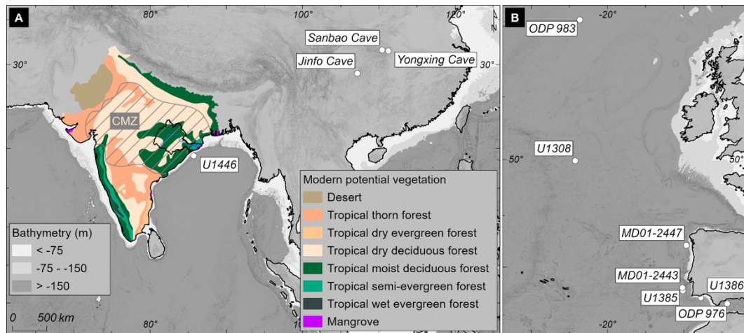
Figure 1. (A) Location of IODP Site U1446 and Chinese stalagmite records from Sanbao (Cheng et al., 2016), Jinfo (Wang et al., 2023), and Yongxing (Zhao et al., 2019) caves. Distribution of modern potential vegetation across the Indian Peninsula, with the Mahanadi catchment outlined in bold and the Core Monsoon Zone (CMZ) indicated by a striped area (adapted from Zorzi et al., 2022). (B) North Atlantic records referenced in the text: ODP 976 (Sassoon et al., 2023); U1386 (Hes et al., 2022); U1385 (Oliveira et al., 2016); MD01-2443 (Tzedakis et al., 2009); MD01-2447 (Desprat et al., 2005, 2017); U1308 (Hodell et al., 2008); ODP 983 (Barker et al., 2015, 2019).
