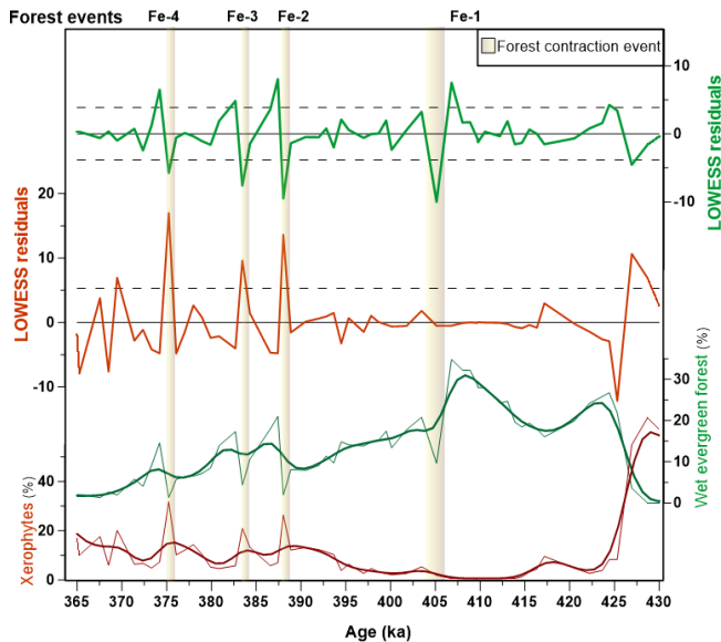
Figure 3. Pollen percentage curves of the xerophyte plants and the wet evergreen forest (bottom panel) along with the respective Gaussian smoothing filter (7 kyr-Gaussian filter, bold line) and the residuals (top panel) during MIS 11. Millennial-scale forest contraction events (brown bands) were identified when at least one sample of the model residuals exceeded the threshold of one standard deviation ( \pm 1\sigma ). Significant forest contractions occurring during the glacial inception were also concomitant with pronounced increases in xerophyte taxa percentages surpassing 1\sigma of their residual values, and were followed by significant expansions of wet evergreen tropical forest taxa.
