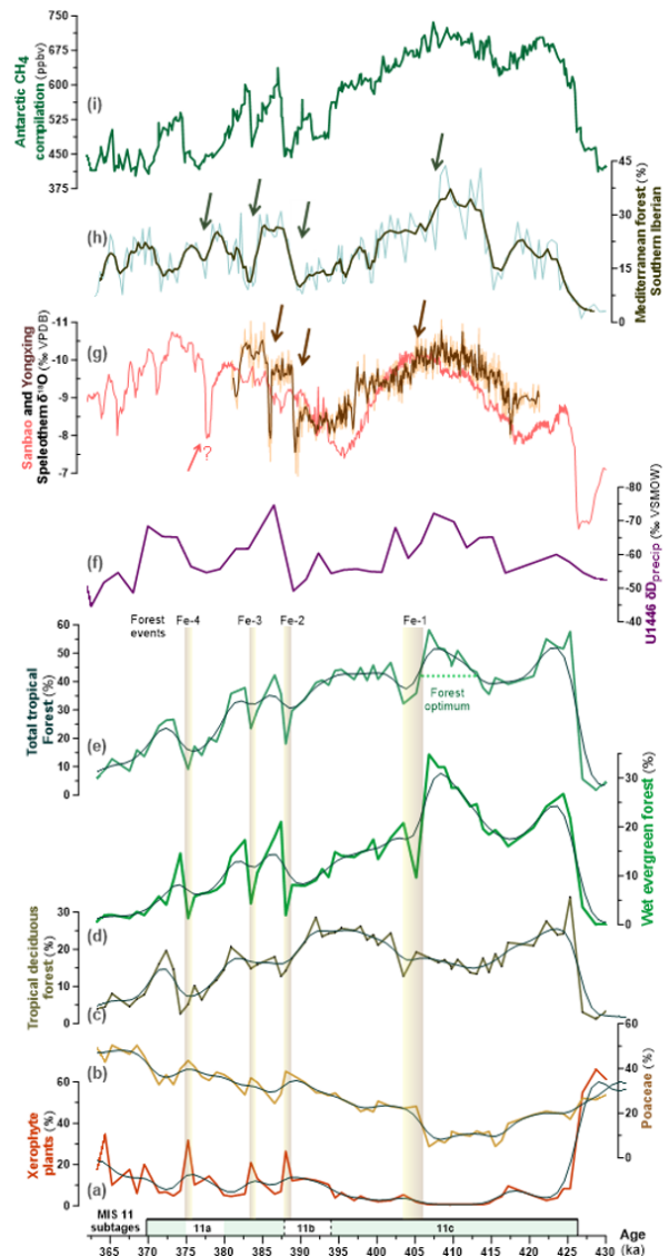
Figure 2. MIS 11 ISM-driven vegetation changes at Site U1446 – represented by the percentages of the main ecological groups/taxa with black lines representing the orbital-scale pattern extracted through a 7 kyr-Gaussian smoothing filter (a) xerophyte plants, (b) Poaceae, (c) tropical deciduous forest, (d) wet evergreen forest, and (e) total tropical forest – in the context of changes in (f) U1446 \delta D_{\text{precip}} (McGrath et al., 2021; lighter values reflect precipitation amount and moisture-source/transport changes), (g) Chinese speleothem \delta^{18}\text{O} from the Sanbao (Cheng et al., 2016) and Yongxing caves (Zhao et al., 2019), (h) Southern Iberian Mediterranean forest from Sites U1386 and U1385 (bold line – 3 point moving average, chronology derived from LR04) (Oliveira et al., 2016; Hes et al., 2022) and (i) \text{CH}_4 concentrations from the Antarctica EPICA Dome C ice core, AICC2012 chronology (Nehrbass-Ahles et al., 2020). MIS 11 substages are indicated at the bottom, with pollen zones distinguishing three forest expansion phases marked by green bands during MIS 11c and 11a, interspersed with phases of more open vegetation during MIS 11b and mid-MIS 11a. Forest events (Fe-1 to -4) are depicted by brown bands indicating forest contractions/ISM weakening. Arrows in (g) and (h) denote potential concurrent millennial-scale events.
