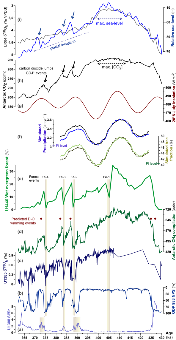
Figure 4. MIS 11 drivers of ISM-driven vegetation variability on orbital and millennial timescales. North Atlantic changes: (a) meltwater discharges inferred from Si/Sr of Site U1308 (Hodell et al., 2008), (b) ODP Site 983 polar planktic foraminifera (Barker et al., 2015, 2019), and (c) \delta^{13}\text{C} from Site U1385 indicative of AMOC changes (Nehrbass-Ahles et al., 2020). (d) \text{CH}_4 record (Nehrbass-Ahles et al., 2020) with red dots denoting predicted Dansgaard-Oeschger (D-O) warming events (Barker et al., 2011). U1446 data: (e) Percentage of the wet evergreen forest with forest contraction events (Fe-1 to -4) (this study) and (f) LOVECLIM1.3 simulations averaged over the Indian CMZ ( 17\text{--}27.5^\circ\text{N} , 67.5\text{--}90^\circ\text{E} ) for the tree fraction and annual precipitation (this study) with time-varying insolation and \text{CO}_2 , and with fixed \text{CO}_2 at 280 ppmv (black line). Primary forcings: (g) 21 July insolation at 20^\circ\text{N} (Berger and Loutre, 1991), with the pre-industrial level indicated, (h) \text{CO}_2 concentrations from the EDC Antarctic ice core, with arrows marking abrupt \text{CDJ}^+ (carbon dioxide jumps) coinciding with significant \text{CH}_4 increases (Nehrbass-Ahles et al., 2020) and (i) Relative sea-level from the Red Sea (Grant et al., 2014) and \delta^{18}\text{O}_{\text{benthic}} from the LR04 (Lisiecki and Raymo, 2005).
