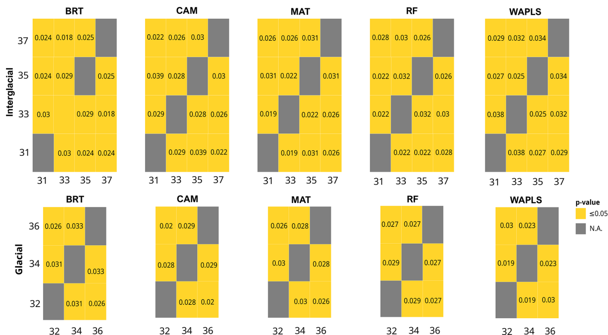
Figure 6. PERMANOVA p -values between the same types of periods (glacial-glacial and interglacial-interglacial) for each climate reconstruction method on centred-reduced data. A p -value less than or equal to 0.05 is significant and indicates that the two periods are different from each other.
