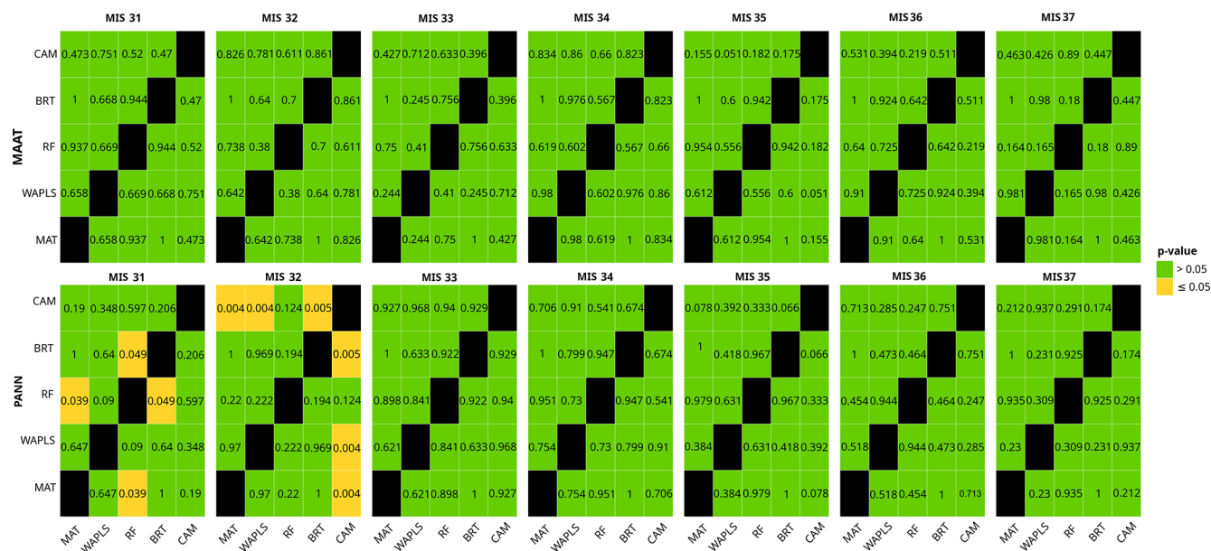
Figure 5. PERMANOVA p -values between climate reconstruction methods for each isotopic stage and for Mean Annual Air Temperature (MAAT) and Mean of Annual Precipitation (PANN). A p -value less than or equal to 0.05 is significant and indicates that the two methods are different from each other.
