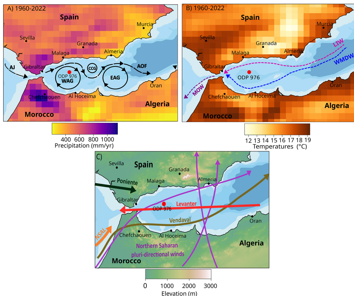
Figure 1. ODP site 976 climate and location maps. Climate data from ERA5 reanalysis between 1960–2022 with a lat-lon grid of 0.25^\circ . (A) Mean annual precipitation with sea surface circulation. AJ: Atlantic Jet, WAG: Western Alboran Gyre, CCG: Central Cyclonic Gyre and EAG: Eastern Alboran Gyre. (B) Mean annual temperature with sea deep circulation. MOW: Mediterranean Outflow Water, LIW: Levantine Intermediate Water and WMDW: Western Mediterranean Deep Water. (C) Atmospheric circulation. NSAL: Northern Saharan Air Layer.
