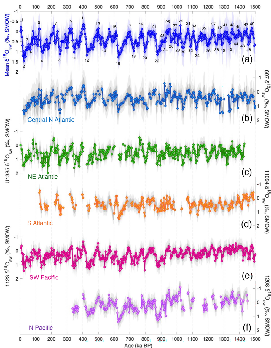
Figure 4. Interpolated and bootstrapped \delta^{18}\text{O}_{\text{seawater}} records for all sites. (a) Non-weighted mean \delta^{18}\text{O}_{\text{seawater}} stack (this study; blue line and markers) with MIS numbers denoting glacial stages (below) and interglacial stages (above). Interpolated and bootstrapped \delta^{18}\text{O}_{\text{seawater}} records for: (b) DSDP Site 607 (Ford et al., 2016; Sosdian and Rosenthal, 2009) (blue); (c) IODP Site U1385 (this study, including additional Iberian Margin records (Birner et al., 2016; Skinner et al., 2003; Skinner and Elderfield, 2007) (green); (d) ODP Site 1094 (Hasenfratz et al., 2019) (orange); (e) ODP Site 1123 (Elderfield et al., 2012) (pink); and (f) ODP Site 1208 (Ford and Raymo, 2020) (purple). All \delta^{18}\text{O}_{\text{seawater}} records were interpolated to a 3 kyr interval and subsequently bootstrapped. Shading denotes 1\sigma and 2\sigma error margins (dark and light grey respectively), propagated from both analytical and calibration uncertainties.
