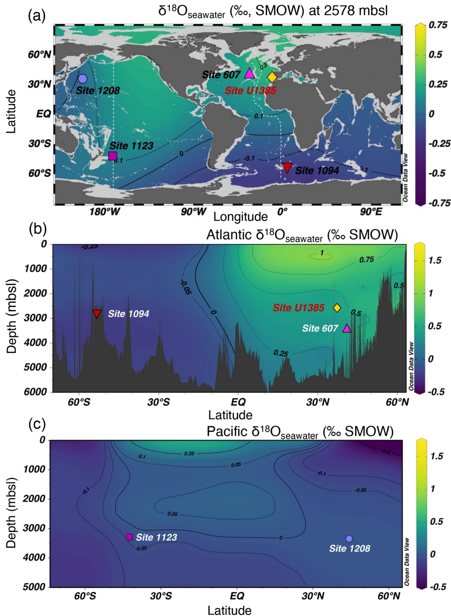
Figure 1. Meridional profiles of deep-water \delta^{18}\text{O}_{\text{seawater}} showing the site locations. (a) \delta^{18}\text{O}_{\text{seawater}} at 2578 m b.s.l., corresponding to the depth of IODP Site U1385 (this study; yellow diamond) in the Northeast Atlantic, along with the geographic location of other sites referenced in the text: North Atlantic DSDP Site 607 (Ford et al., 2016; Sosdian and Rosenthal, 2009) (pink triangle); Southwestern Pacific ODP Site 1123 (Elderfield et al., 2012) (purple square); North Pacific ODP Site 1208 (Ford and Raymo, 2020) (lilac circle); and the Southern Ocean ODP Site 1094 (Hasenfratz et al., 2019) (red inverted triangle) located in the Atlantic sector of the Antarctic Zone. Meridional transects shown in panels (b) and (c) are indicated by white dashed lines. (b, c) Atlantic and Pacific meridional profiles of deep-water \delta^{18}\text{O}_{\text{seawater}} (‰, SMOW) showing site locations. Maps were created using GLODAPv2.2021 and GLODAPv2.2023 and GEOSECS in Ocean Data View (Schlitzer, 2019; http://odv.awi.de/ , last access: 7 July 2026). Data for panel (c) are from (LeGrande and Schmidt, 2006).
