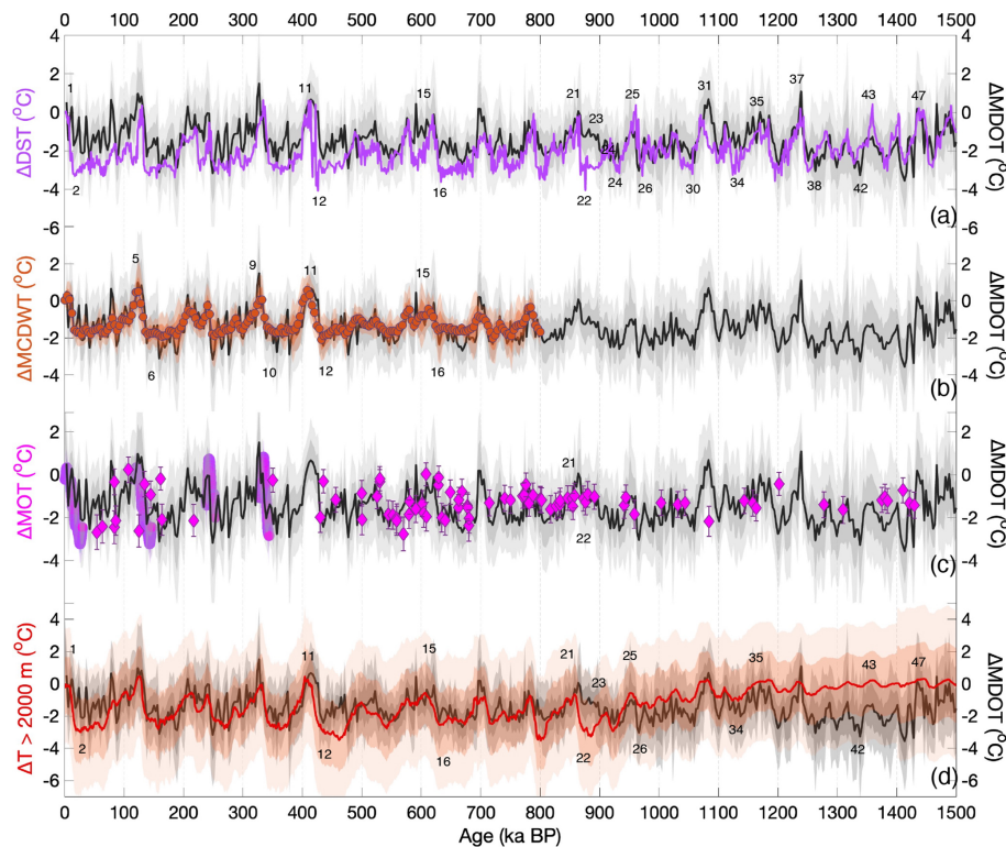
Figure 10. Comparison of MDOT with similar mean ocean and deep-water temperature reconstructions. All panels show the change in volume-weighted MDOT ( \Delta\text{MDOT} ) (this study; black line) relative to an average present day value ( 1.73^\circ\text{C} ) versus: (a) the change in deep-sea temperature ( \Delta\text{DST} ) estimated relative to the present (Rohling et al., 2021) (purple line); (b) the change in mean CDW temperature ( \Delta\text{MCDWT} ) relative to present (Chandler and Langebroek, 2024) (dark orange circles); (c) the change in MOT ( \Delta\text{MOT} ) derived from noble gas measurements in ice cores (Grimmer et al., 2025) (purple and pink circles) and, in Allan Hills blue ice (pink diamonds) (Shackleton et al., 2026), error bars on individual MOT estimates represent absolute uncertainties; and, (d) \Delta\text{MOT} inferred from \Delta\text{GMSST} and proxy-based deep-water temperature (Clark et al., 2025a) (red), with both records referenced to the Early Holocene ( 0^\circ\text{C} at 10 ka) and offset by -1.73^\circ\text{C} following (Clark et al., 2025a). Dark and light shading of the same colour represent 1\sigma and 2\sigma uncertainty envelopes, respectively. Uncertainties associated with \Delta\text{MOT} are taken directly from the published datasets of Clark et al. (2025a). MIS numbers mark many of the glacial (even) and interglacial (odd) stages.
