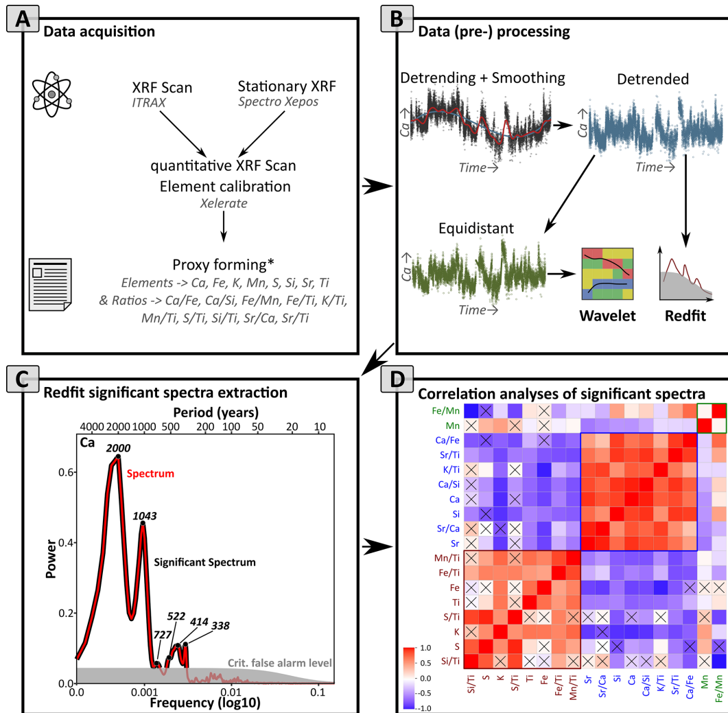
Figure 2. Flowchart of the high resolution XRF methodological approach. (A) Acquisition of high resolution XRF data, calibration and forming elements and elemental ratios. *Proxy choice was done by common and published palaeolimnological XRF proxies (Cohen, 2003; Davies et al., 2015). (B) Processing of high-resolution data for time series (Redfit and Wavelet) analyses, by detrending and equidistant resampling (precondition for Wavelet analyses). (C) Extraction of significant (line above the critical Level of the AR1 red noise) Redfit power spectra of each proxy. (D) Correlation analysis of the significant Redfit power spectra using the Spearman coefficient. The crosses show the non-significant (0.05 level) correlation values.
