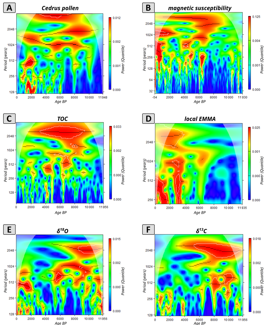
Figure 8. Wavelet power spectra of (a) Cedrus pollen proportion (Campbell et al., 2017), (b) Magnetic susceptibility scan and (c) TOC (Zielhofer et al., 2017a), (d) Grain Size Endmember Analysis (EMMA) ratio (local provenance) (Zielhofer et al., 2017b), (e) \delta^{18}\text{O} values and (f) \delta^{13}\text{C} values of ostracod shells (Zielhofer et al., 2019b). Colours show the specific power values. White lines enclose the significant areas. Grey facet shows the cone of influence.
