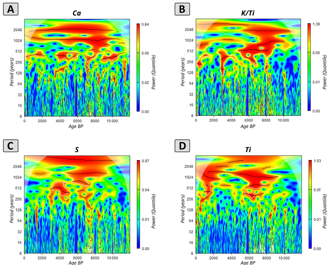
Figure 6. Exemplary wavelet power spectra of (a) Ca, (b) K/Ti, (c) S and (d) Ti. Colours show the specific power values. White lines enclose the significant areas and black lines local maxima. Grey facet shows the cone of influence.
