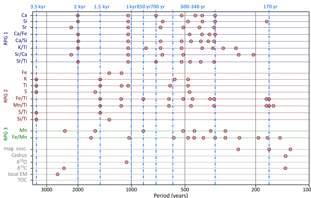
Figure 4. Synoptic graph of the positive peaks of the significant Redfit spectra of each XRF and non-XRF proxy. The x-axis is \log_{10} scaled, reflects the period and the red dots show the position of the peaks. The configuration and grouping of the XRF proxies follow the results from the correlation analysis (Redfit Proxy Groups). The blue dotted lines (with labels on top of the graph) show dominant modes of periodicity of the presented proxies.
