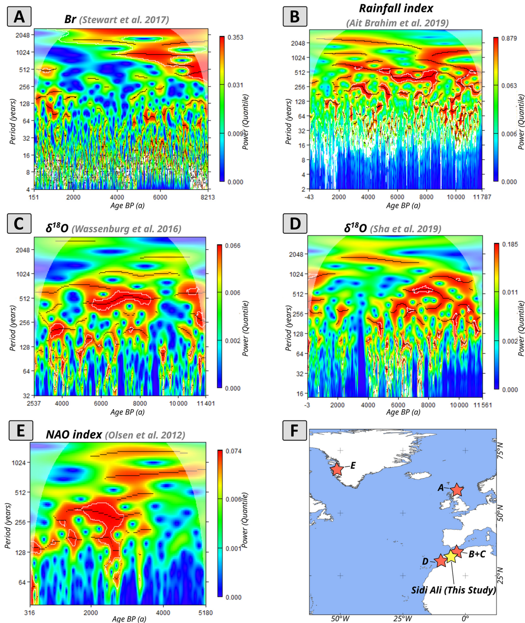
Figure 9. Wavelet power spectra of (A) Br record (Stewart et al., 2017), (B) Rainfall index (Ait Brahimi et al., 2019), (C) \delta^{18}\text{O} record from Grotte de Piste cave (Wassenburg et al., 2016) and (D) \delta^{18}\text{O} record from Chaara cave (Sha et al., 2019), (E) NAO index (Olsen et al., 2012). Colours show the specific power values. White lines enclose the significant areas. Grey facet shows the cone of influence. Panel F shows a map of the geographic locations of the datasets presented in this figure (EPSG: 4326).
