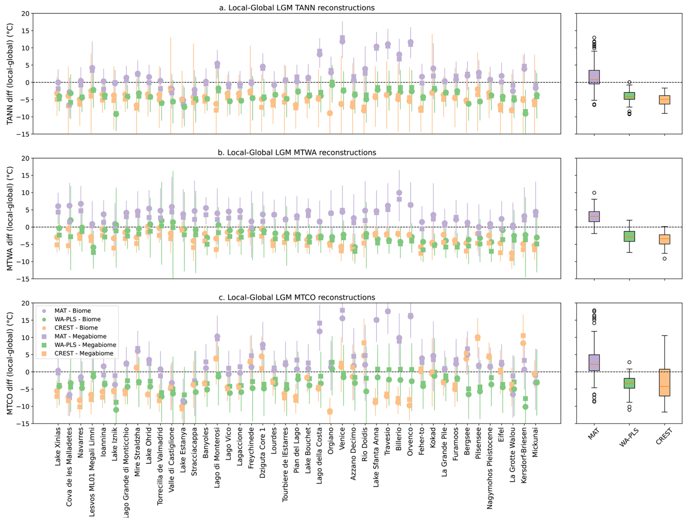
Figure 9. Mean LGM annual temperature (a), MTWA (b) and MTCO (c) anomalies for each fossil site, calculated as the difference between (mega)biomized and not-(mega)biomized (global calibration) climate variables for the three methods of pollen-based climate reconstruction. The biomization and megabiomization results are shown using circle and square symbols, respectively. Site names are arranged (left to right) in ascending order of latitude. Results are reported in Supplement 6. Errors are 1\sigma . The boxplots on the right represent the distributions of the mean local–global differences for each climate variable across reconstruction methods (in color).
