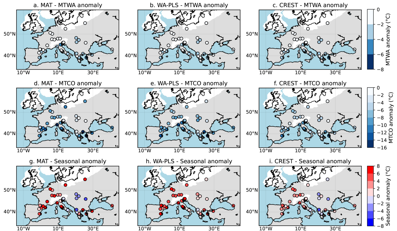
Figure 6. Monthly (MTWA and MTCO, in a–c and d–f , respectively) temperature anomaly (LGM–Modern climate) results, using the biomization process for the three different pollen-based climate reconstruction methods. From MTWA and MTCO results, seasonal anomalies are reported on panels ( g )–( i ) in Fig. 6 and 7. Modern climates and LGM climate results are reported in Supplement 6. The white area represents the ice sheet extent (Peltier and Solheim, 2004; Ehlers et al., 2011; Seguinot et al., 2018). Geographic coordinates are displayed in WGS84.
