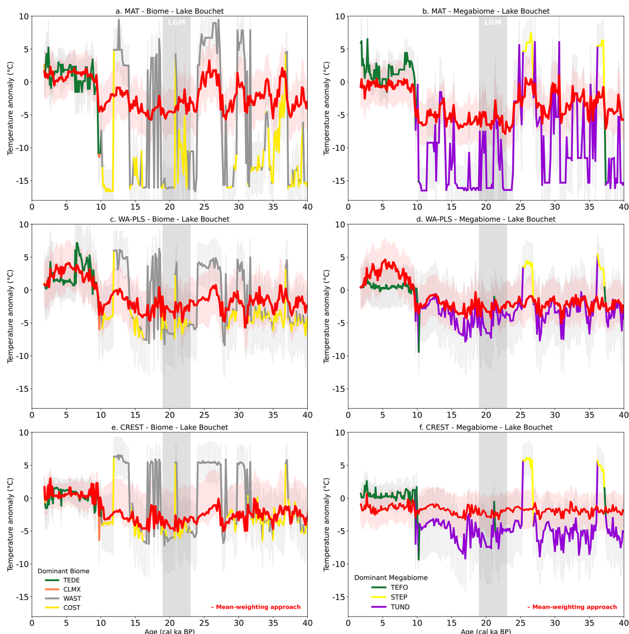
Figure 4. TANN anomaly (LGM–Modern climate, LGM cooling) reconstructed over time at Lake Bouchet using three different reconstruction methods for (mega)biomization procedures. Bold curves show TANN reconstructed and their climatic errors ( 1\sigma ) from the dominant (mega)biome (colored according to the dominant biome). Bold red curves report the weighted mean TANN reconstructed from (mega)biome scores. Confidence in mean-weighting is indicated by red areas. The grey area indicates the LGM time interval. The modern climate reference is TANN = 8.3 °C. All climate data were processed using the current biomization assignment scheme in CREST (Fig. 2).
