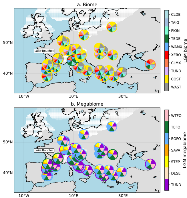
Figure 3. Percentage of fossil biomes (a) and megabiomes (b) in pollen sequences during the LGM across Europe. Colored outlines around the pie charts indicate the dominant (mega)biomes. The position of the Lake Bouchet samples is outlined with a thin black circle and labeled in the figure. The white area represents the ice sheet extent (Peltier and Solheim, 2004; Ehlers et al., 2011; Seguinot et al., 2018). Geographic coordinates are displayed in WGS84.
