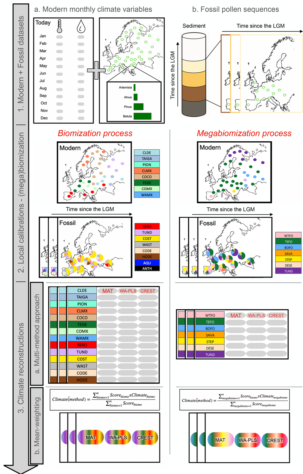
Figure 1. Schematic representation of the methodological approach developed in Sect. 3 of this study. Gray vertical boxes (on the left of this figure) illustrate methodological steps performed in this study. Reconstruction methods are developed in Sect. 4.
