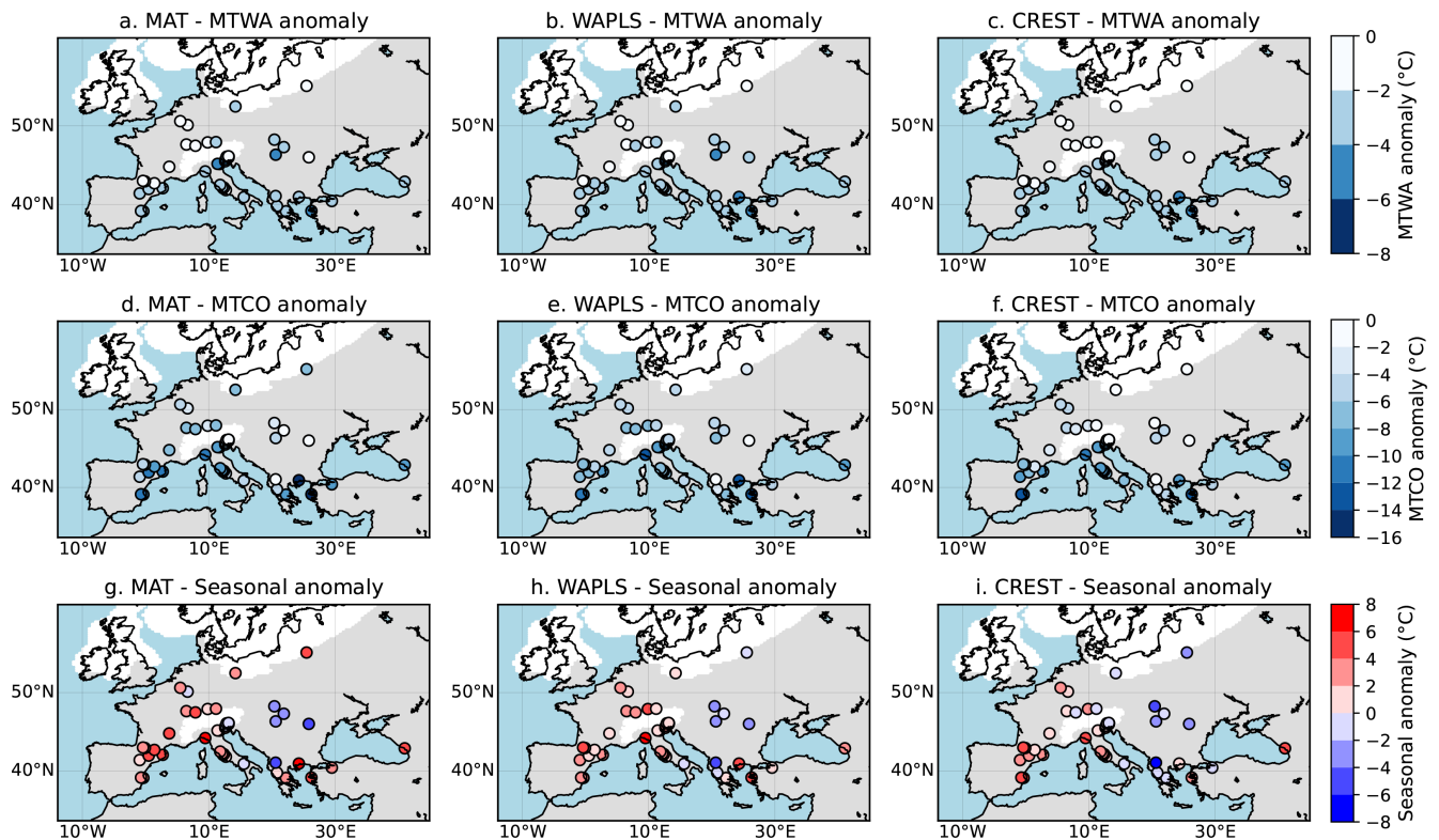
Figure 7. Monthly (MTWA and MTCO, in a–c and d–f , respectively) temperature anomaly (LGM–Modern climate) results, using the megabiome process for the three different pollen-based climate reconstruction methods. From MTWA and MTCO results, seasonal anomalies are reported on Fig. ( g )–( i ). Modern climates and LGM climate results are reported in Supplement 6. The white area represents the ice sheet extent (Peltier and Solheim, 2004; Ehlers et al., 2011; Seguinot et al., 2018). Geographic coordinates are displayed in WGS84.
