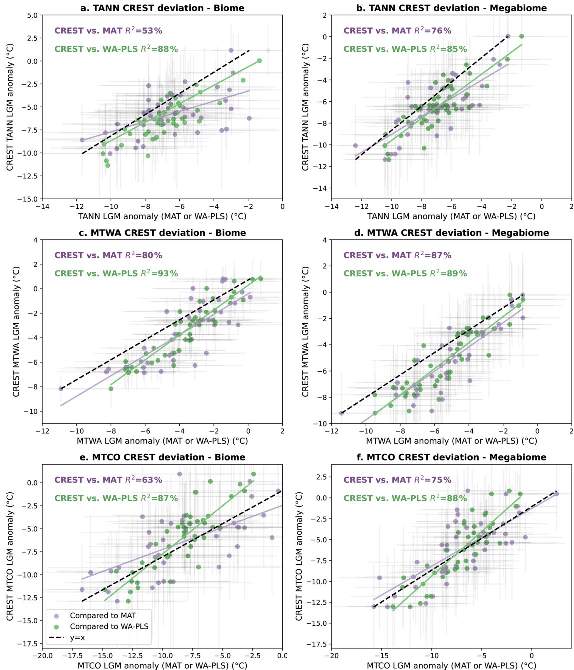
Figure 11. Linear relationship between TANN (a, b), MTWA (c, d) and MTCO (e, f) anomaly results (LGM–Modern climate) from the three pollen-based climate reconstruction methods, using biomization and megabiomization procedures. All R^2 values reported in this study are statistically significant, with p values < 0.01 . These plots show relationships between CREST results and those from statistical methods (MAT in blue and WA-PLS in green) from the 43 fossil sites. Errors are 1\sigma .
