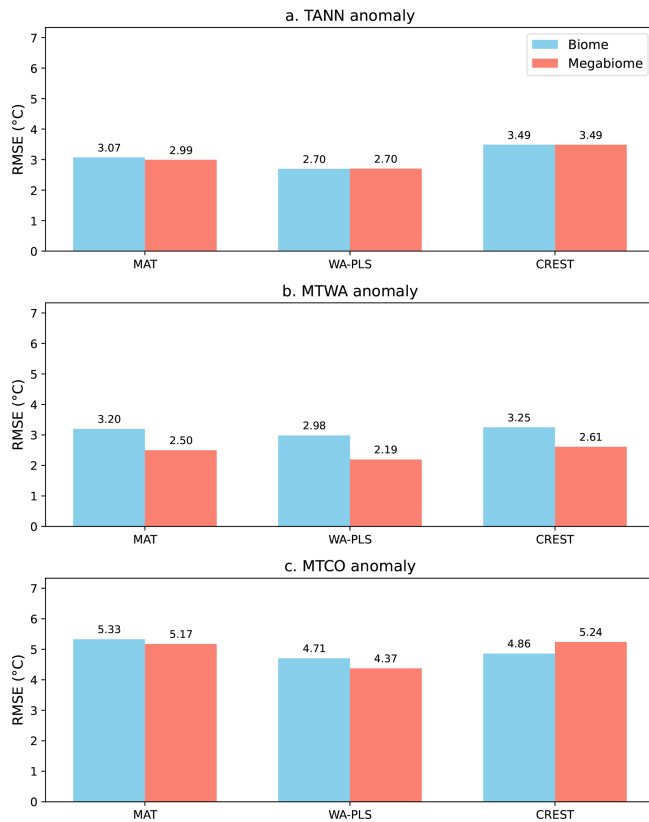
Figure 12. RMSE of mean annual (a) and monthly anomalies (b, c) (LGM–Modern climate) between our three reconstruction methods (MAT, WA-PLS, CREST) and results from Davis et al. (2024). Bars represent RMSE for Biome (blue) and Megabiome (orange), with RMSE values reported above each bar to indicate the reconstruction error relative to Davis et al. (2024).
