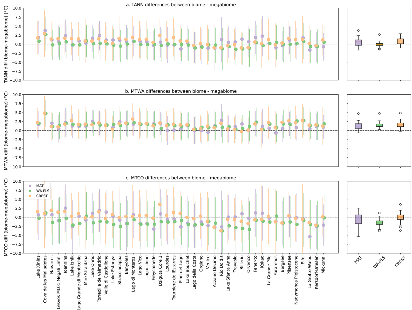
Figure 10. Mean LGM annual temperature (a), MTWA (b) and MTCO (c) anomalies for each fossil site, calculated as the difference between biomized and megabiomized climate variables for the three methods of pollen-based climate reconstruction. Site names are arranged in ascending order of latitude. Results are reported in Supplement 6. Errors are 1\sigma . The boxplots on the right represent the distributions of the mean biome–megabiome differences for each climate variable across reconstruction methods (in color).
