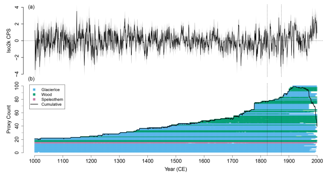
Figure 2. (a) NAO reconstruction ensemble members (grey shading) and ensemble median (black line). Horizontal dashed line shows zero. Vertical dashed lines indicate calibration and validation cutoff years at 1823 and 1873 CE. (b) Record coverage through time for the full Northern Hemisphere Iso2k dataset including glacier ice (blue), wood cellulose (green), and speleothem (red) records. Solid black line indicates the total number of available records in each year.
