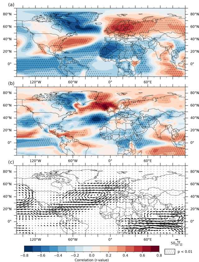
Figure 5. Winter \text{NAO}_{\text{iLME}} correlations (color contours) with iLME winter surface air temperature, precipitation amount, and composite IVT from 1823–2000 CE. Stippling denotes p < 0.01 . (a) \text{NAO}_{\text{iLME}} correlation with winter surface air temperature. (b) \text{NAO}_{\text{iLME}} correlation with winter precipitation amount. (c) Difference between winter IVT during positive and negative winter \text{NAO}_{\text{iLME}} years, defined as \text{NAO}_{\text{iLME}} greater or less than one standard deviation from the mean, respectively, over the period 1823–2000 CE.
