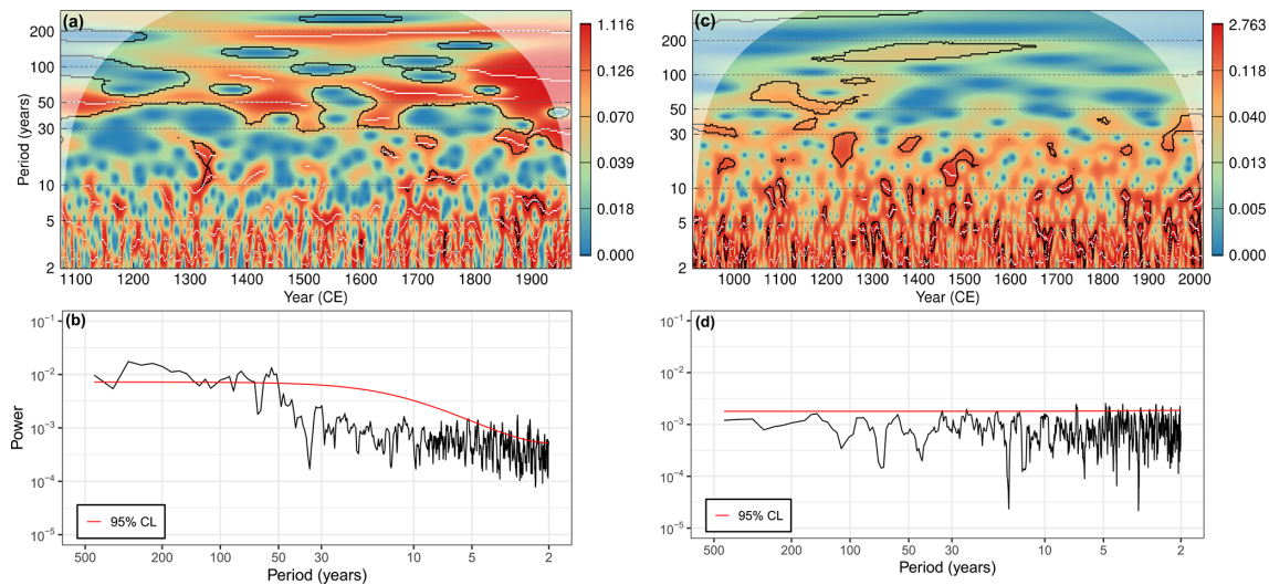
Figure 8. As in Fig. 6 but for the NAO reconstruction ensemble means from Ortega et al. (2015) (a, b) and Cook et al. (2019) (c, d).
