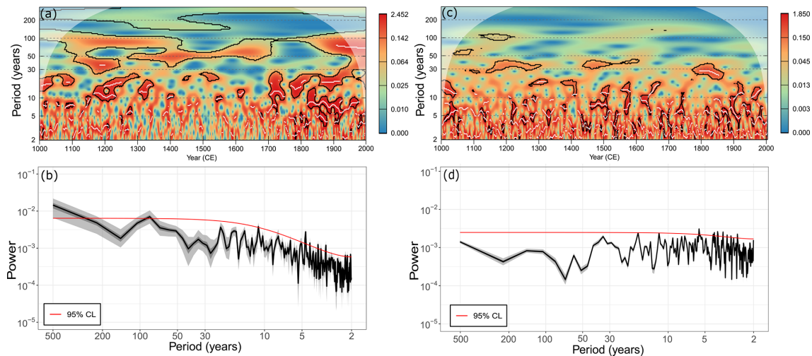
Figure 6. (a) Wavelet decomposition of the NAO reconstruction from 1000–2000 CE. Color contours are scaled by power quantiles. Black contours bound statistically significant power ( p < 0.05 ) and white curves show ridges (power maxima). White envelope shows the region where padding may influence estimates. (b) The multi-taper method spectral decomposition for the NAO reconstruction. Red line shows 95 % confidence level based on an AR(1) null. Grey shading shows ensemble range. (c) and (d) are as in (a) and (b) but for the NAO pseudo-reconstruction from the iLME \delta^{18}\text{O}_{\text{precip}} field.
