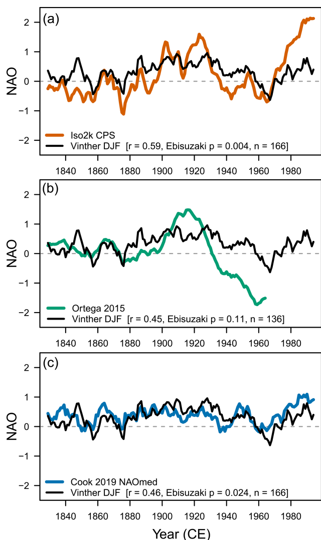
Figure 7. Decadally smoothed NAO reconstructions during the observational period compared with the decadal smoothed \text{NAO}_{\text{Vinther}} index (black lines). Series are smoothed using an 11-year centered running mean. (a) Iso2k CPS reconstruction (this study; orange) vs. \text{NAO}_{\text{Vinther}} . (b) Ortega et al. (2015) calibration constrained median (teal) vs. \text{NAO}_{\text{Vinther}} . (c) Cook et al. (2019) \text{NAO}_{\text{med}} (blue) vs. \text{NAO}_{\text{Vinther}} .
