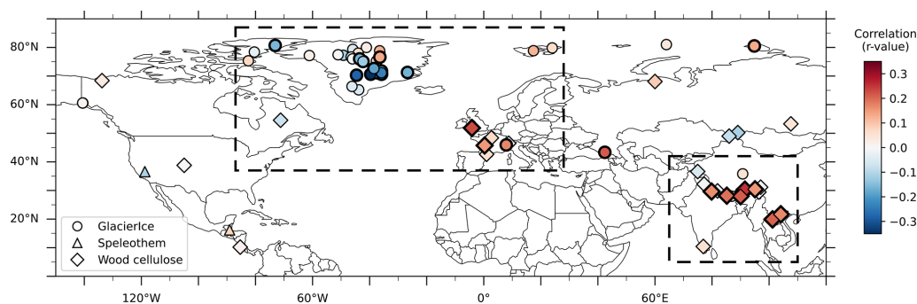
Figure 1. Map of Iso2k records included in the analysis. Shapes correspond to archive type and colors denote the Pearson's r -value of each record with \text{NAO}_{\text{Vinther}} (1823–2000 CE). Bold outlines signify significant correlation ( p < 0.1 ). Regional subsets used for validation are indicated by dashed boxes over Greenland and southeast Asia.
