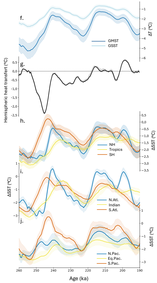
All annual records (n=106)
