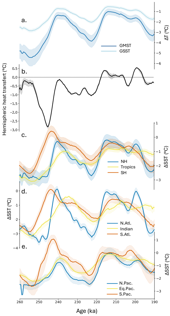
Selected records (n=91)
