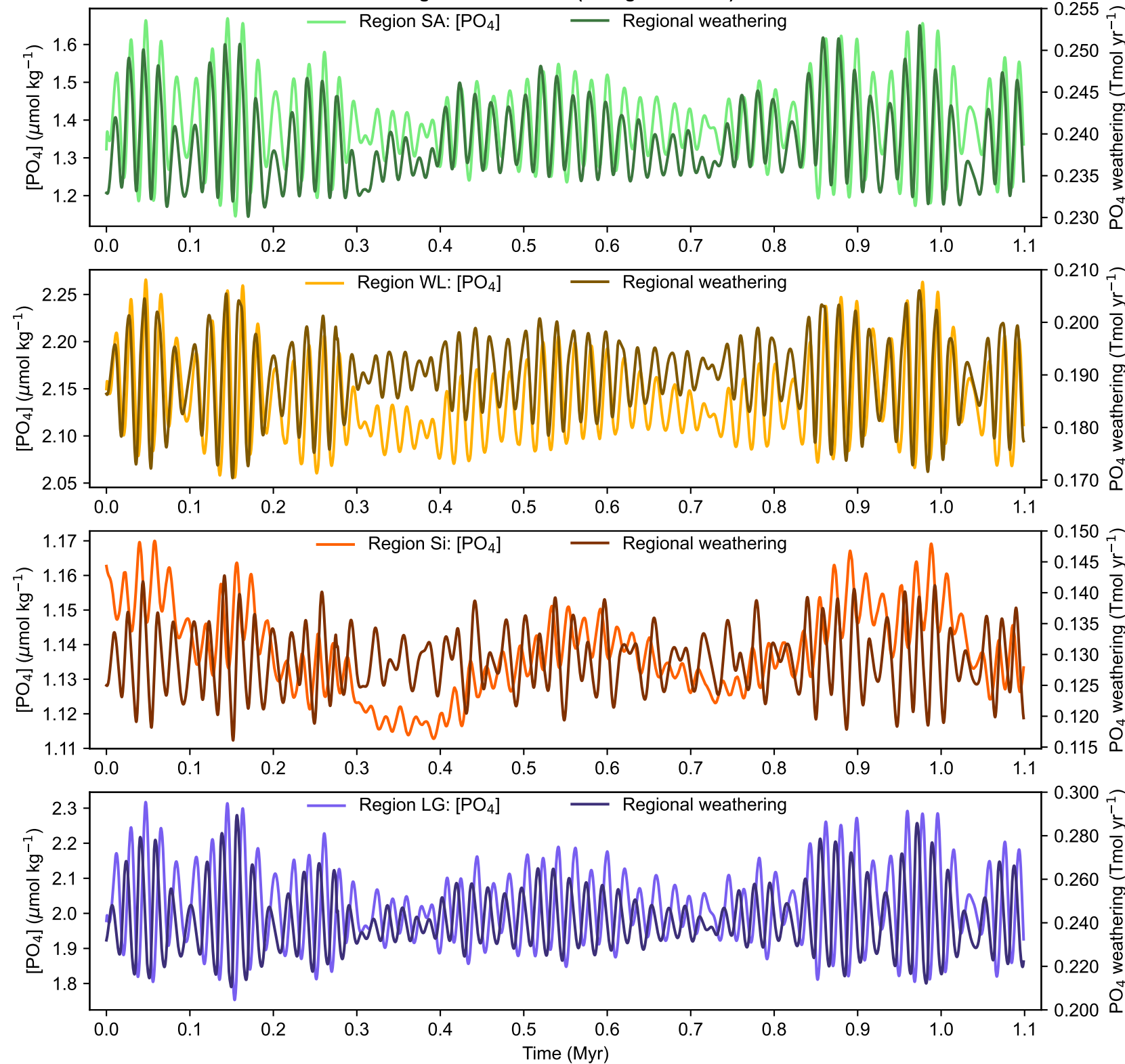
Regional time series (no lag correction)
