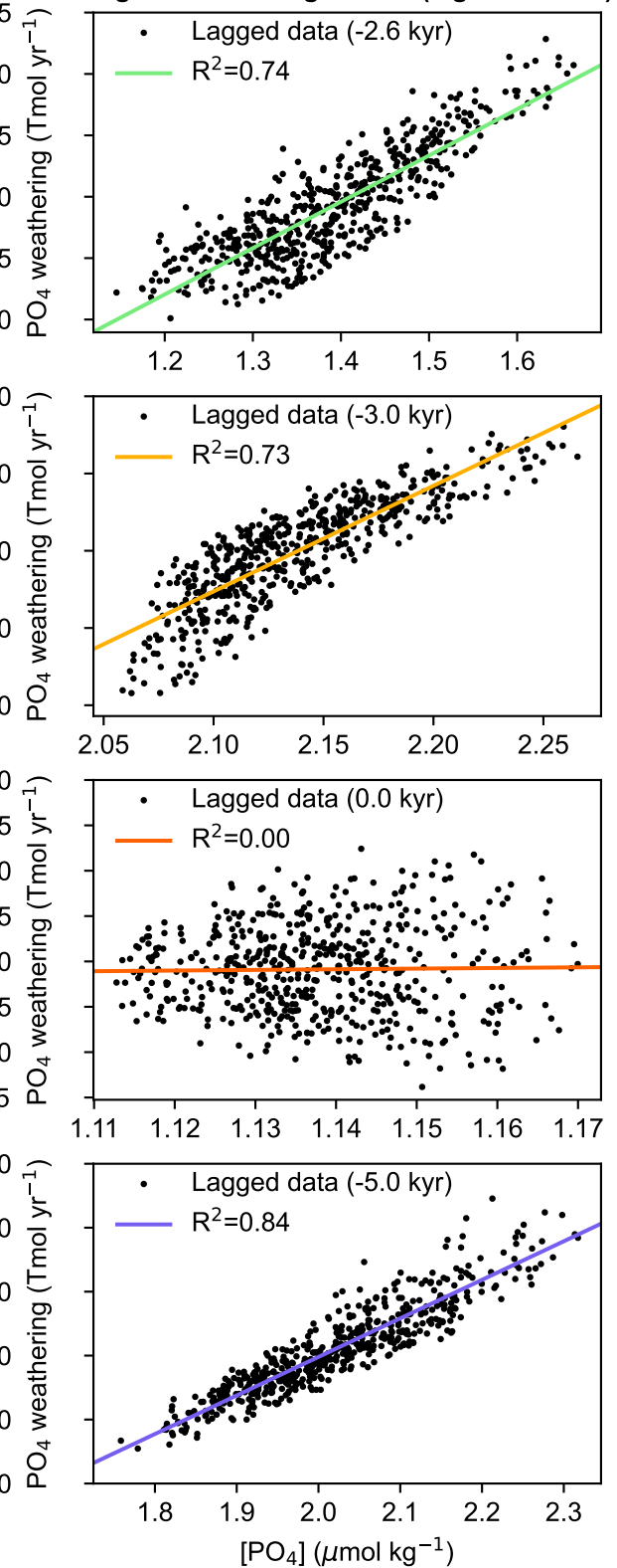
Regional linear regression (lag correction)
