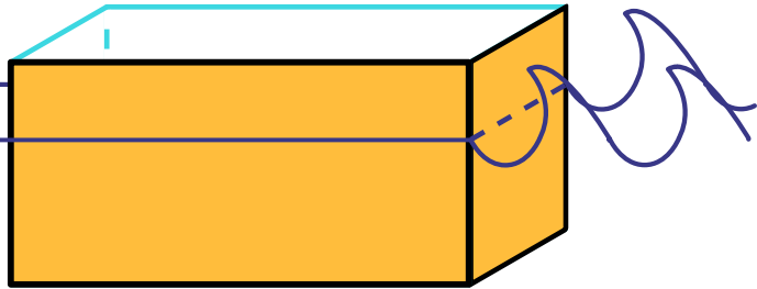
(c) Wave erosion
