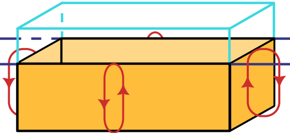
(b) Buoyant convection
