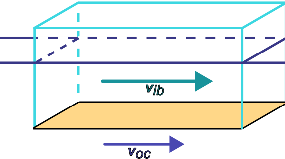
(a) Basal melt
