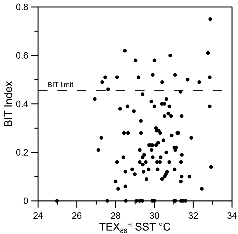
Figure S1: BIT compared to TEX 86 H SST values.
