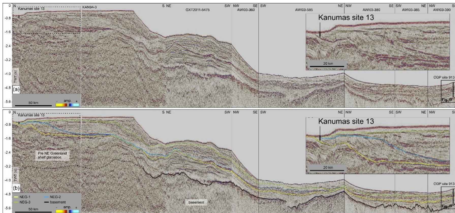
Figure S3: Composite seismic profile. See Fig. 1 for location. a) composite seismic profile from Norske Trough to Greenland Basin. Tied to Kanumas site 13 in Norske Trough and ODP Site 913 in Greenland Basin. b) Composite seismic profile with interpreted regional reflections NEG-1-NEG-3 (this study). Seismic courtesy of AWI, TGS and GEUS.
