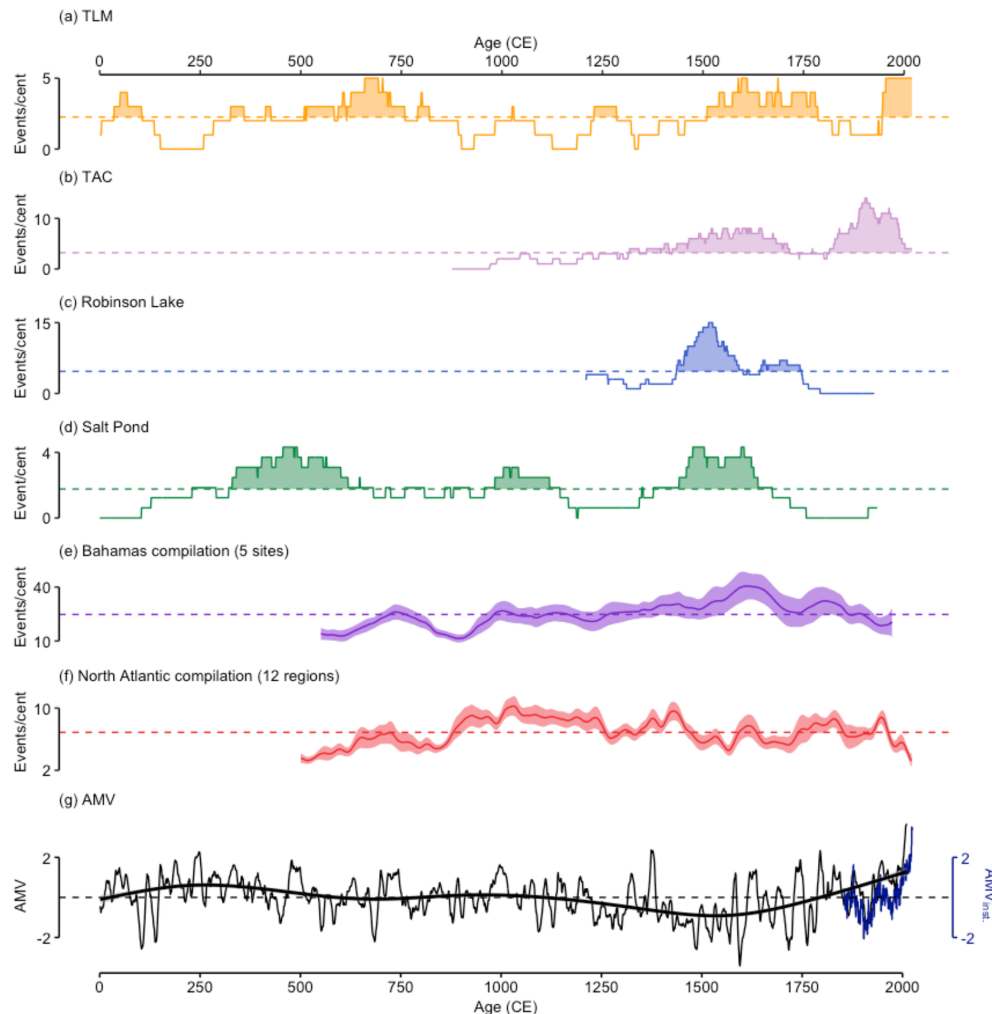
Figure 9. Events per century (Event/cent) from the Magdalen Islands and nearby regions reconstructions. (a–b) 100-year moving sum of storm events at TLM (orange line) and TAC (purple line). (c–e) Comparisons with previously published paleo-storm reconstructions. (c) 100-year moving sum of storm events from Robinson Lake, Nova Scotia, between 1210–1925 CE (Oliva et al., 2017). (d) 100-year moving sum of storm events from Salt Pond, Massachusetts, spanning the past 2000 years (Donnelly et al., 2015). (e) A smoothed 1500-year compilation of storm records from five Bahamian blue hole records, with the shaded area representing the confidence interval (Wallace et al., 2019, 2021a, b; Winkler et al., 2020, 2023). The location of the studies in (a)–(e) is shown in Fig. 6a. (f) Smoothed 1500-year compilation of storm records from 12 regions spanning from Belize to New England from Yang et al. (2024). (g) The annually-resolved Atlantic Multidecadal Variability (AMV) reconstruction based on titanium measurements from a varved lake record from Ellesmere Island, in Arctic Canada. An instrumental AMV record (1854–2023) is shown in dark blue (Huang et al., 2017).
