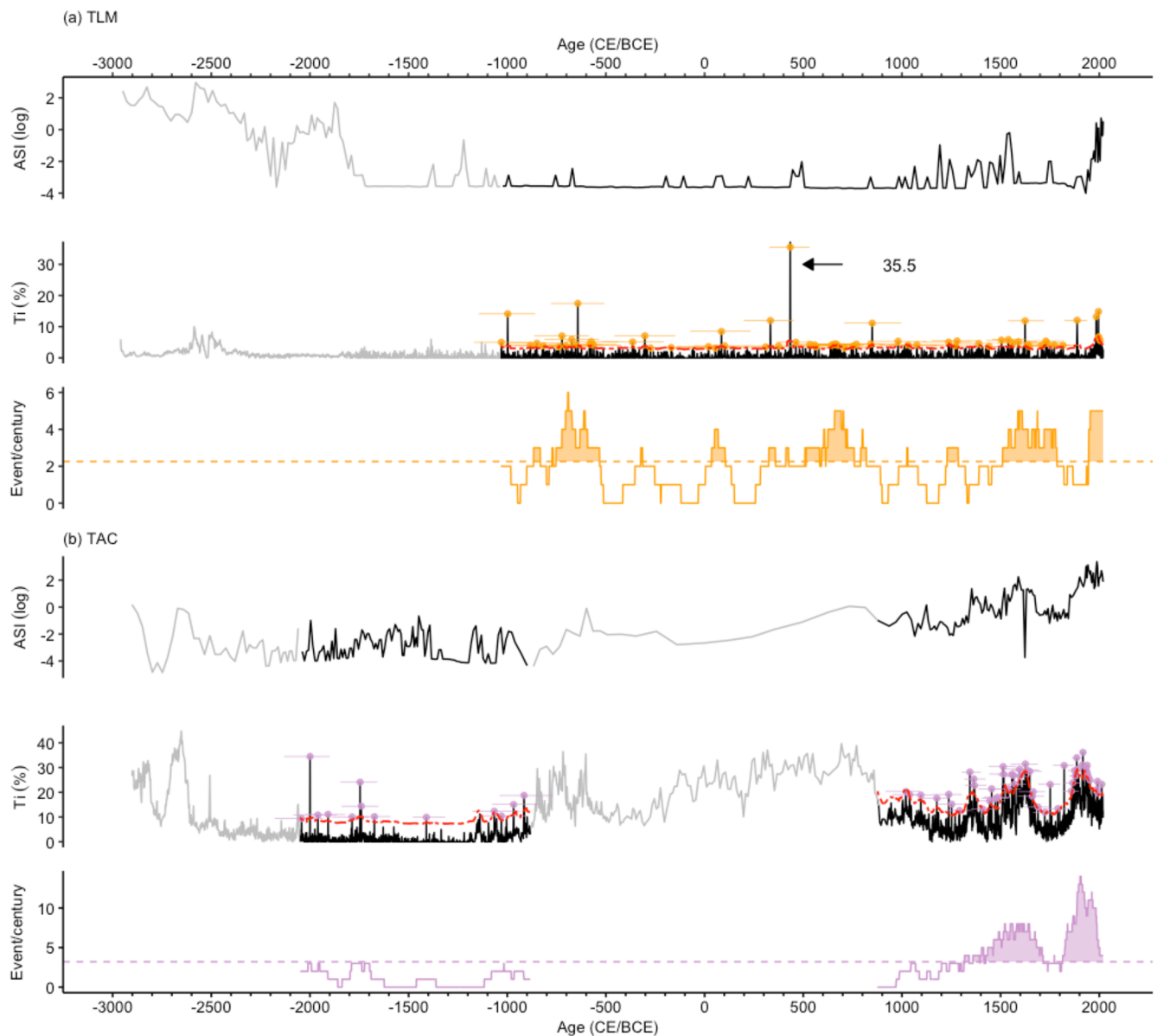
Figure 6. ASI (log), Ti (%), and storm events per century for TLM ( a ; in orange) and TAC ( b ; in purple). Solid black lines in ( a ) and ( b ) show ASI and Ti measurements during the periods of storm reconstruction, corresponding to the ombrotrophic portions of the core. Grey lines indicate the non-ombrotrophic portions of the cores, excluded from the reconstruction. Dashed red lines indicate the moving thresholds of event detection, calculated using the Tukey rule over a moving average (see Methods for details). Events are marked by orange (TLM) and purple (TAC) dots, with horizontal bars representing age uncertainty. Event frequencies are shown as a 100-year moving sum, with the average number of events per century shown as horizontal dashed lines.
