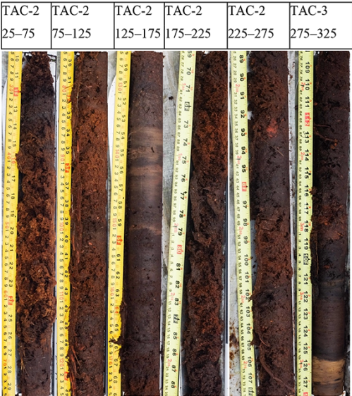
Figure C1. Photographs of the core segments taken at the TLM (a) and TAC (b) sites after extraction from the peatlands with depth indicated in cm. Only sections included in the TLM and TAC composite core are shown, except for the surface monoliths. (a) The basal sand unit is visible in TLM-1 650–700 between 693–700 cm. (b) The basal sand unit is visible in TAC-3 275–325 cm between 317–325 cm.
