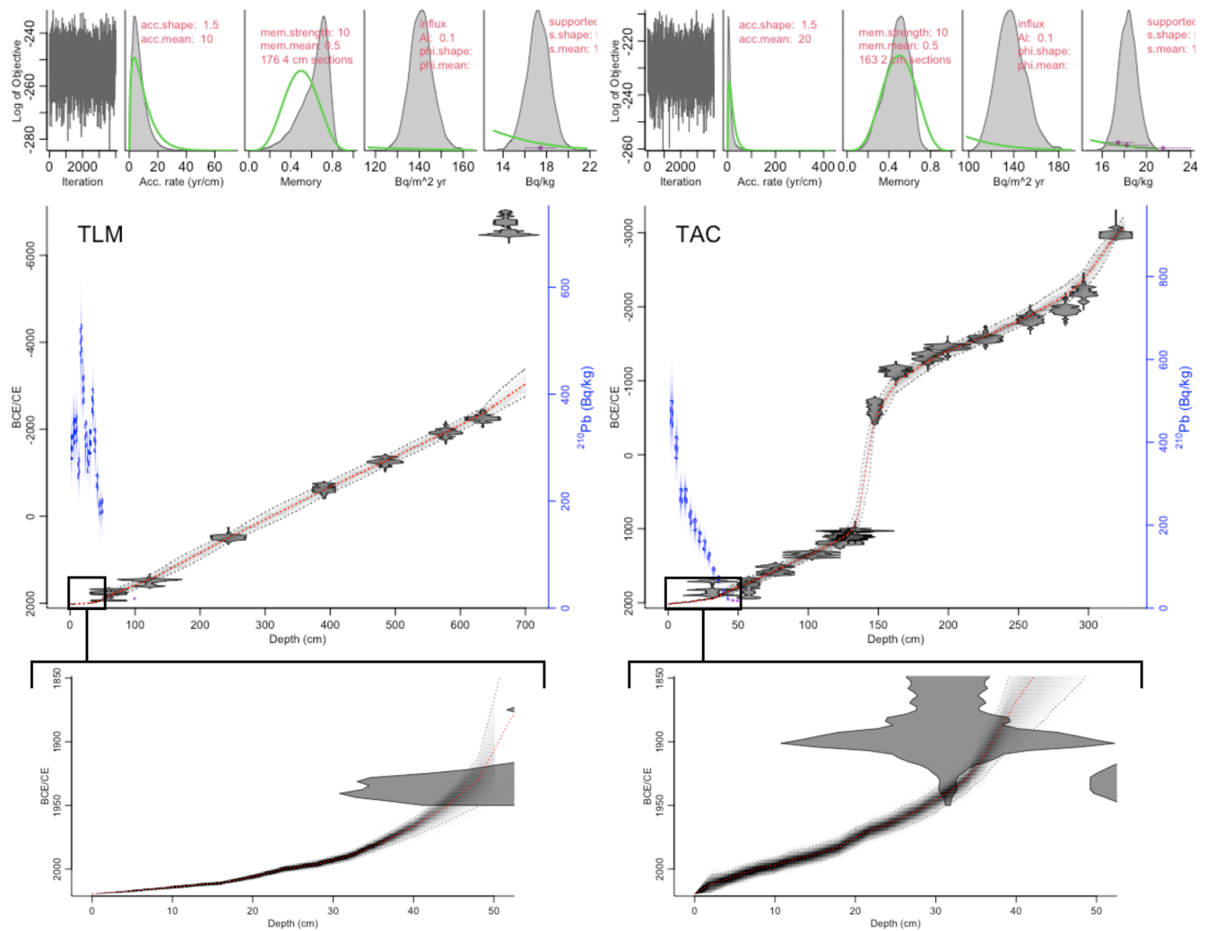
Figure D1. rplum-derived age-depth models for TLM (left) and TAC (right). Radiocarbon ( ^{14}\text{C} ) dates are shown in grey along the mean age model (dotted red). The rate of supported ^{210}\text{Pb} (right axis) is indicated by blue boxes on the left side (the blue boxes are the measured ^{210}\text{Pb} values, while the blue shadings represent the modelled ^{210}\text{Pb} values). For each core, the upper left panel shows the Markov Chain Monte Carlo (MCMC) iterations; followed by the prior (green curve) and posterior (grey histogram) distributions for the accumulation rate (second panel), memory (third panel), ^{210}\text{Pb} influx in \text{Bq m}^{-2} \text{yr}^{-1} (fourth panel) and supported ^{210}\text{Pb} in \text{Bq kg}^{-1} (fifth panel). A homing-in on the first 50 cm of the age-depth models is shown in the bottom panels.
