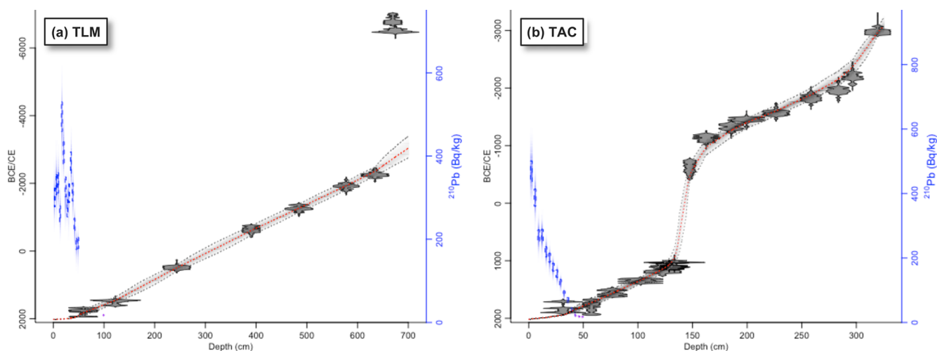
Figure 2. Rplum-derived age-depth models for TLM (a) and TAC (b). Radiocarbon ( ^{14}\text{C} ) dates are shown in grey along the mean age model (dotted red). The rate of supported ^{210}\text{Pb} (right axis) is indicated by blue boxes on the left side (the blue boxes are the measured ^{210}\text{Pb} values, while the blue shadings represent the modelled ^{210}\text{Pb} values). A complete version with the upper graphs and blown-up version of the ^{210}\text{Pb} diagrams is available in Fig. C1.
