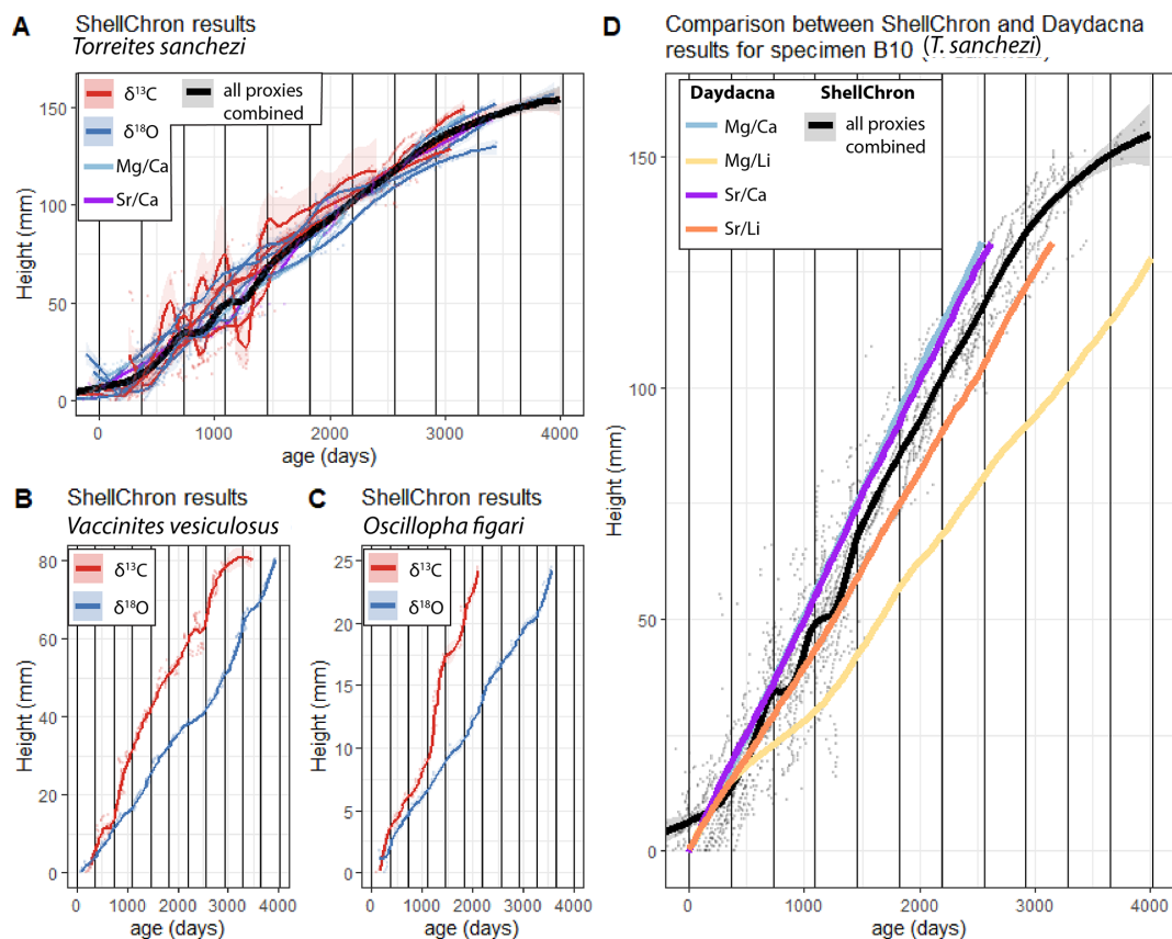
Figure 6. Plot of shell height vs. age in all specimens based on ShellChron modelling on Mg/Ca, Sr/Ca, \delta^{18}\text{O}_\text{c} and \delta^{13}\text{C} profiles in T. sanchezi (A), \delta^{18}\text{O}_\text{c} and \delta^{13}\text{C} profiles in V. vesiculosus (B) and \delta^{18}\text{O}_\text{c} and \delta^{13}\text{C} profiles in O. figari (C). Solid lines represent LOESS smoothed curves (span = 0.2) through the age-height data, with shaded areas indicating uncertainties around the growth models. (D) Comparison between ShellChron results for T. sanchezi specimen B10 profiles (combined chronology from all proxies; black line in panel (A)) and Daydacna results on subdaily-scale trace element profiles through the same specimen. Colours of curves and uncertainty envelopes represent the proxy on which age modelling was based (see legends in top-left corners of the panels).
