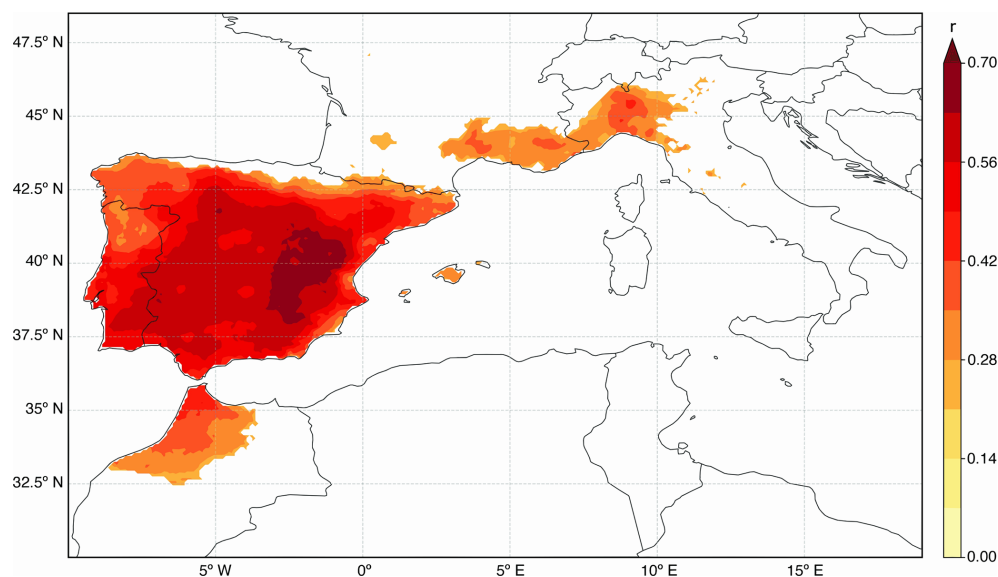
Figure 8. Spatial correlation patterns between the tree-ring residual chronology and accumulated rainfall during 320 d prior to 1 July (1951–2023).
