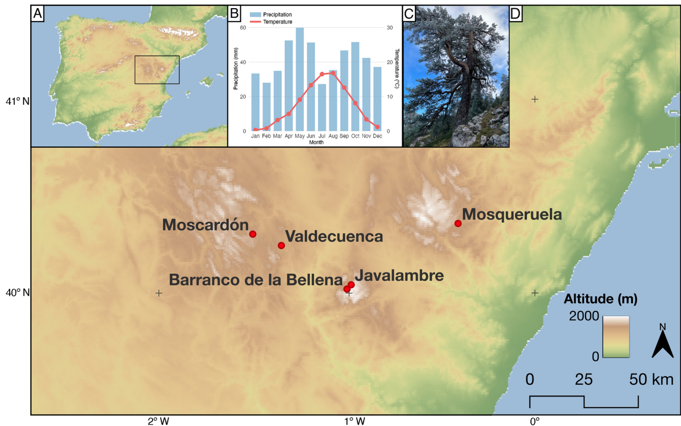
Figure 1. (A) Orographic map of the Iberian Peninsula and study area. (B) Climate diagram showing monthly precipitation from the ROCIO 5 \times 5 km grid (Peral García et al., 2017) and temperature from the Spain02 20 \times 20 km grid (Herrera et al., 2016), both calculated as the average value of the 16 grid cells closest to the coordinate 40.3^\circ \text{N} , 1.4^\circ \text{W} , for the period 1986–2015. (C) Photograph of a Pinus sylvestris at Barranco de la Bellena from which samples were taken. (D) Study area with the five sampling locations pointed in red.
