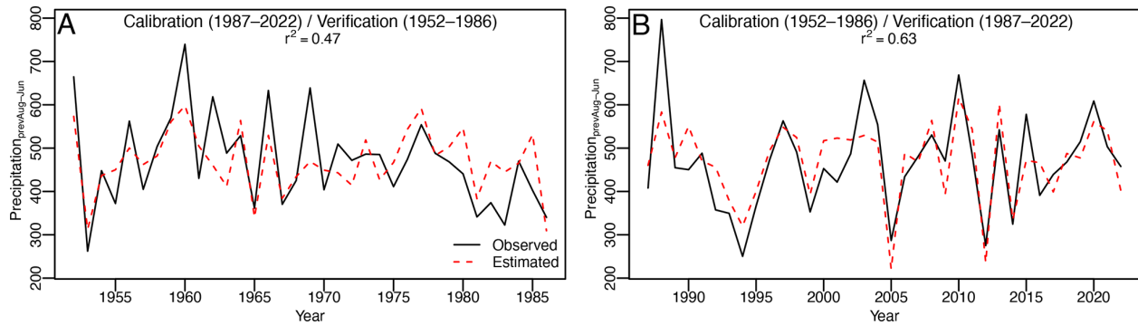
Figure 6. Calibration and verification results of the 11-month precipitation reconstruction ending in current-year 30 June ( \alpha = 0.05 ). (A) Calibration period: 1987–2022, verification period: 1952–1986. (B) Calibration period: 1952–1986, verification period: 1987–2022.
