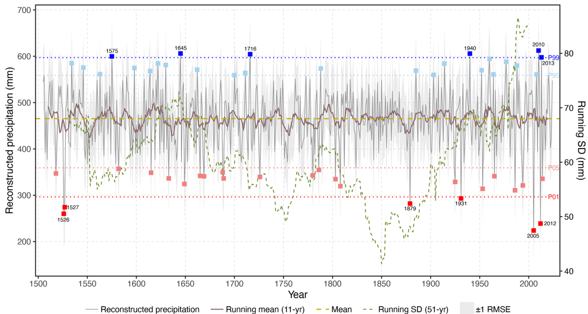
Figure 7. Annual rainfall reconstruction between 16 August of the previous year and 30 June of the current year back to 1505 (grey curve). A 11-year rolling mean is shown in brown. Dark blue squares represent years above 99th percentile, light blue squares between 95th and 99th percentiles, dark red below 1st percentile and light red between 1st and 5th. The variability in the reconstructed values is shown with a green dashed line showing a 51-year running standard deviation.
