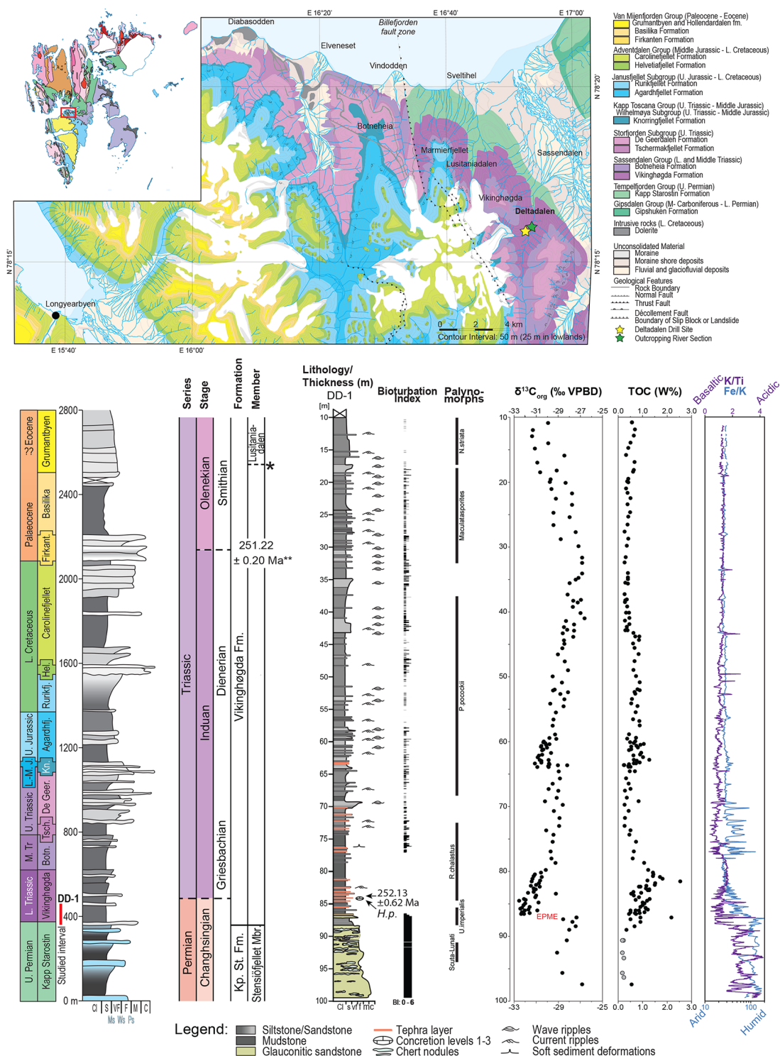
Figure 9. Top: geological map of central Spitsbergen highlighting the drill site (yellow star) and the adjacent Deltadalen river section (green star; geological map adapted from Major et al., 1992). Overview of the sedimentary section illustrating the lithostratigraphic formations in central Spitsbergen after Dallmann et al. (1999), Mørk et al. (1999b), Midtkandal et al. (2008), Nagy and Berge (2008), Dypvik et al. (2011), Blomeier et al. (2013), Lord et al. (2014), Koevoets et al. (2016), and Smellor and Larssen (2016). Bottom: the Permian–Triassic boundary as it appears in the Deltadalen DD-1 drill core. Modified after Zuchuat et al. (2020). EMPE – End-Permian Mass Extinction Event; Kp. St. Fm. – Kapp Starostin Formation; Mbr. – member; Fm – formation; H.p. – Hindeodus parvus ; * – member boundary after Mørk et al. (1999b); ** Induan–Olenekian boundary age after Burgess et al. (2014).
