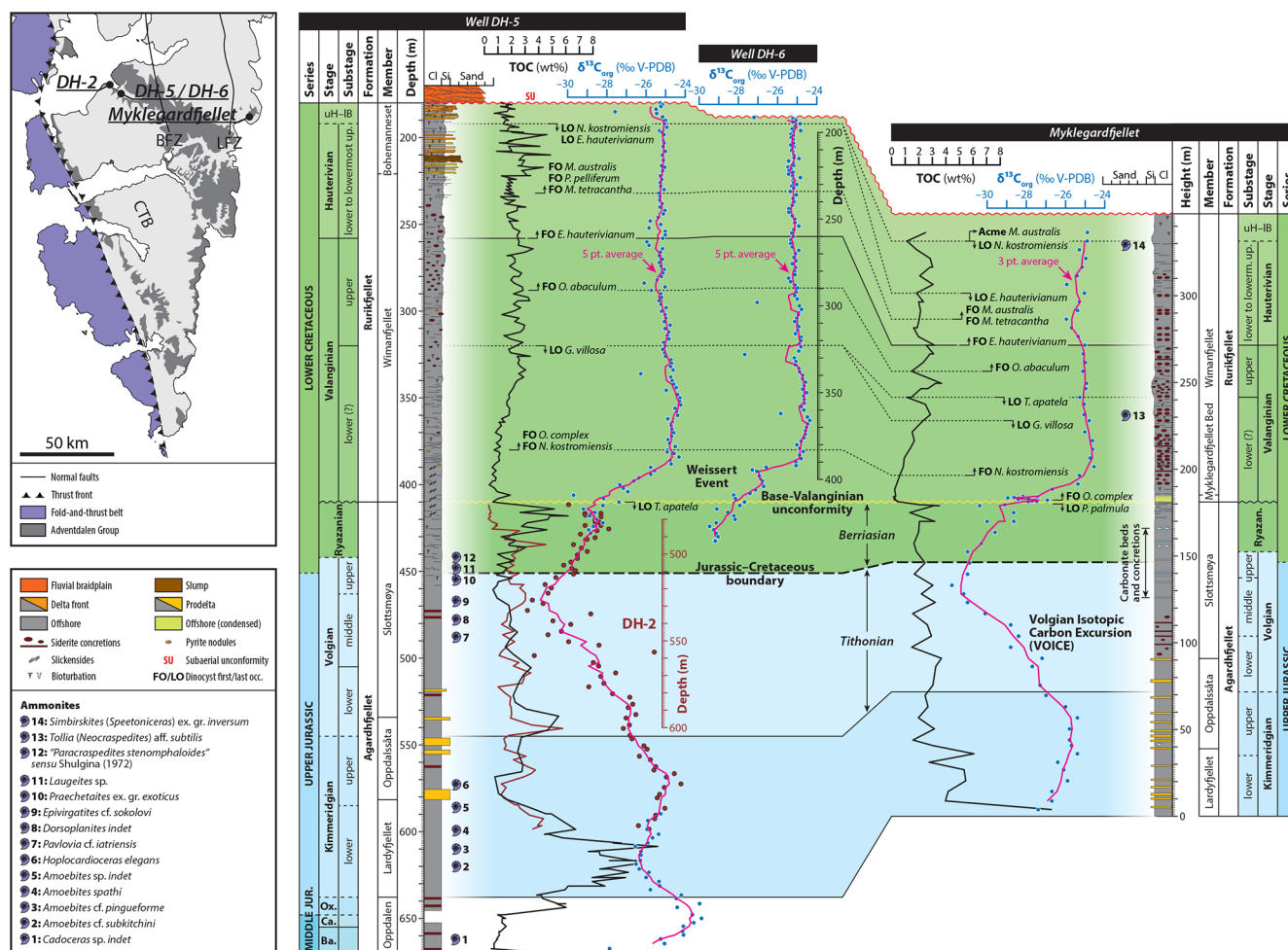
Figure 10. Correlation of organic stable carbon isotope ( \delta^{13}\text{C}_{\text{org}} ) stratigraphy between the cored wells DH-2, DH-5, and DH-6 and the Myklegardfjellet outcrop section, calibrated by total organic carbon (TOC) trends, and dinocyst and ammonite biostratigraphy (compiled and modified from Jelby et al. 2020b, 2025, and Koevoets et al., 2016, 2018). The boundary between the Agardhfjellet and Rurikfjellet formations (conforming to a base-Valanginian unconformity and demarcated by a marked drop in TOC values) is used as a correlation datum. Note the clear expression of the Weissert Event and “Volgian Isotopic Carbon Excursion” (VOICE) in the different sections. uH–lB, upper Hauterivian–lower Barremian. For details on the dinocyst bio-events, the reader is referred to Jelby et al. (2020b, 2025) and Śliwińska et al. (2020).
