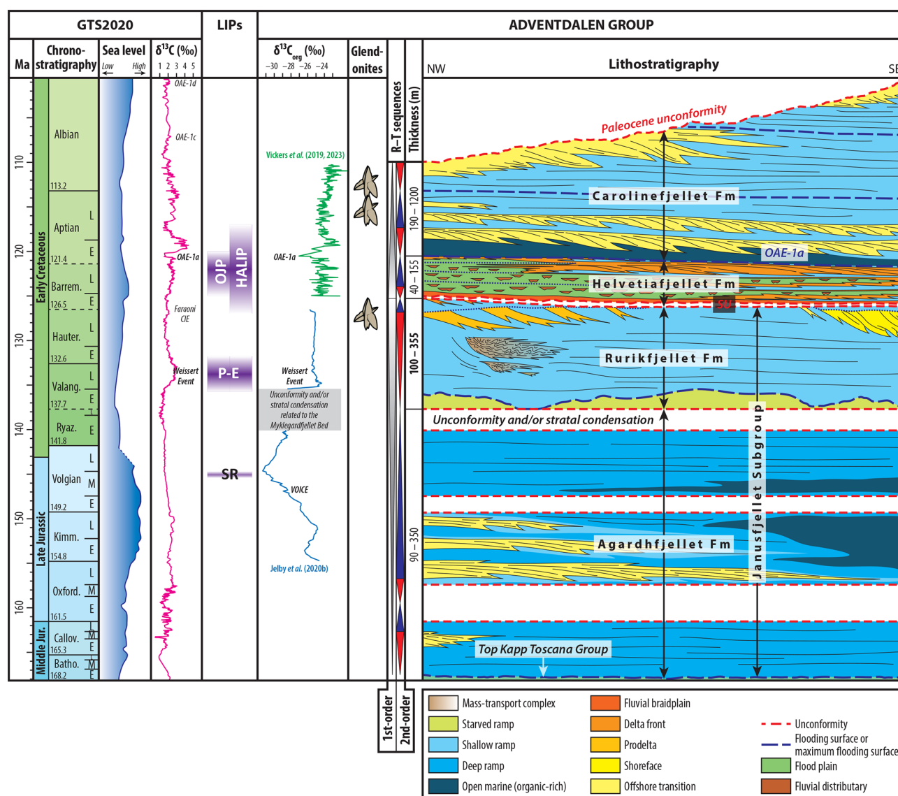
Figure 11. Overview of the Upper Jurassic and Lower Cretaceous stratigraphy of Svalbard plotted against time, from Jelby et al. (2025), based on Grundvåg et al. (2017, 2019). To the left of the stratigraphic summary chart, thicknesses of the formations, first- and second-order regressive-transgressive sequences, occurrence of glendonites (Vickers et al., 2019a), LIP volcanic episodes (see references in Vickers et al., 2023), and organic stable carbon isotopes (see Jelby et al., 2025, and references therein) are shown. These are plotted against global \delta^{13}\text{C} trends, sea level, and ages from the Geological Time Scale 2020 (Gale et al., 2020; Hesselbo et al., 2020).
