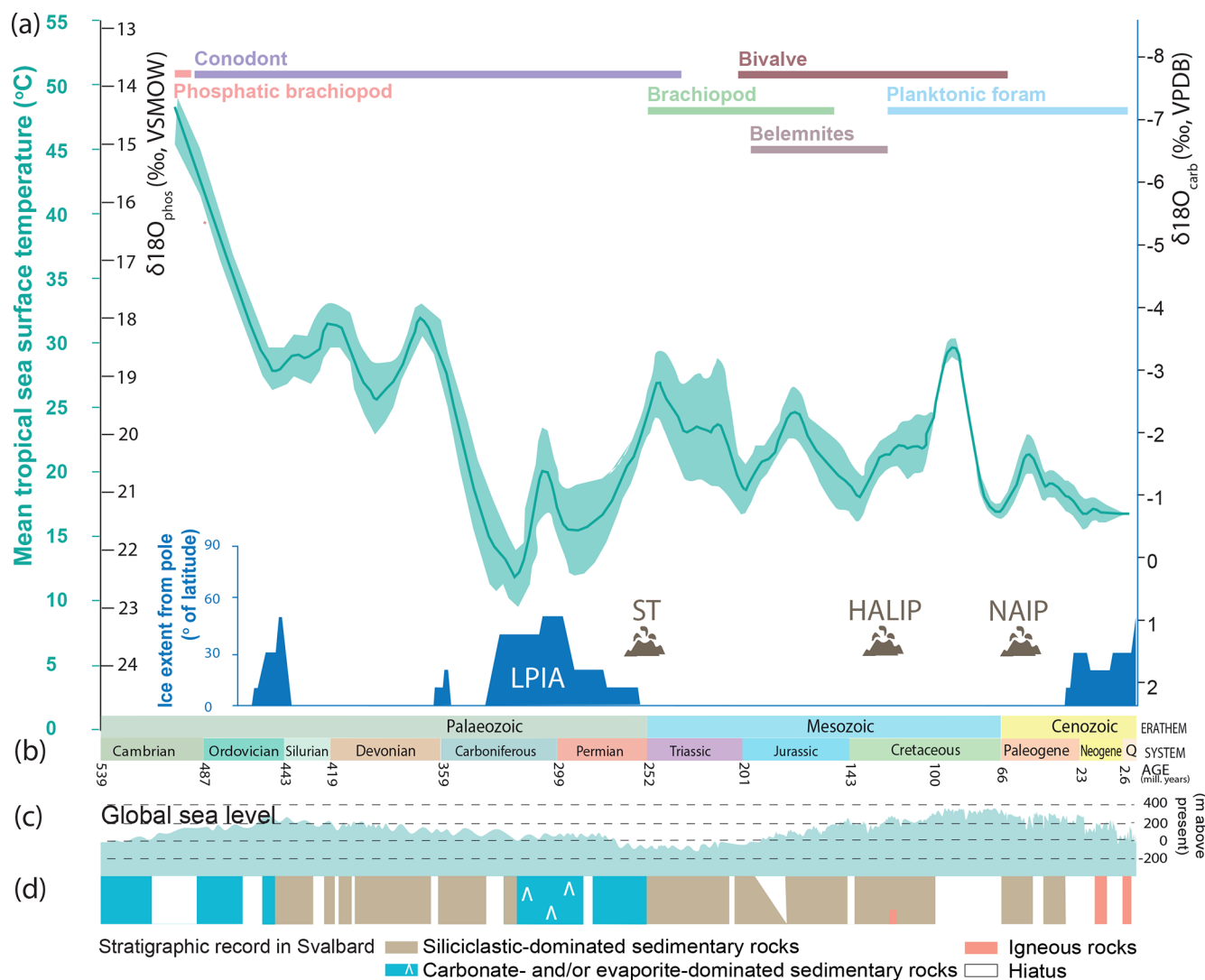
Figure 1. The stratigraphic record of Svalbard in a global deep-time climate context. (a) Global data coverage including mean tropical sea surface temperatures per Myr marked as a green curve, with shaded area 95 % confidence intervals, based on oxygen isotopes from phosphatic and carbonate fossils from Scotese et al. (2021), after Song et al. (2019). The scale of \delta^{18}\text{O}_{\text{phos}} (black axis on the left) represents phosphatic fossils (phosphatic brachiopod, conodont, and fish). The scale of \delta^{18}\text{O}_{\text{carb}} (black axis on the right) represents carbonate fossils (belemnite, bivalve, brachiopod, planktonic foraminifera). The ice extent from pole, marked in blue, after Macdonald (2020), LPIA – Late Paleozoic Ice Age; major LIPs recorded in Svalbard: ST – Siberian Traps, HALIP – High Arctic Large Igneous Province, NAIP – North Atlantic Igneous Province, (b) Phanerozoic timescale, (c) sea-level curve (after Dallmann, 2015, based on work of the International Commission on Stratigraphy), and (d) overview of the geological record of Svalbard (modified from Dallmann, 2015).
