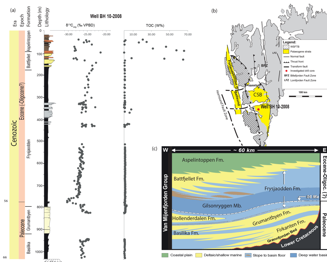
Figure 12. (a) Geochemical data from well BH 10-2008 are from Doerner et al. (2020), and borehole stratigraphy is after Grundvåg et al. (2014). (b) Geological map showing the outline of Paleocene deposits and position of BH 10-2008 from Helland-Hansen and Grundvåg (2021). (c) Lithostratigraphic summary of the Paleogene deposits of the Central Spitsbergen Basin. Modified from Helland-Hansen and Grundvåg (2021). The age of the Paleocene–Eocene boundary is from Charles et al. (2011) and Harding et al. (2011).
