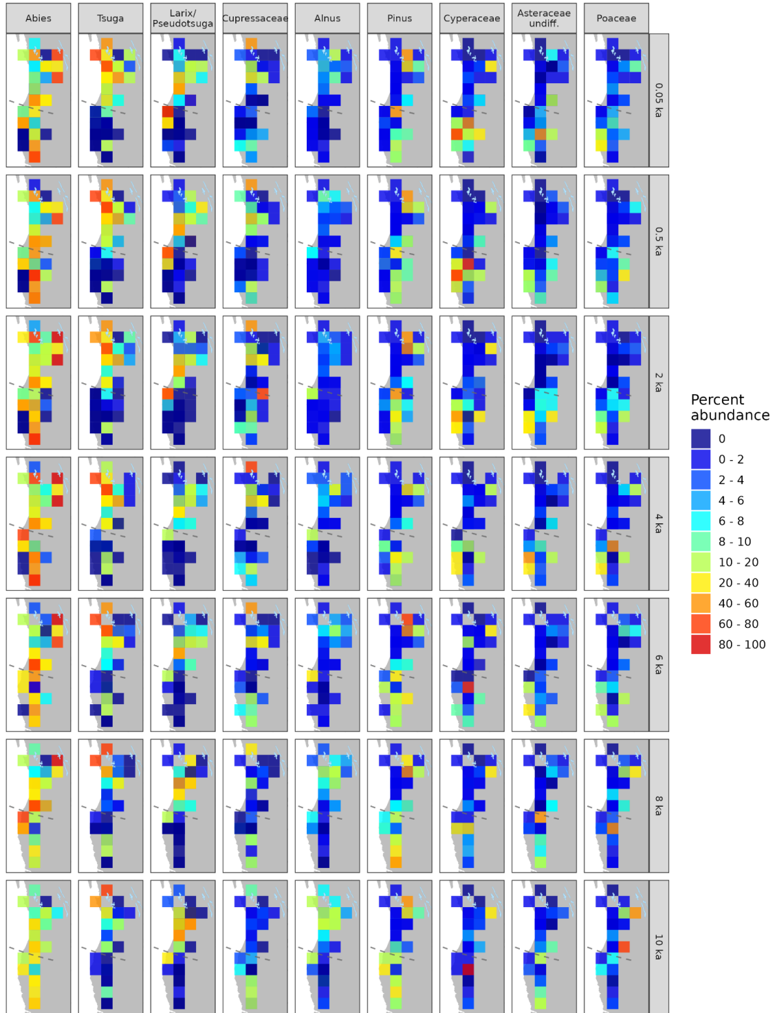
Figure S14: Maps of taxon percent abundance inferred using REVEALS for Abies , Alnus , Asterx , Cupressaceae , Cyperaceae , Larix , Pinus , Poaceae , and Tsuga for the the Pacific Coast, Cascade, and Sierra Nevada Ranges (PCCS) case study region. Estimates are presented on an equal area projected grid,
