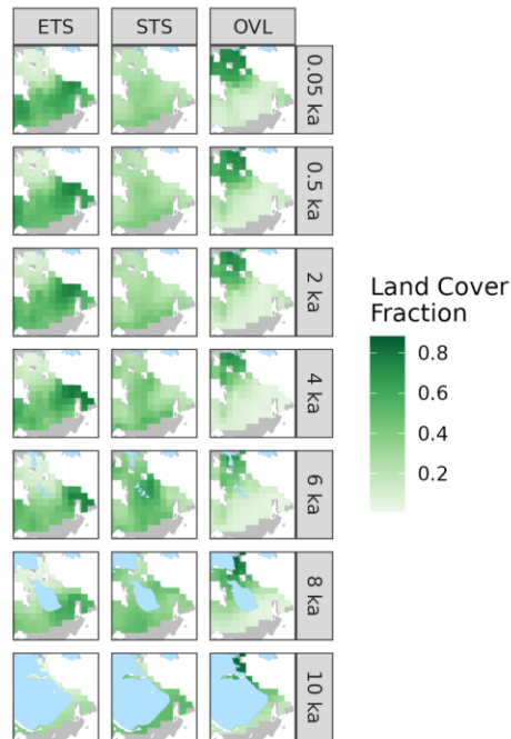
Figure S9: Interpolated REVEALS-based estimates of fractional cover for evergreen trees and shrubs (ETS), summergreen trees and shrubs (STS), and open vegetation/land (OVL) for the Eastern Canada (ECAN) case study region. Estimates are presented on an equal area projected grid, for selected time periods, with ages reported as ka. Map ordering follows the geological convention of oldest maps at bottom. Ice extent shown in light blue.
