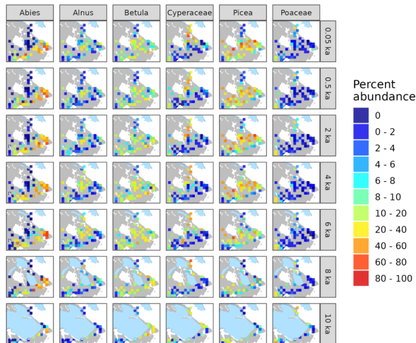
Figure S10: Maps of taxon percent abundance inferred using REVEALS for Abies , Alnus , Betula , Cyperaceae , Picea , and Poaceae for the Eastern Canada (ECAN) case study region. Estimates are
