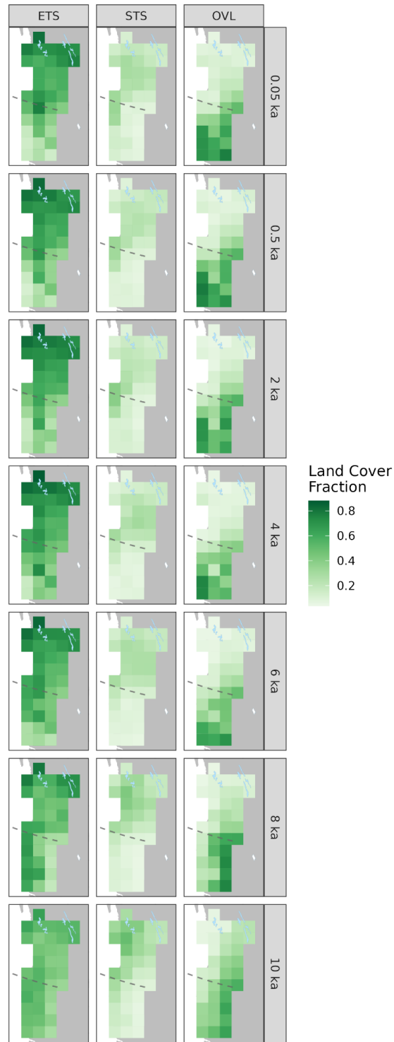
Figure S13: Interpolated REVEALS-based estimates of fractional cover for evergreen trees and shrubs (ETS), summergreen trees and shrubs (STS), and open vegetation/land (OVL) for the Pacific Coast, Cascade, and Sierra Nevada Ranges (PCCS) case study region. Estimates are presented on an equal area
