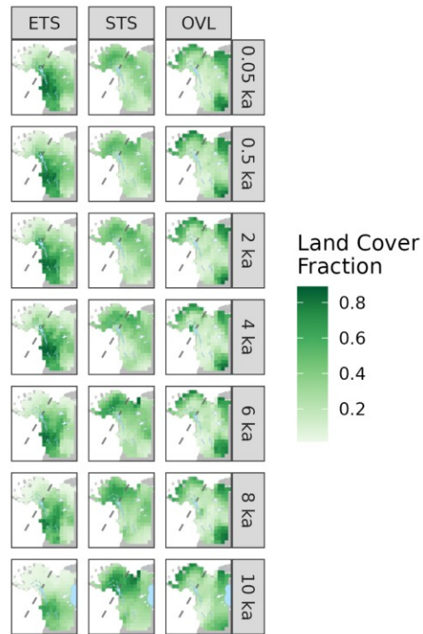
Figure S11: Interpolated REVEALS-based estimates of fractional cover for evergreen trees and shrubs (ETS), summergreen trees and shrubs (STS), and open vegetation/land (OVL) for the Western Canada and Alaska (WCAN/AK) case study region. Estimates are presented on an equal area projected grid, for selected time periods, with ages reported as ka. Map ordering follows the geological convention of oldest maps at bottom. Ice extent shown in light blue.
