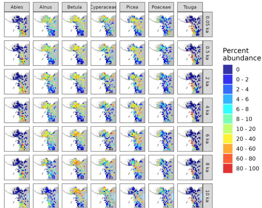
Figure S12: Maps of taxon percent abundance inferred using REVEALS for Abies , Alnus , Betula , Cyperaceae , Picea , Poaceae , and Tsuga for the Western Canada and Alaska (WCAN/AK) case study region. Estimates are presented on an equal area projected grid, for selected time periods, with ages reported as ka. Map ordering follows the geological convention of oldest maps at bottom. Ice extent shown for the in light blue.
