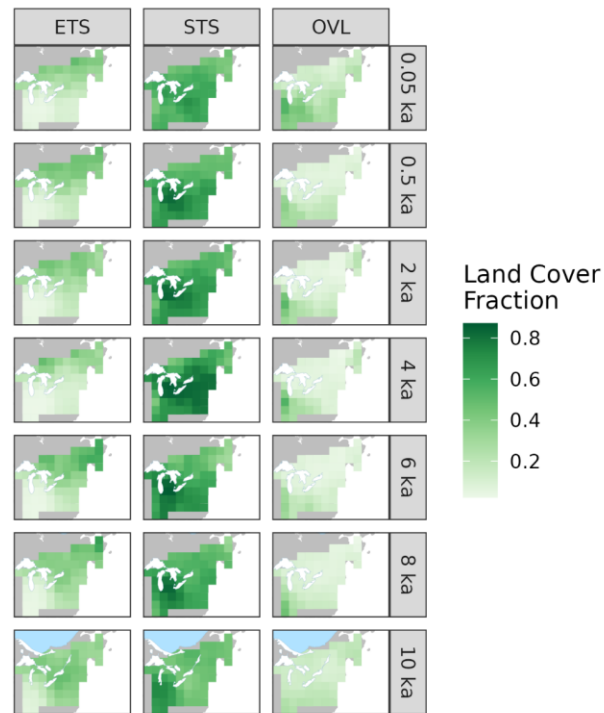
Figure S7: Interpolated REVEALS-based estimates of fractional cover for evergreen trees and shrubs (ETS), summergreen trees and shrubs (STS), and open vegetation/land (OVL) for the Northeastern US & Southeastern Canada (NEUS/SEC) case study region. Estimates are presented on an equal area projected grid, for selected time periods, with ages reported as ka. Map ordering follows the geological convention of oldest maps at bottom. Ice extent shown in light blue.
