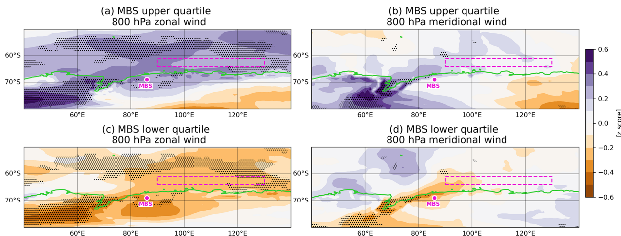
Figure 2. Composite maps of the averaged austral winter (JJA) ERA5 800 hPa meridional and zonal wind anomalies for the Mount Brown South site average (MBS CI^{-} ) (a) upper and (c) lower quartile of zonal wind and (b) upper and (d) lower quartile of meridional wind. Upper quartiles (a, b) [1982, 1986, 1987, 1993, 1996, 1997, 2009, 2012, 2014, 2015] and lower quartiles (c, d) [1980, 1981, 1983, 1990, 1991, 1995, 1999, 2001, 2010, 2011]. The stippling indicates points where the K-S test p value is < 0.1 . The MBS northeast coast box is highlighted in fuchsia and the fuchsia dot indicates MBS.
