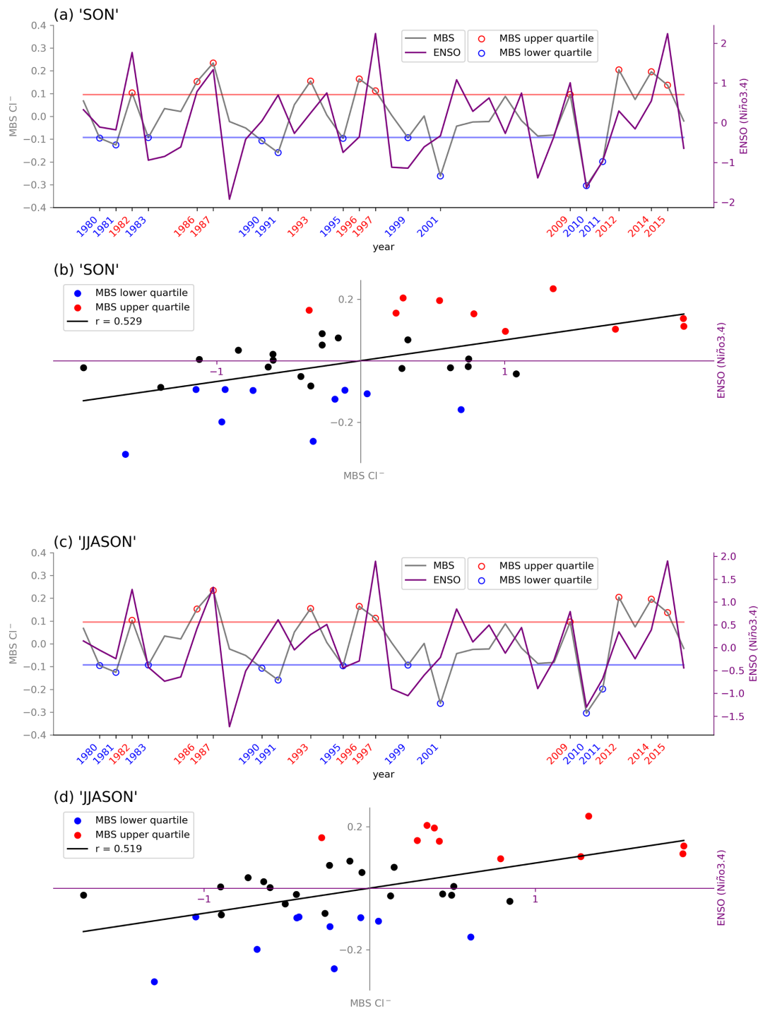
Figure A3. Time series of the annual detrended, log-transformed sea salt concentrations for the Mount Brown South site average (MBS \text{Cl}^- ) and the detrended (a) (September–November), (c) (July–November) El Niño–Southern Oscillation region SST anomalies (Niño3.4). Red line (blue line) indicates the upper (lower) quartile boundary. Scatter plot shows the relationship between the MBS \text{Cl}^- and (b) (September–November) Niño3.4 (d) (July–November) Niño3.4 with the MBS upper (lower) quartile highlighted by the red dots (blue dots) based on the period 1979–2016.
