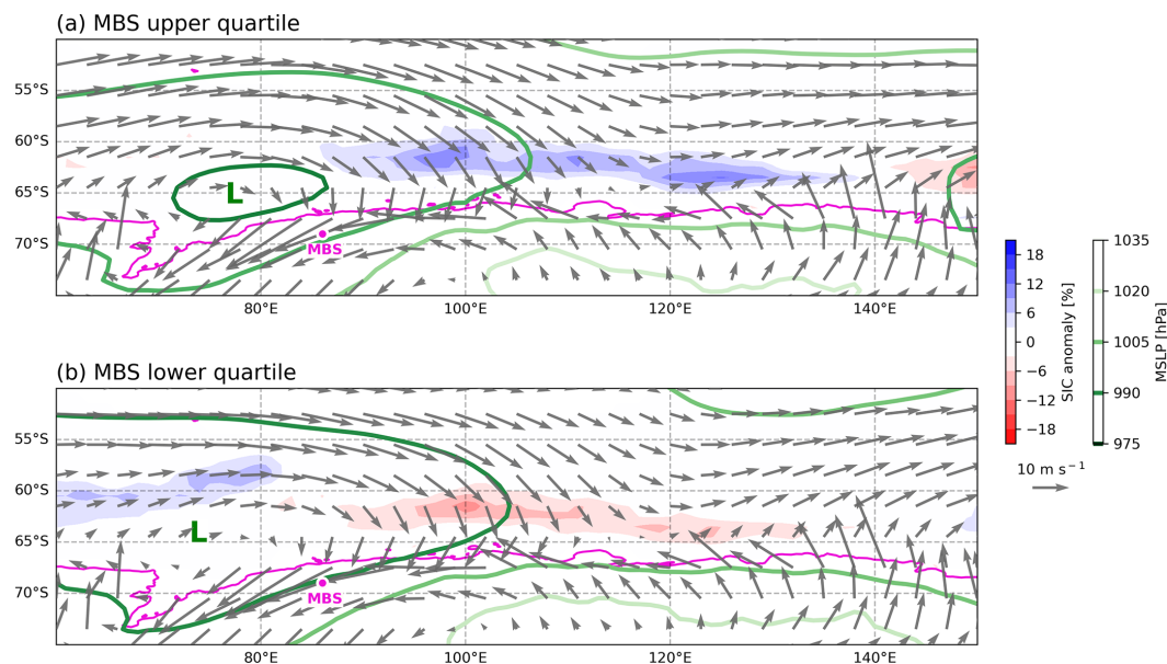
Figure 4. Composite maps of the austral winter (JJA) daily ERA5 mean sea level pressure (contours), daily ERA5 800 hPa mean wind vectors averaged over the 5 maximum precipitation days in austral winter, and (monthly) austral winter (JJA) averaged sea ice concentration (shading) for the Mount Brown South site average (MBS \text{CI}^- ) (a) upper [1982, 1986, 1987, 1993, 1996, 1997, 2009, 2012, 2014, 2015] and (b) MBS lower quartile [1980, 1981, 1983, 1990, 1991, 1995, 1999, 2001, 2010, 2011]. The fuchsia dot indicates MBS.
