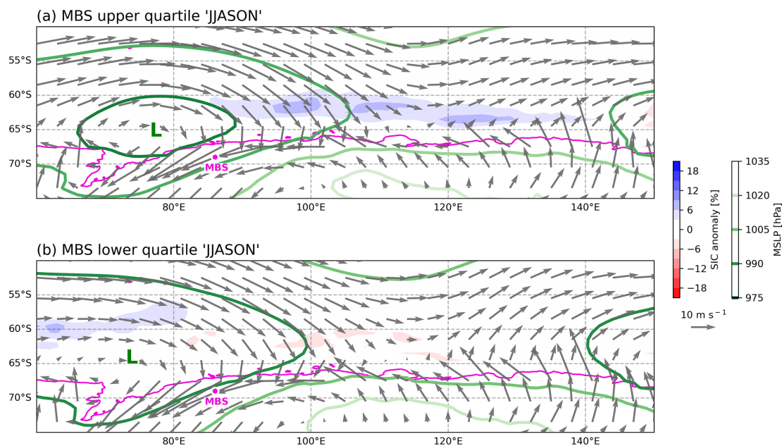
Figure A7. Composite maps of the daily ERA5 mean sea level pressure (contours), daily ERA5 800 hPa mean wind vectors averaged over the 5 maximum precipitation days in JJASON, JJASON averaged sea ice concentration (shading) for the Mount Brown South site average (MBS CI^- ) (a) upper [1982, 1986, 1987, 1993, 1996, 1997, 2009, 2012, 2014, 2015] and (b) MBS lower quartile [1980, 1981, 1983, 1990, 1991, 1995, 1999, 2001, 2010, 2011]. The green dot indicates MBS.
