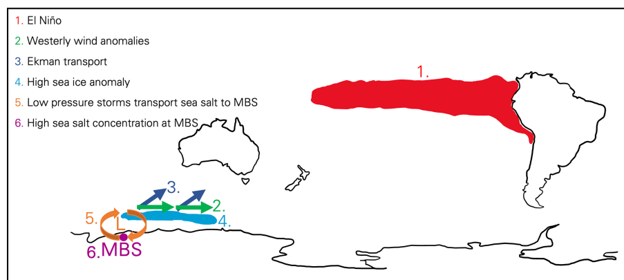
Figure 9. Schematic depicting the winter conditions associated with high sea salt concentration in the MBS ice core. Generated from composite maps (Figs. 2, 3, 5, 6).
