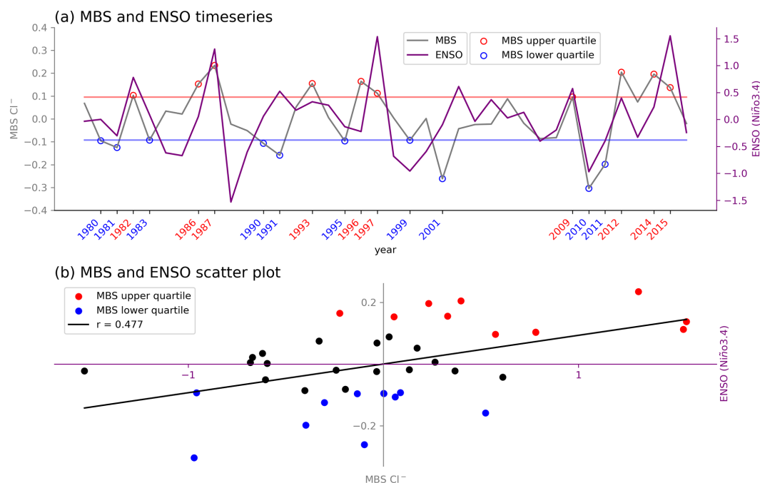
Figure 5. (a) Time series of the annual detrended, log-transformed sea salt concentrations for the Mount Brown South site average (MBS \text{CI}^- ) and the detrended (June–August) El Niño–Southern Oscillation region SST anomalies (Niño3.4). Red line (blue line) indicates the MBS upper (lower) quartile boundary. Red and blue years on the x axis represent the MBS upper and lower quartile years. (b) Scatter plot shows the relationship between the two time series with the MBS upper (lower) quartile highlighted by the red dots (blue dots) based on the period 1979–2016.
