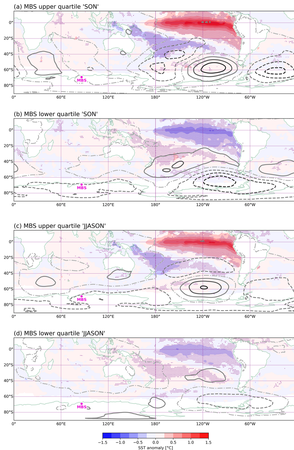
Figure A4. Composite maps of the (a, b) September–November, (c, d) July–November sea surface temperature anomaly (shading) and ERA5 mean sea level pressure anomaly (contours) for the Mount Brown South site average (MBS \text{CI}^- ) (a, c) upper [1982, 1986, 1987, 1993, 1996, 1997, 2009, 2012, 2014, 2015] and (b, d) lower quartile [1980, 1981, 1983, 1990, 1991, 1995, 1999, 2001, 2010, 2011]. High (low) MSLP anomalies shown by solid (dashed) contours, with darker shades of grey indicating stronger anomalies. The contour line graduations indicate 0.8 hPa. The stippling indicates points where the sea surface temperature anomaly (shading) K-S test p value is < 0.1 . The fuchsia dot indicates MBS.
