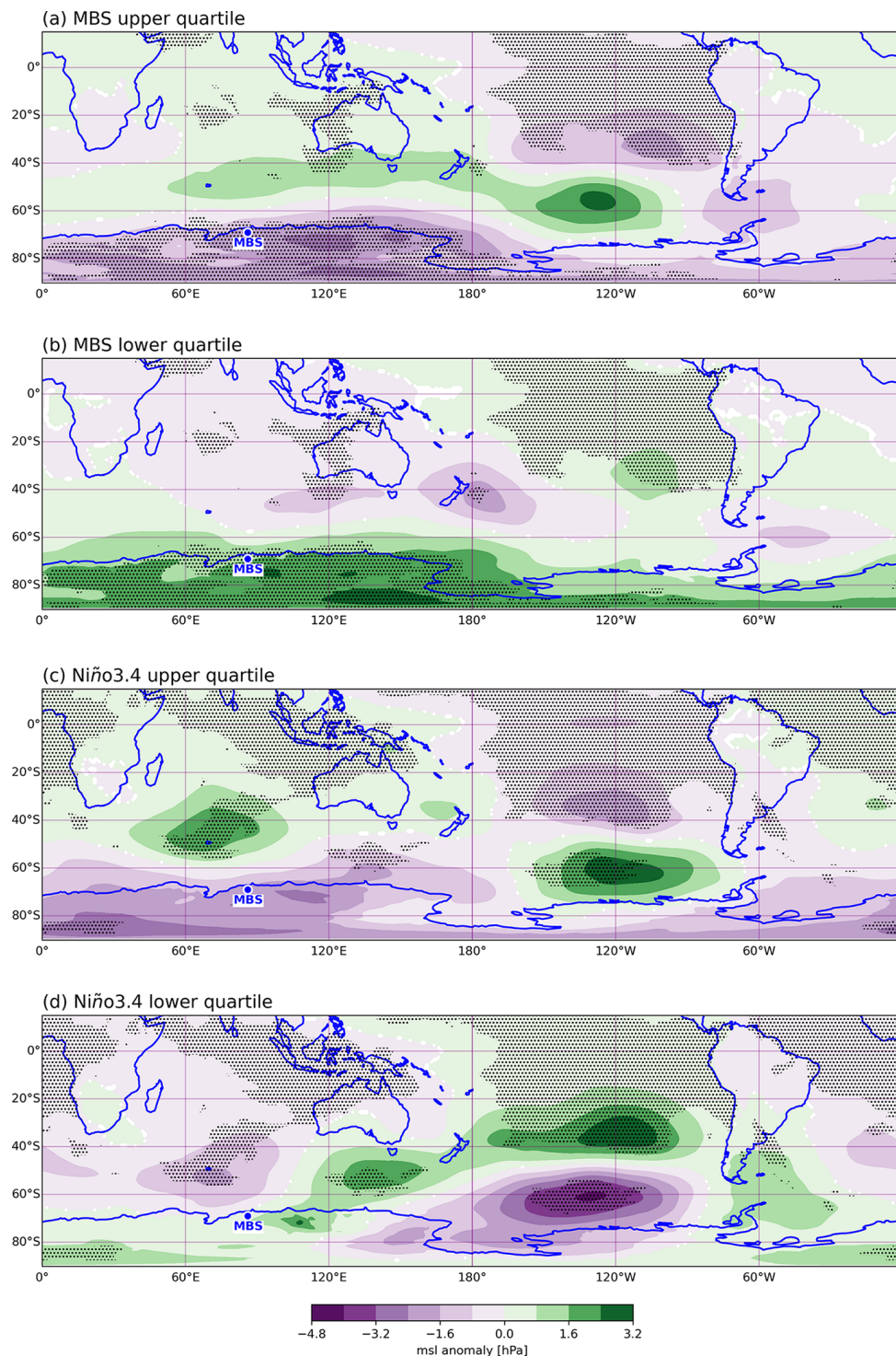
Figure A1. Composite maps of the winter ERA5 mean sea level pressure anomaly for the Mount Brown South site average (MBS \text{Cl}^- ) (a) upper [1982, 1986, 1987, 1993, 1996, 1997, 2009, 2012, 2014, 2015] and (b) lower quartile [1980, 1981, 1983, 1990, 1991, 1995, 1999, 2001, 2010, 2011] and for the Niño3.4 (c) upper [1982, 1987, 1991, 1993, 1997, 2002, 2004, 2009, 2012, 2015] and (d) lower quartile [1984, 1985, 1988, 1989, 1998, 1999, 2000, 2007, 2010, 2011]. The stippling indicates points where the mean sea level pressure anomaly K-S test p value is < 0.1 . The blue dot indicates MBS.
