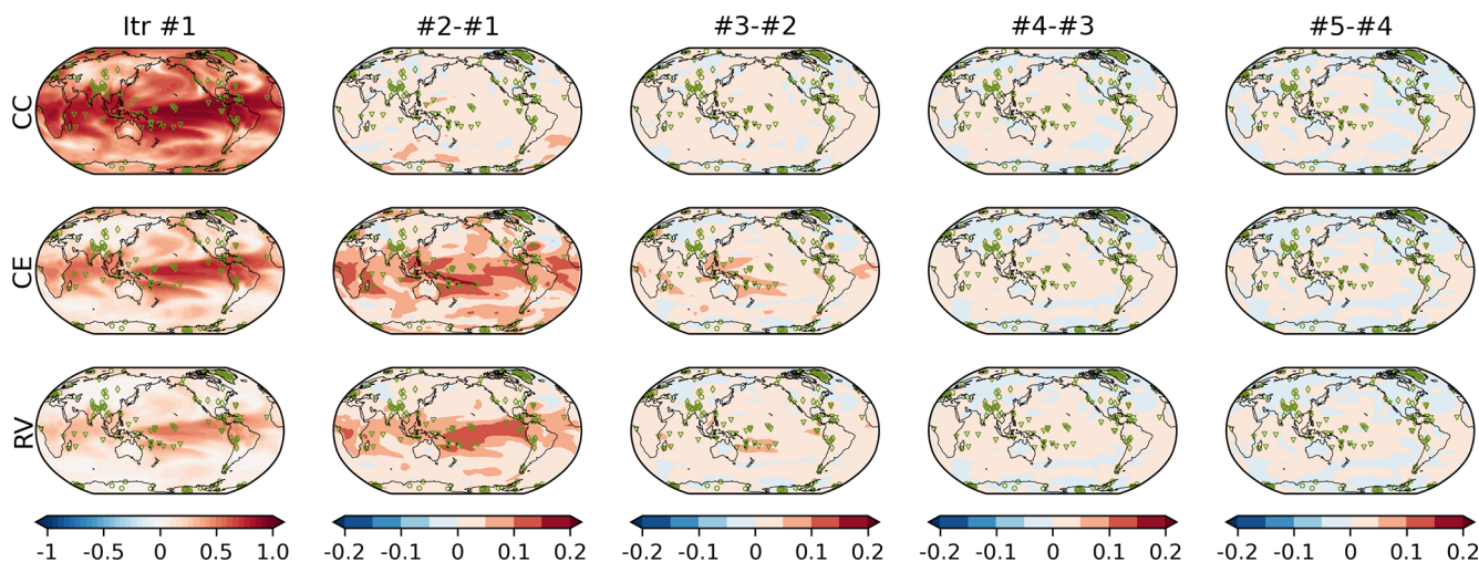
Figure 5. Reconstruction skill score of (top) CC, (middle) CE, and (bottom) RV in OSSE EST Rx16. Left column shows the reconstruction skill at the first iteration (i.e., without observation error estimation). Second to fifth columns show the skill difference from the previous iteration; for instance, the second column shows the difference between second and first iterations. Markers in each map show the position of proxies.
