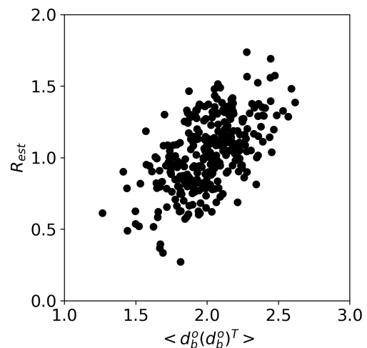
Figure 14. Relationship between \langle d_b^o(d_b^o)^T \rangle and R_{est} at the 20th iterations for the simplified two-variable model.
