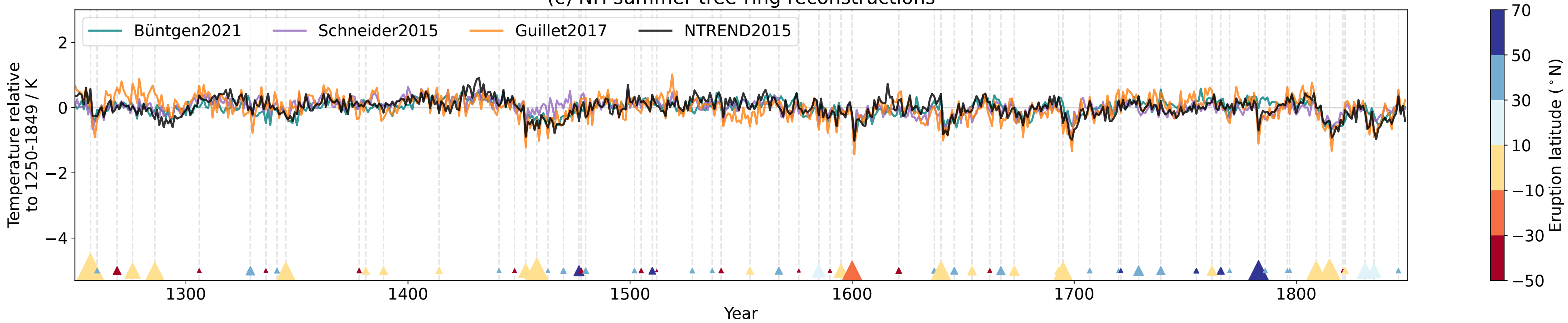
(c) NH summer tree-ring reconstructions
