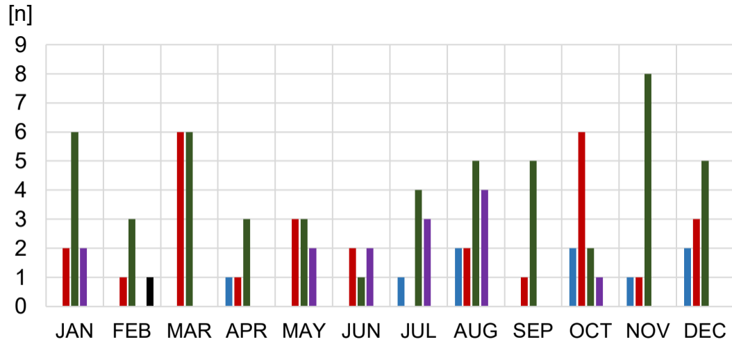
(a) Fresh and strong breeze Gale Storm Squall Tornado
