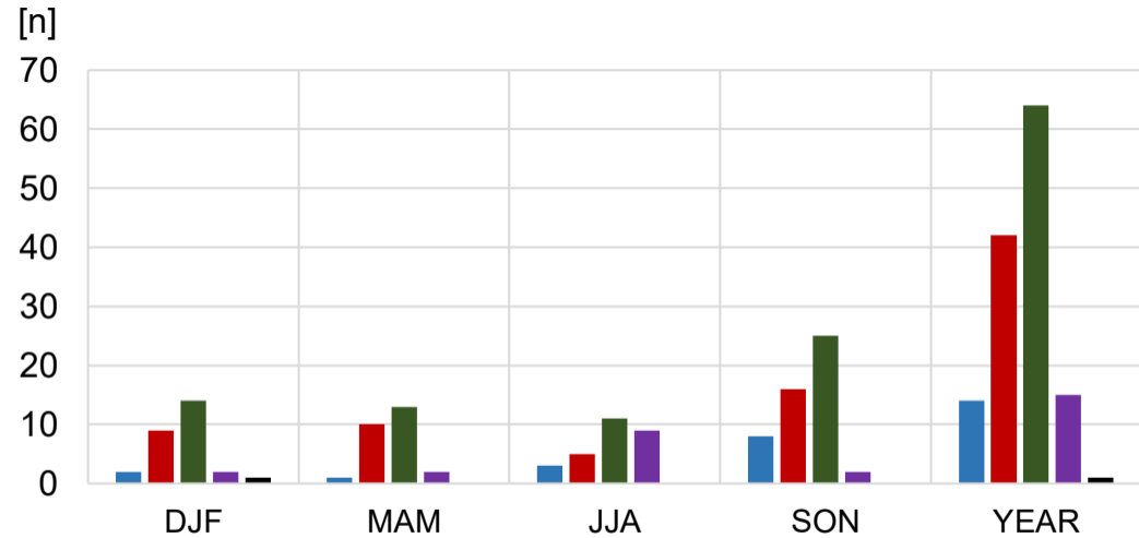
(b) Fresh and strong breeze Gale Storm Squall Tornado
