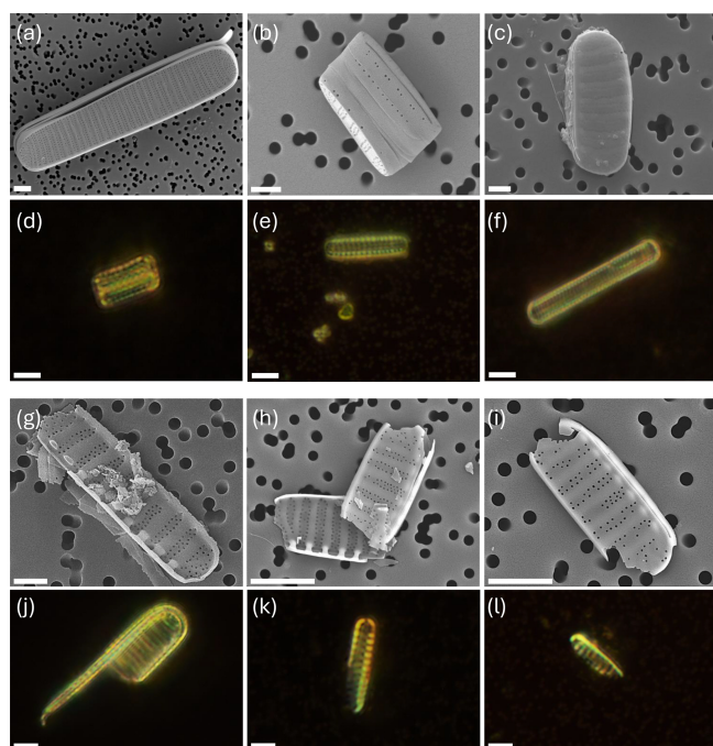
Figure 3. Scanning electron microscope (a, b, c, g, h, i) and optical microscope (d, e, f, j, k, l) images of entire diatom valves (a–f) and valve fragments (g–l). Scale bar: 1 \mu\text{m} for SEM images and 5 \mu\text{m} for optical images (magnification 1000 \times ).
