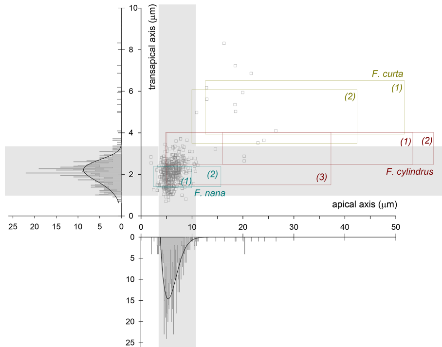
Figure 4. Morphometric data of entire valves from the RICE ice core. Apical axis ( \mu\text{m} ) vs. transapical axis ( \mu\text{m} ). Frequency histograms (bottom and left) are also reported. Grey bands indicate the interval where 95 % of specimens are included. Boxes marked with (1) refer to morphometric data for F. cylindrus , F. nana , and F. curta from Cefarelli et al. (2010); boxes marked with (2) refer to morphometric data from earlier literature collected and listed in Cefarelli et al. (2010). The box with (3) refers to data from Lundholm and Hasle (2008) for F. cylindrus .
