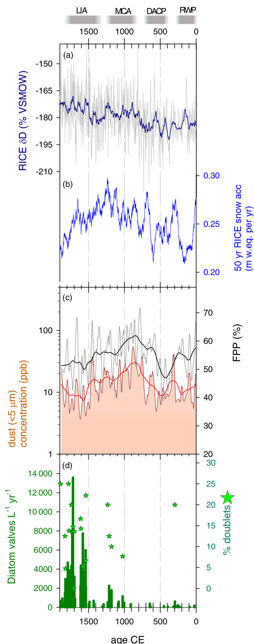
Figure 2. The climate history of RICE over the past 2 kyr. RWP: Roman Warm Period; DACP: Dark Ages Cold Period; MCA: Medieval Climate Anomaly; LIA: Little Ice Age. (a) RICE water stable isotope record ( \delta D ‰ VSMOW; blue line: 50-year running mean); (b) snow accumulation at the site (50-year running mean). (a, b) Data from Bertler et al. (2018). (c) Dust size index FPP (%) defined as in Delmonte et al. (2017), light grey. 20-year running mean and local smoothing (loess, polynomial degree 1, sampling proportion 0.1), black. Concentration (log) of dust particles smaller than 5 \mu\text{m} , dark red. 20-year running mean and loess local smoothing as in panel (c), red. (d) Diatom content of samples, expressed as number of diatom valves per litre per year. Green stars indicate the percentage of doublets in the samples. Panels (c) and (d) are generated from data obtained in this work; these are reported in Tables S1 and S2.
