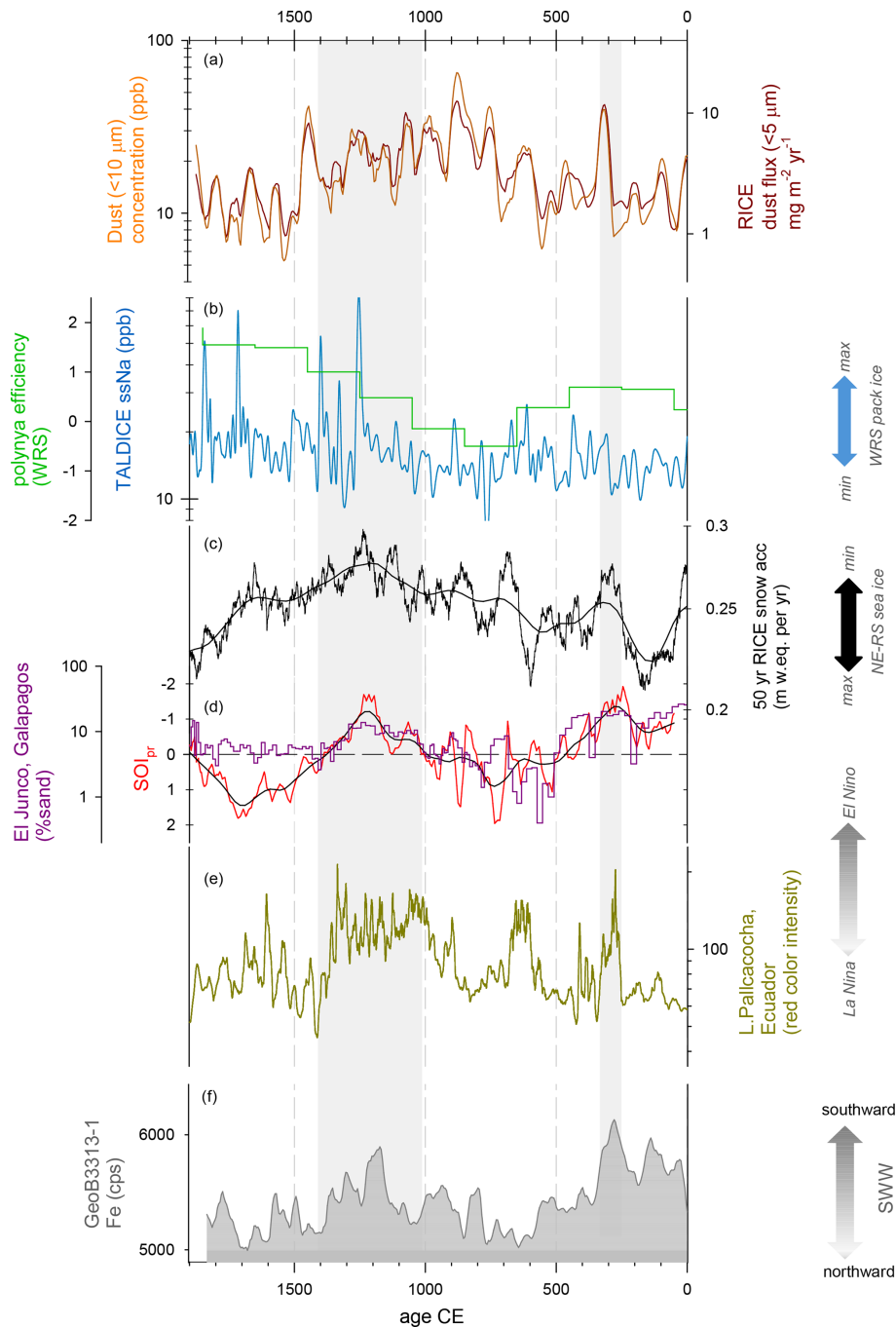
Figure 5. Comparison of ice core and climate records from the Southern Hemisphere over the last 2000 years. (a) RICE concentration of dust particles smaller than 10\ \mu\text{m} (ppb) and RICE flux ( \text{mg m}^{-2}\ \text{yr}^{-1} ) of particles smaller than 5\ \mu\text{m} (30-year running average). (b) Sea salt sodium (ssNa) concentration at TALDICE (and polynya efficiency; Mezgec et al., 2017). (c) RICE snow accumulation rate, as in Fig. 2b. (d) Red line: Southern Oscillation Index ( \text{SOI}_{\text{pr}} ) record (with loess smooth superposed, black line) from Yan et al. (2011). This index was calculated as the difference between the reconstructed precipitation records from Indonesia and the Galápagos (see text). Purple line: rainfall history of the Galápagos, used in the reconstruction of \text{SOI}_{\text{pr}} but extending for a longer time period. This series is derived from a lake-level reconstruction based on grain size data from Lago El Junco sediment core. (e) Laguna Pallcacocha (Ecuador) red colour intensity record of sediments (Moy et al., 2002; 30-year running average). El Niño-related high-precipitation events are related to greater colour intensities. (f) Iron content from GeoB3313-1 core smoothed over a 20-year running average (Lamy et al., 2001); higher Fe concentrations indicate a poleward position of the southwesterly winds (SWW) and vice versa.
