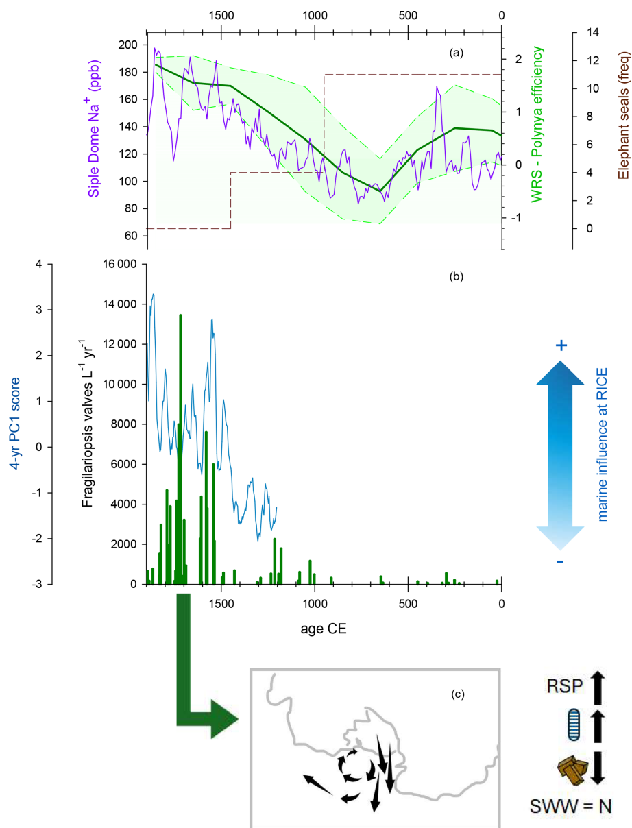
Figure 6. (a) Polynya efficiency (Mezgec et al., 2017) with standard deviation values, derived from a stacked record of F. curta from the landfast sea ice zone of the western Ross Sea and ssNa record from Taylor Dome (see Mezgec et al., 2017, for details). Elephant seal frequency data from Hall et al. (2006; as reported in Mezgec et al., 2017). Sodium data from Siple Dome are also reported (Kreutz et al., 1997). (b) First principal component obtained from the 4-year-resolved ICP-MS data series (Brightley, 2017) spanning the period 1204–1992 CE; PC1 explains 62 % of the variance and is related to marine-sourced winds (see text). Green histograms refer to the number of entire Fragilariopsis spp. valves per litre per year (same as in Fig. S5c). (c) Qualitative sketch of the atmospheric circulation pattern leading to expansion of the Ross Sea polynya and diatom transport to RICE. Arrows on the right show expansion of the Ross Sea polynya, an increase in aeolian diatom content, a decrease in dust influx, and a northward shift in the southwesterlies.
