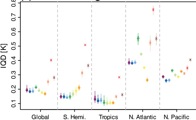
(c) Millennial magnitude deviations
