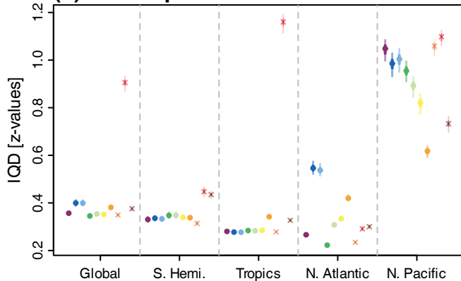
(b) Orbital pattern deviations
