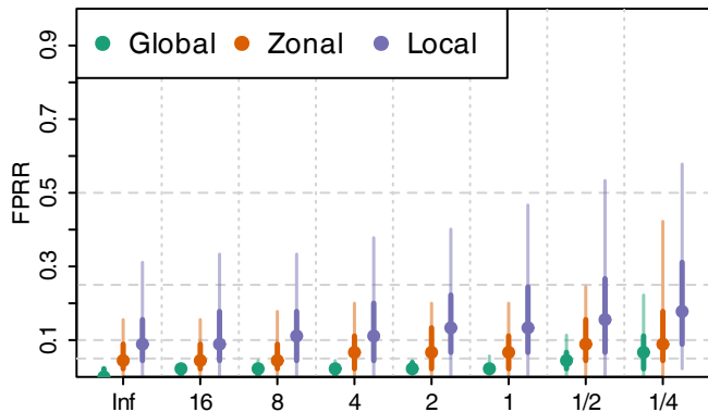
(a) Orbital magnitude
