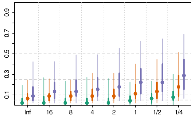
(b) Orbital pattern
