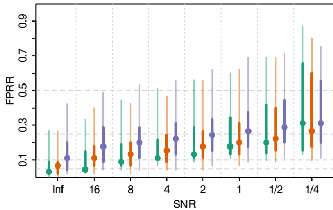
(c) Millennial magnitude
