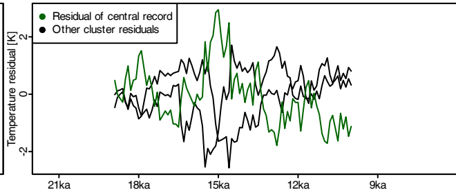
(b) Residuals from cluster mean, SNR: 1.6, decorr. length: 678 yrs
