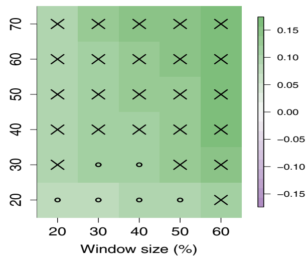
(b) Lag-1 autocorrelation
