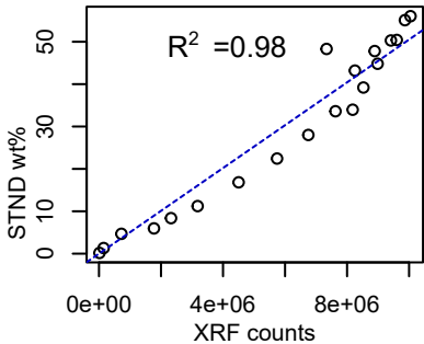
CaO
