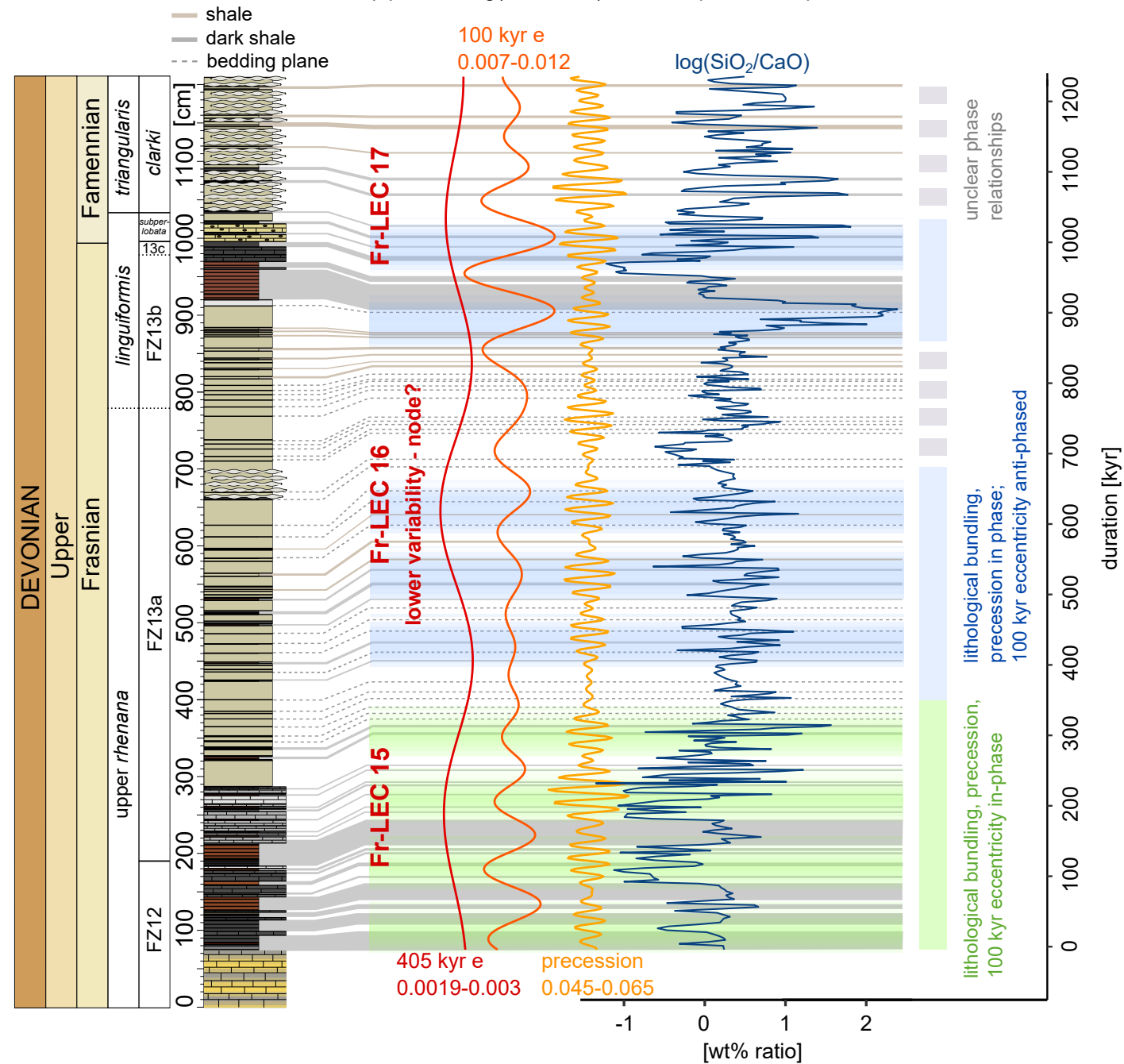
(a) Lithology
