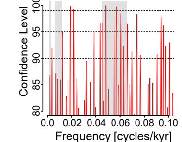
(e) Harmonic F Test Confidence Level Estimates
