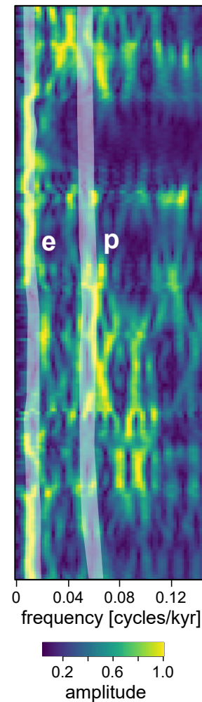
(b) EHA (MTM) based on precession tracing tbw=2, window = 150 kyr, normalized ampl., step = 5 kyr.
