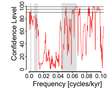
(e) Harmonic F Test Confidence Level Estimates
