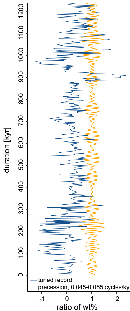
(a) Tuned log SiO 2 /CaO and bandpassed precession
