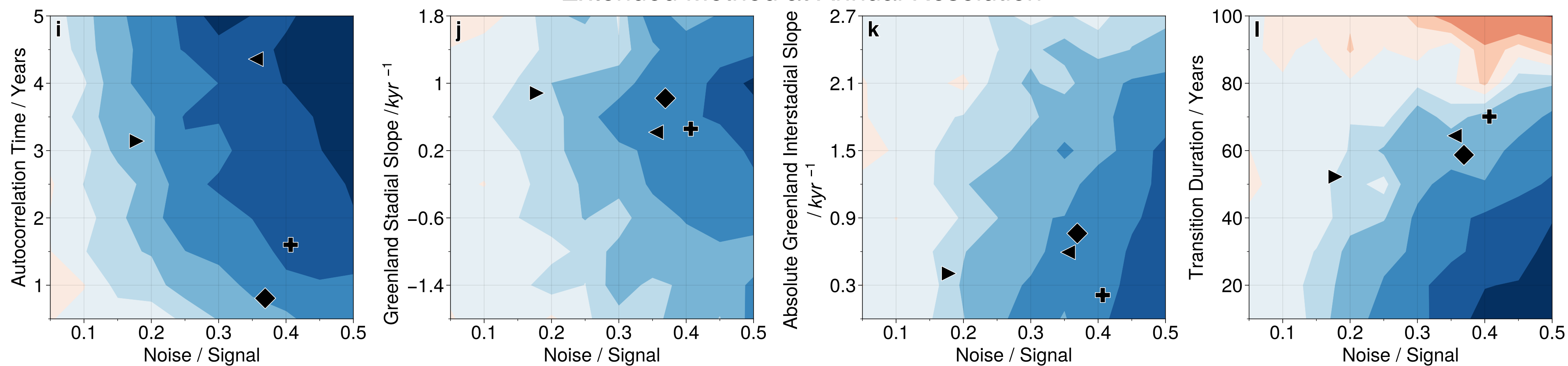
Extended Method at Decadal Resolution
