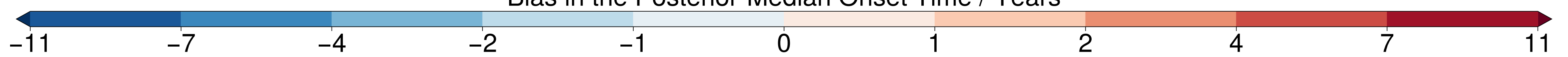
Bias in the Posterior-Median Onset Time / Years
