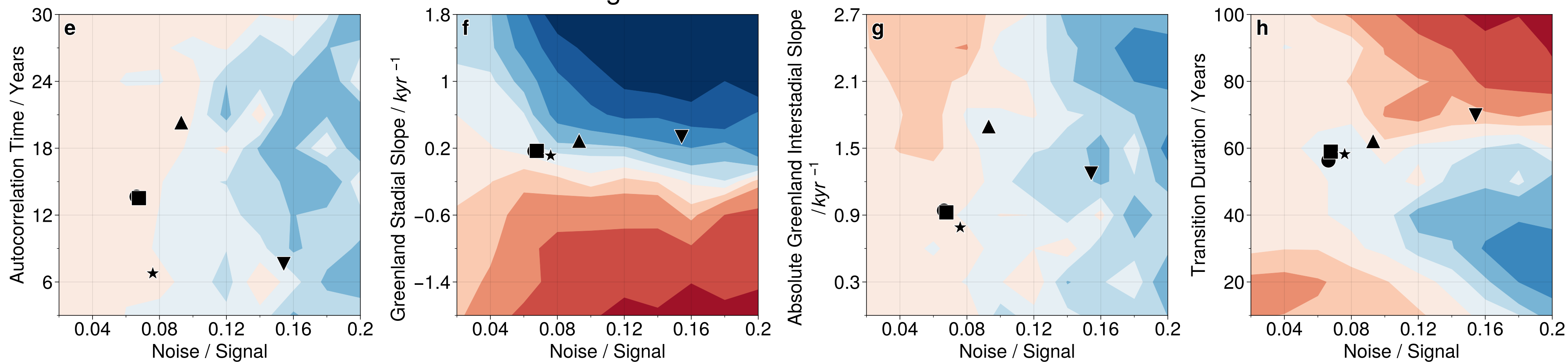
Extended Method at Annual Resolution
