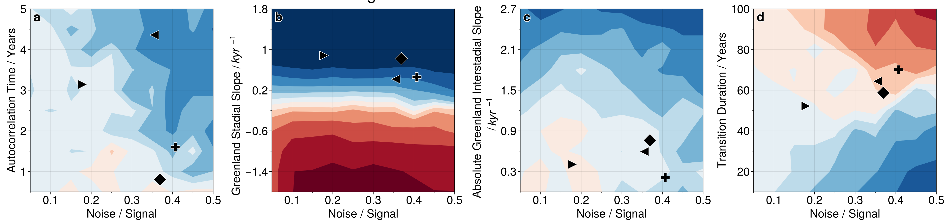
Original Method at Decadal Resolution
