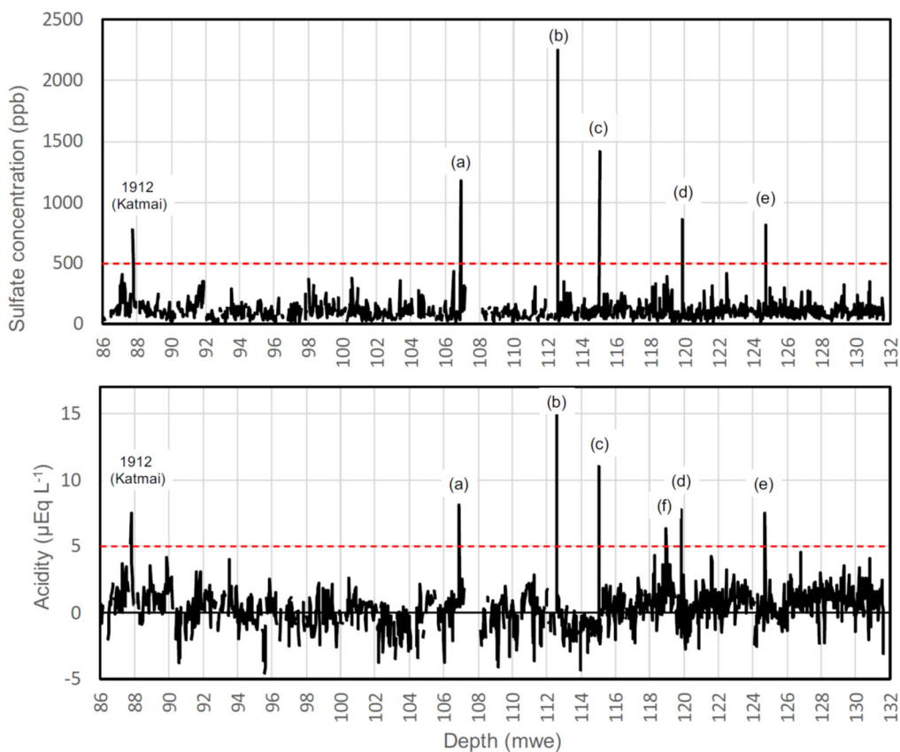
Figure S2. Raw profiles of sulfate and acidity in the Elbrus ice between 86 and 132 mwe. Samples considered to be impacted by large dust events has been removed (see Preunkert et al., 2019). In addition to the 1912 Katmai volcanic horizon at 87.75 mwe, several ice layers revealed sulfate concentrations exceeding 500 ppb (denoted (a) to (e)), and acidity higher than 5 \mu\text{Eq L}^{-1} (denoted (a) to (f)) that would be related to other volcanic events (see Table 1). The horizontal red dashed lines indicate the sulfate concentration limit of 500 ppb, the acidity limit of 5 \mu\text{Eq L}^{-1} .
