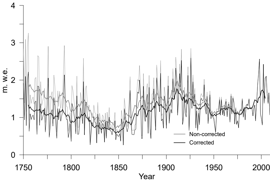
Figure S6. Reconstruction of annual snow accumulation at the WP non-corrected and corrected for snow accumulation surface distribution (section 2.3.2)
