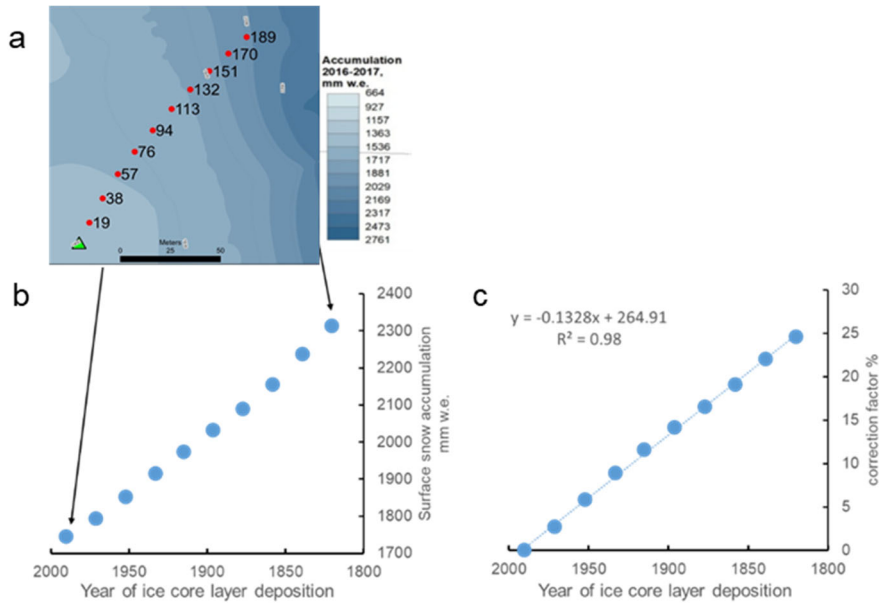
50 Figure S5. Surface snow accumulation distribution in 2016-2017 (Lavrentiev et al., 2022) (a), surface snow accumulation corresponding to age when the ice core layer was deposited on the glacier surface (b); correction to account for the surface accumulation distribution (c).
