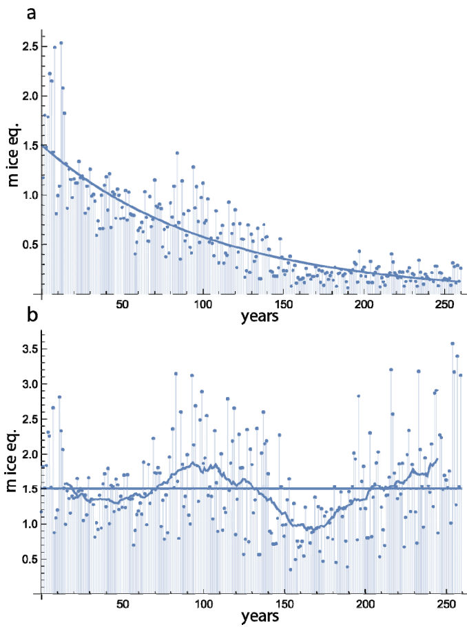
40 Figure S3. Thickness of an annual layer as a function of age. Measured layer thickness in ice equivalent (a) and annual layer thickness corrected by the model of J. Nye (Nye, 1963; Dansgaard and Johnsen, 1969) (b)
