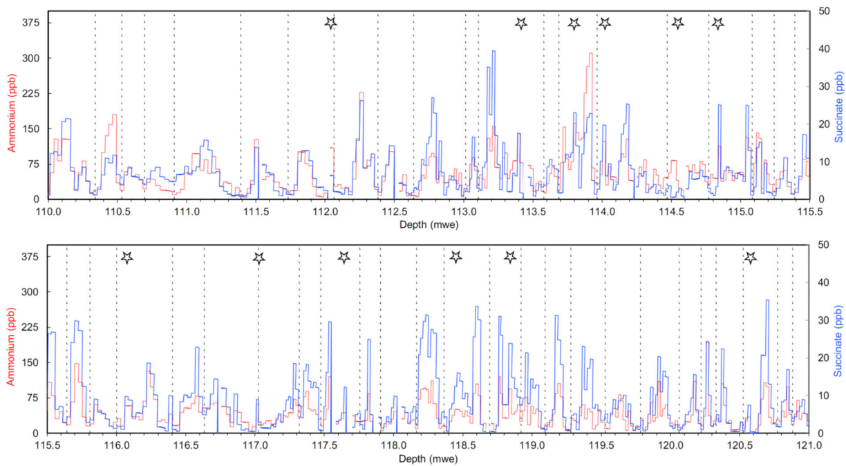
Figure S1. Annual layer counting between 110 and 121 mwe from co-authors A5 and A3. Vertical dashed lines denote yearly dissection proposed by co-author A5 based on identification of winter layers characterized by low concentrations of ammonium and succinate. Stars indicate where co-author A3 counted additional years with respect to those counted by co-author A5.
