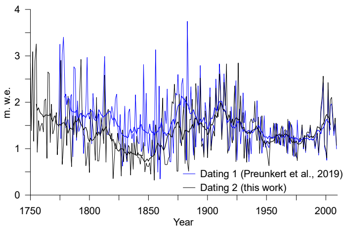
45 Figure S4. Reconstruction of annual snow accumulation at the WP using the A5 (Preunkert et al., 2019) and A4 (this work, see section 2.2.1) chronologies. 10-year moving averages are shown in thick lines.
