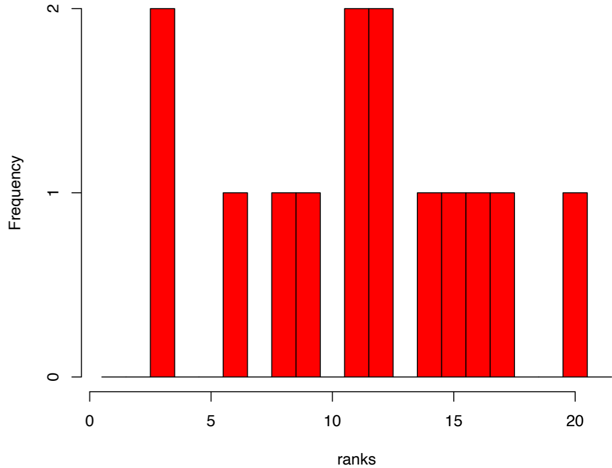
Rank histogram for PlioVAR–UK37 data with recentred ensemble
