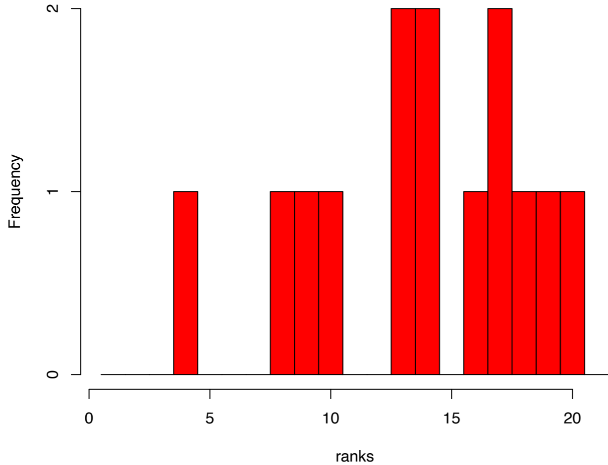
Rank histogram for PlioVAR–UK37 proxy data with PlioMIP ensemble
