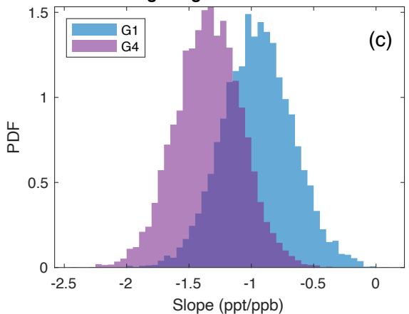
Same Age Regression below 1200 m
