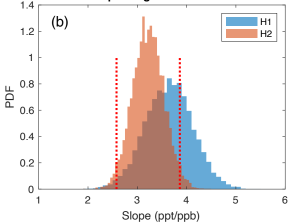
Same Age Regression above 800 m
