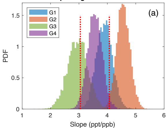
Same Age Regression below 1200 m
