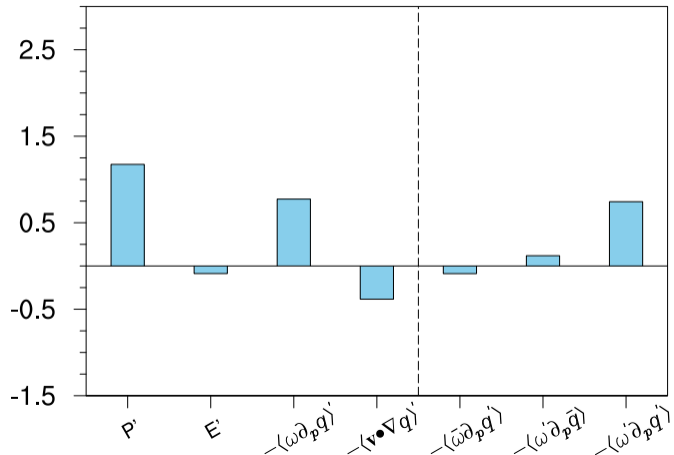
(b) Moisture budget (HM100-HM0)
