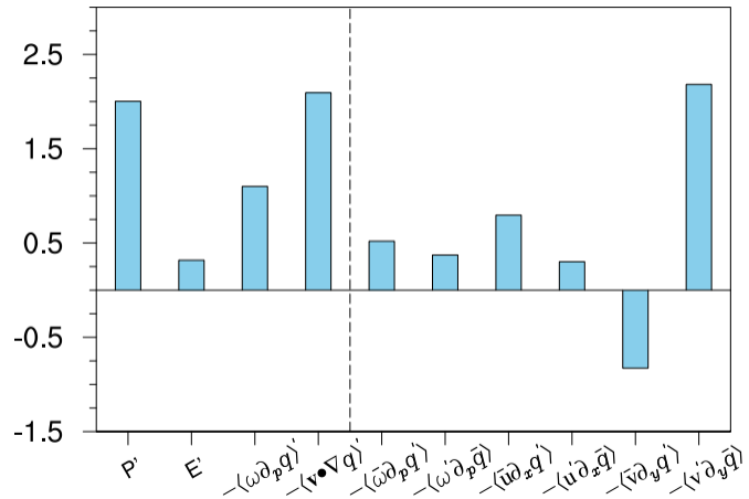
(a) Moisture budget (IP100-IP0)
