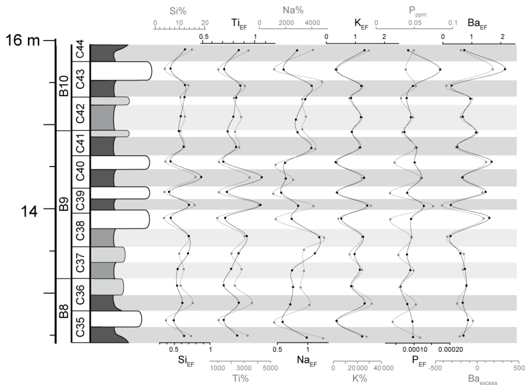
Figure 9. Lithological log of the Santiurde interval studied in detail, showing fluctuations in the percentage of elements related to detrital input (Si, Ti, Na, and K), palaeoproductivity (P and Ba), and their enrichment factors (EFs). The Ba_{excess} ratio is also presented.
