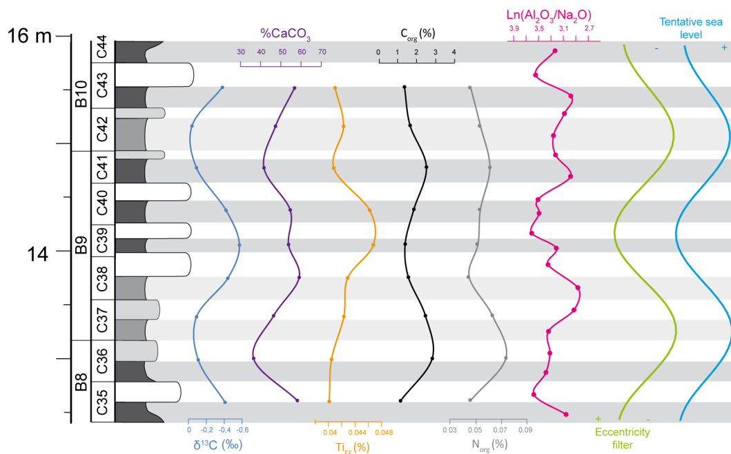
Figure 14. Lithological log of the Santiurde interval studied in detail, showing the average value per couplet of \delta^{13}\text{C}_{\text{carb}} , \% \text{CaCO}_3 , \text{Ti}_{\text{EF}} , \text{C}_{\text{org}} and \text{N}_{\text{org}} . The palaeo-weathering index \text{Ln}(\text{Al}_2\text{O}_3 / \text{Na}_2\text{O}) of all beds, the short eccentricity colour filter output (Fig. 5), and a tentative sea level curve are also shown.
