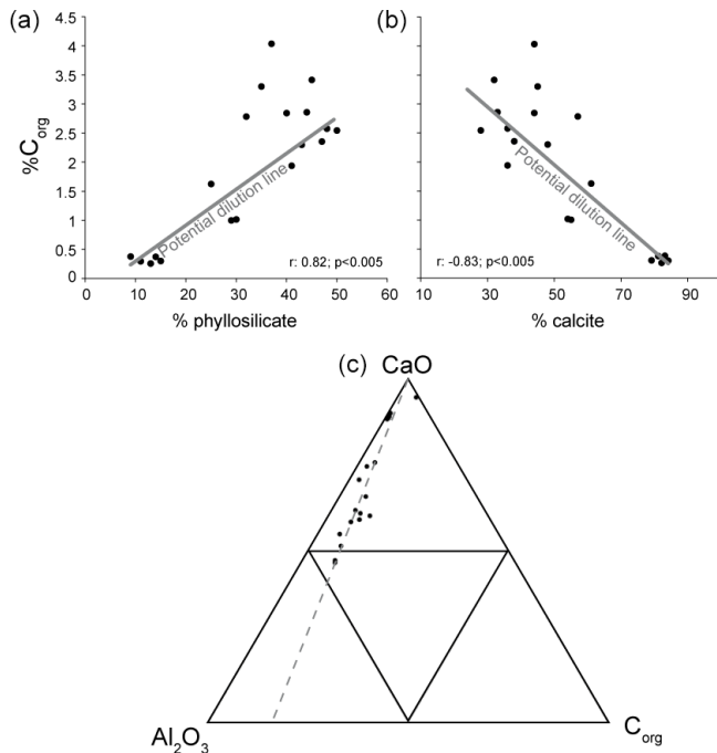
Figure 12. Cross-plot of C org against (a) phyllosilicate and (b) calcite content. Potential dilution lines of C org are marked in both graphs. (c) Ca–Al–C org ternary plot with Santiurde samples, which follow a constant C org / Al 2 O 3 .
