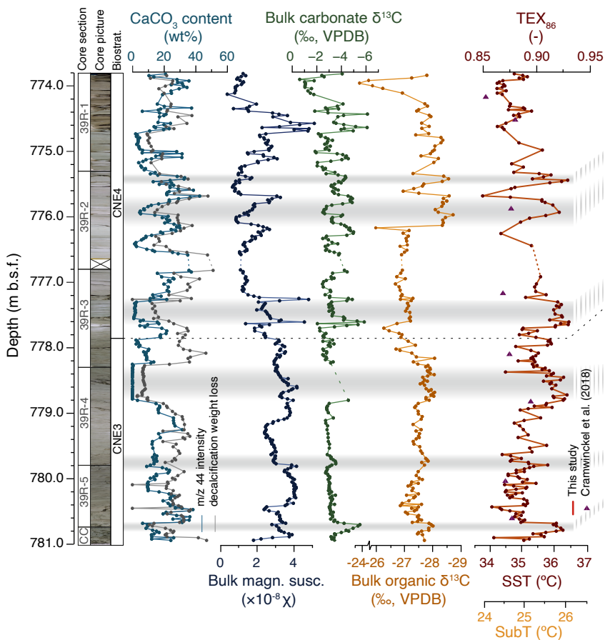
(a) Site 959
