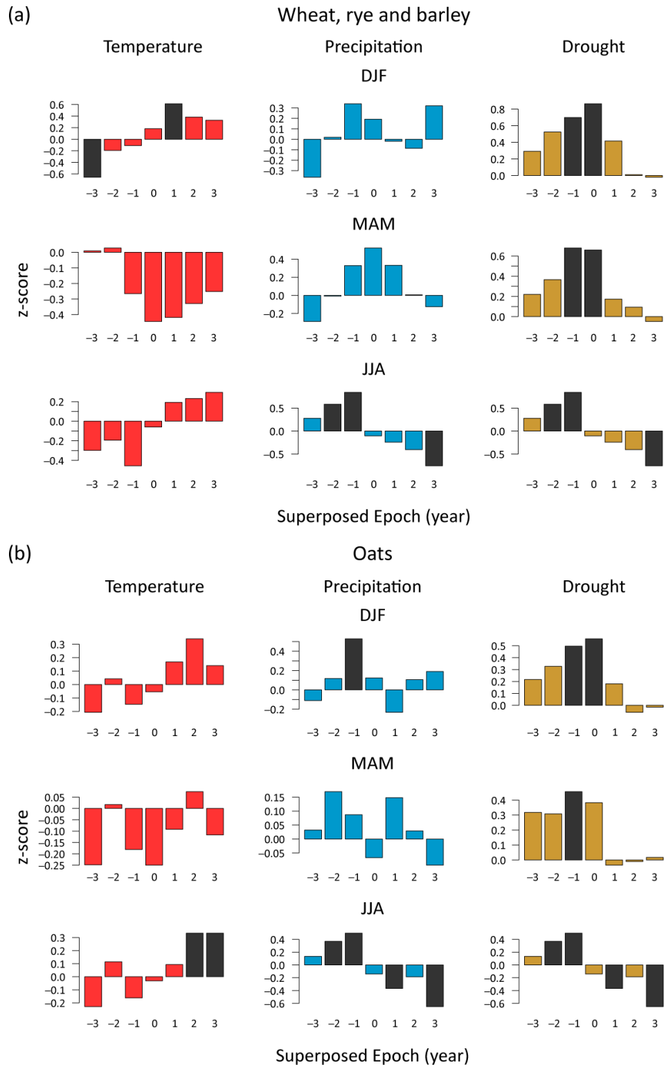
Figure 8. Superposed epoch analysis of seasonal (DJF – winter; MAM – spring; JJA – summer) temperatures, precipitation, and scPDSI in the Czech Lands from 1725–1824 CE, aligned with years of extremely high prices (0 – event year) for wheat, rye, and barley (a) and for oats (b). The individual columns display mean climate conditions 3 years before and after the event years. Climate variables were transformed into z scores, and significant anomalies ( p < 0.05 ) are indicated in black.
