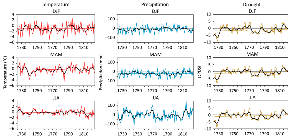
Figure 7. Fluctuations and linear trends in mean winter (DJF), spring (MAM), and summer (JJA) temperatures, precipitation totals, and scPDSI in the Czech Lands during the period 1725–1824 CE. These are displayed as deviations relative to the 1961–1990 reference period and smoothed with a 10-year Gaussian filter.
