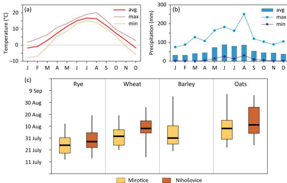
Figure 3. Annual variations in monthly mean temperatures (a) and precipitation totals (b) in Sušice (avg – monthly mean; max – absolute monthly maximum; min – absolute monthly minimum) (data source: In-počasí, 2023). (c) Boxplots (maximum and minimum, upper and lower quartiles, median) of the start dates of the harvest for four main cereals in Mirotice and Nihošovice (excluding barley) for the period 1951–1980 (data source: CHMI database FENODATA).
