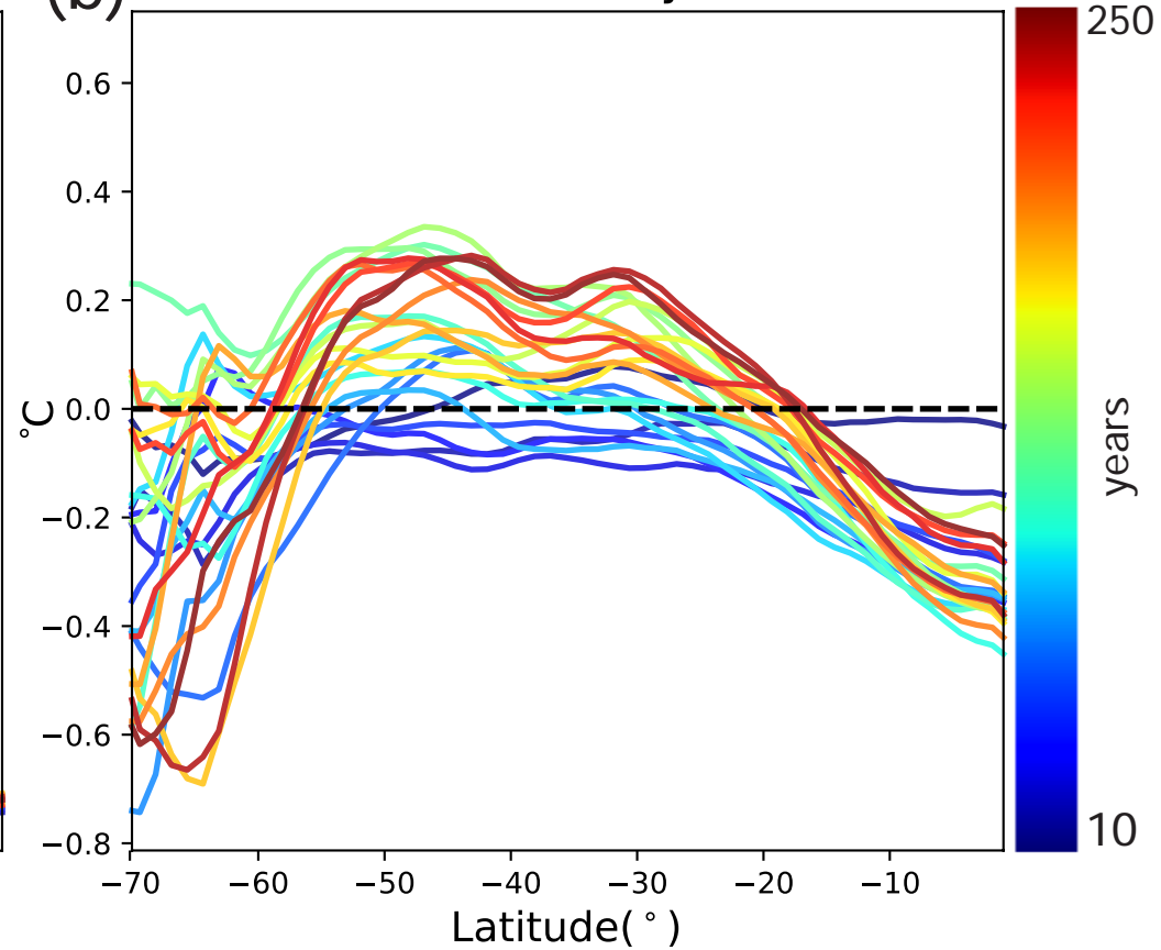
(b) SAT anomalies 10-year mean
