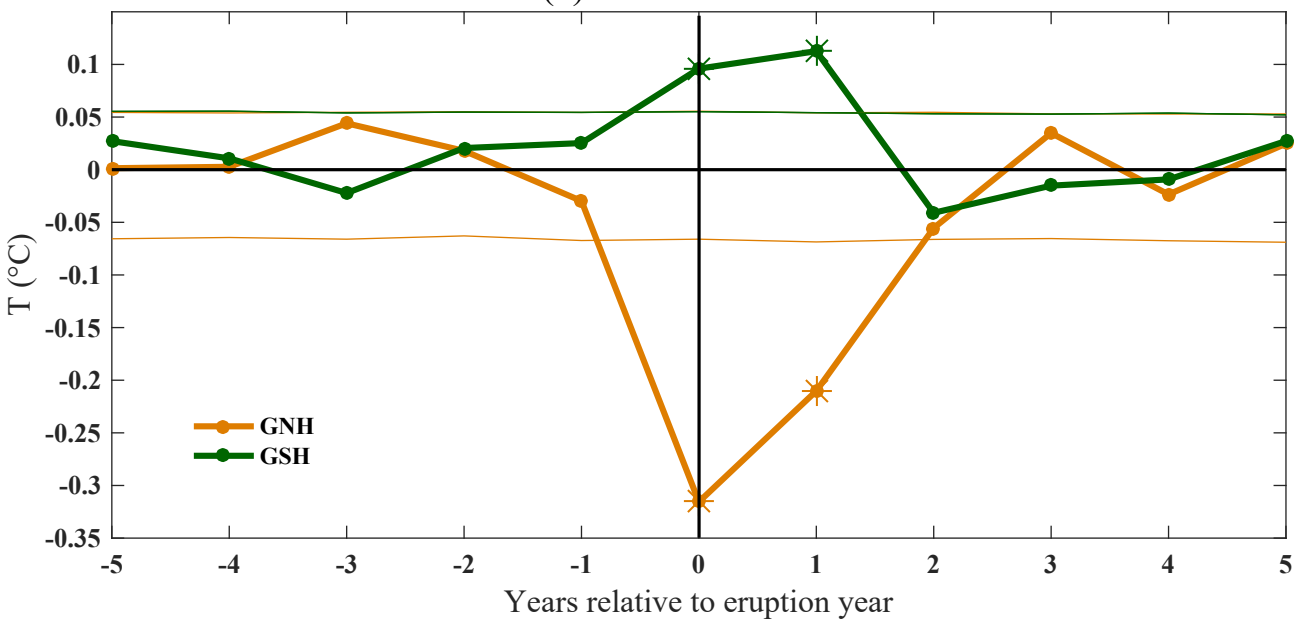
(b) ASM land-ocean
