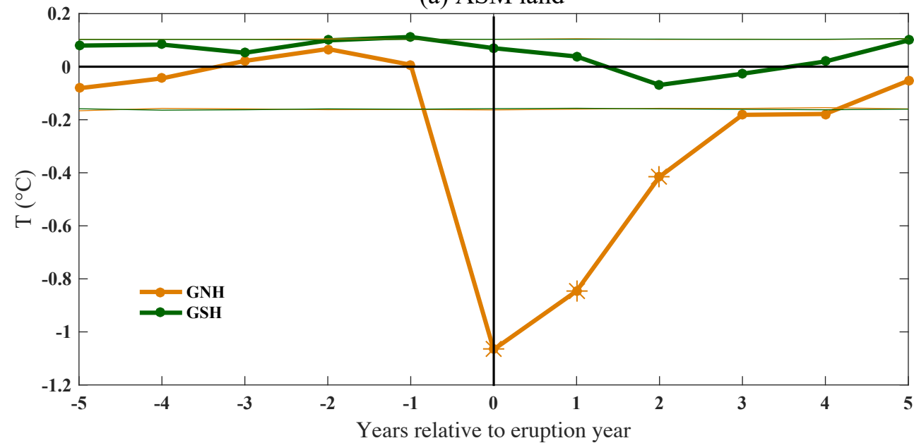
(a) ASM land
