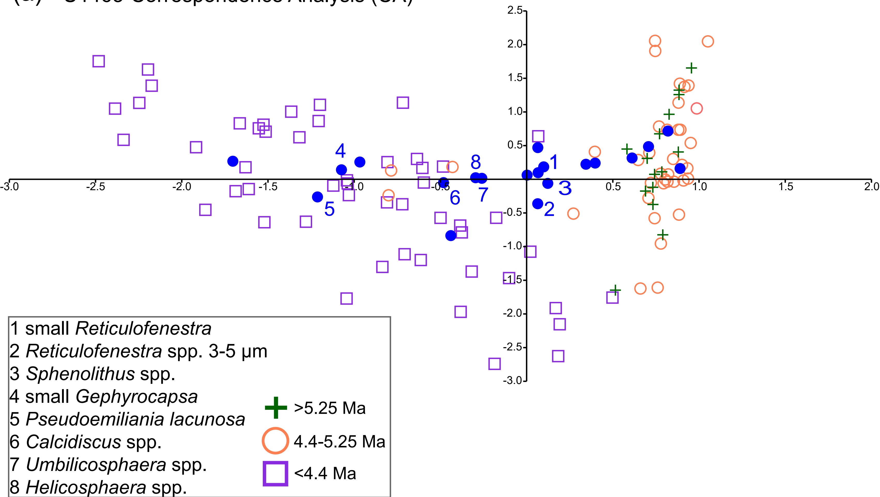
(a) U1463 Correspondence Analysis (CA)
