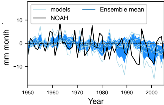
(a) (Reference: 1950-1979 CE)
