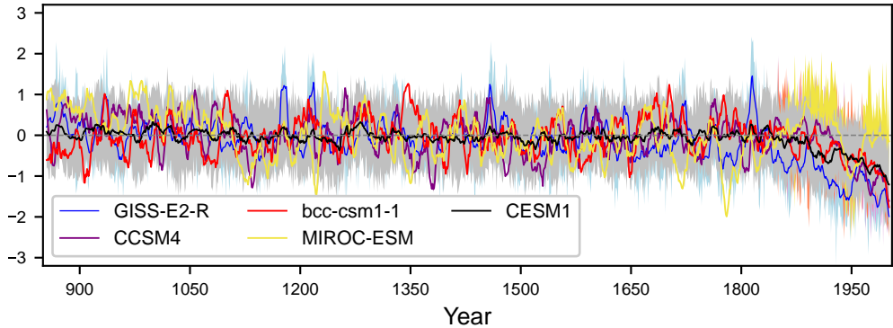
(b) Standardized soil moisture anomaly (Reference: 850-1849 CE)
