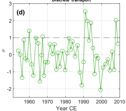
Res Discrete transport
