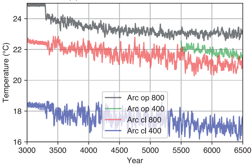
(c) N. Atlantic SST near Site 647
