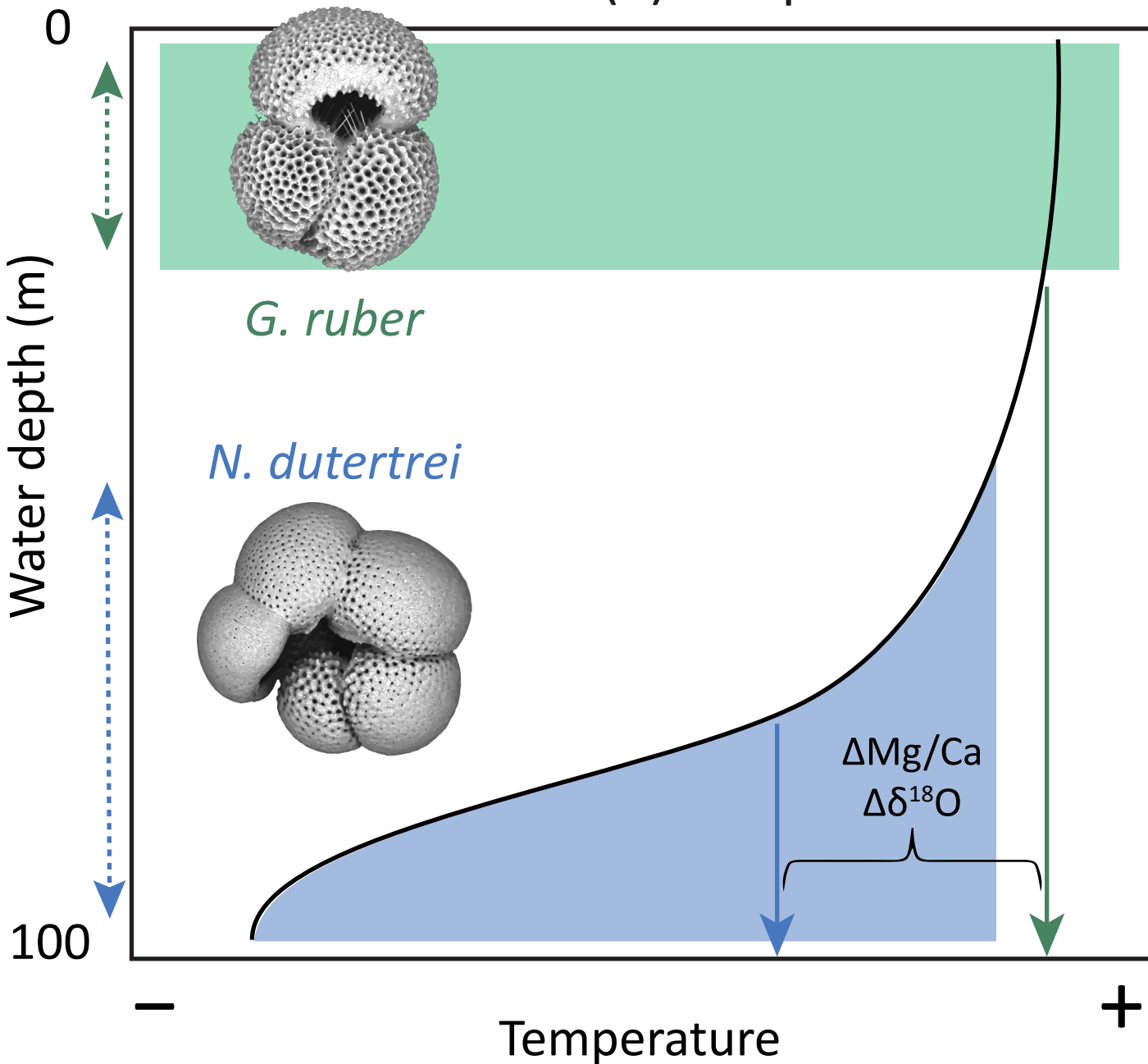
(a) Deep thermocline
