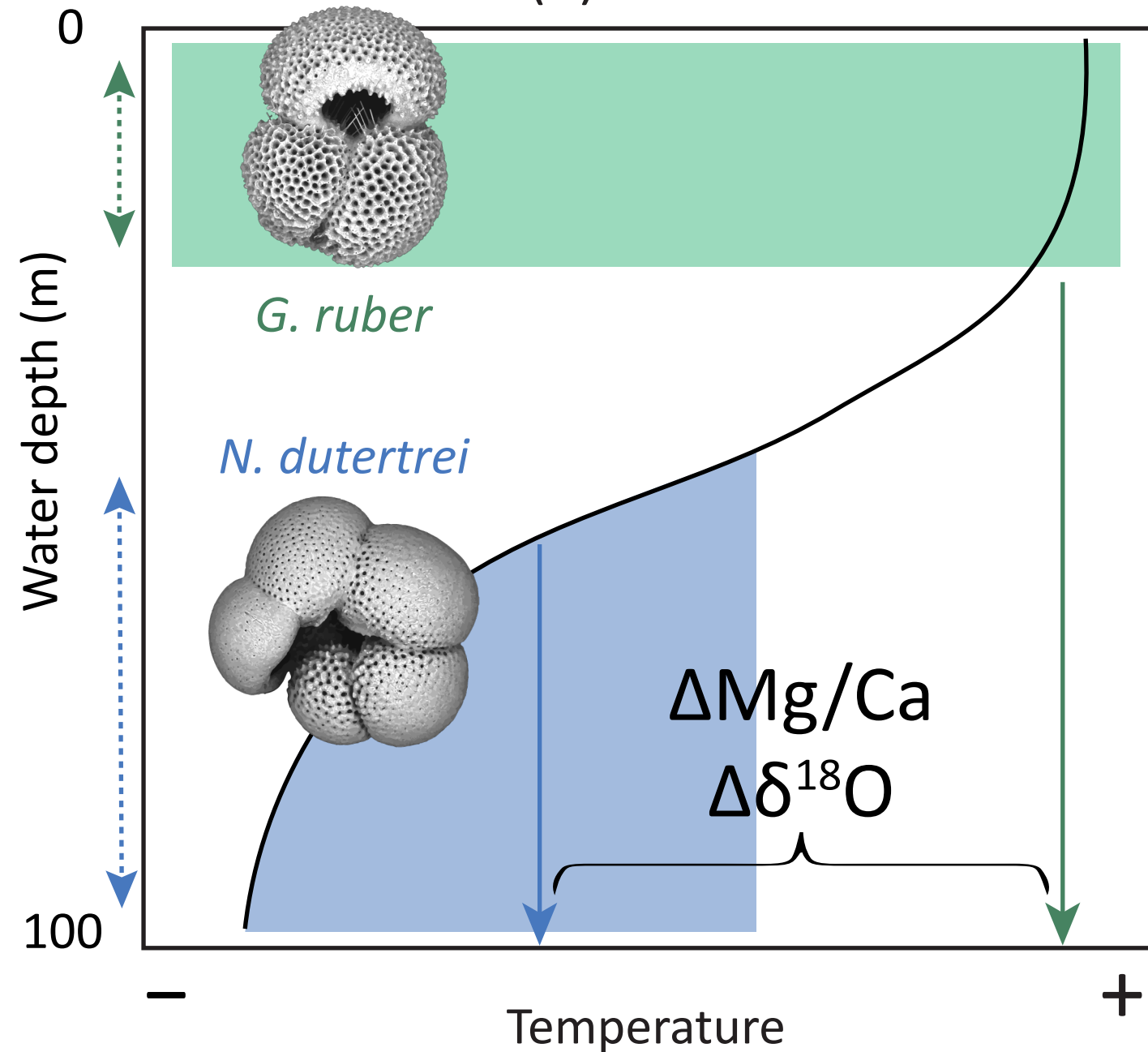
(b) Shallow thermocline
