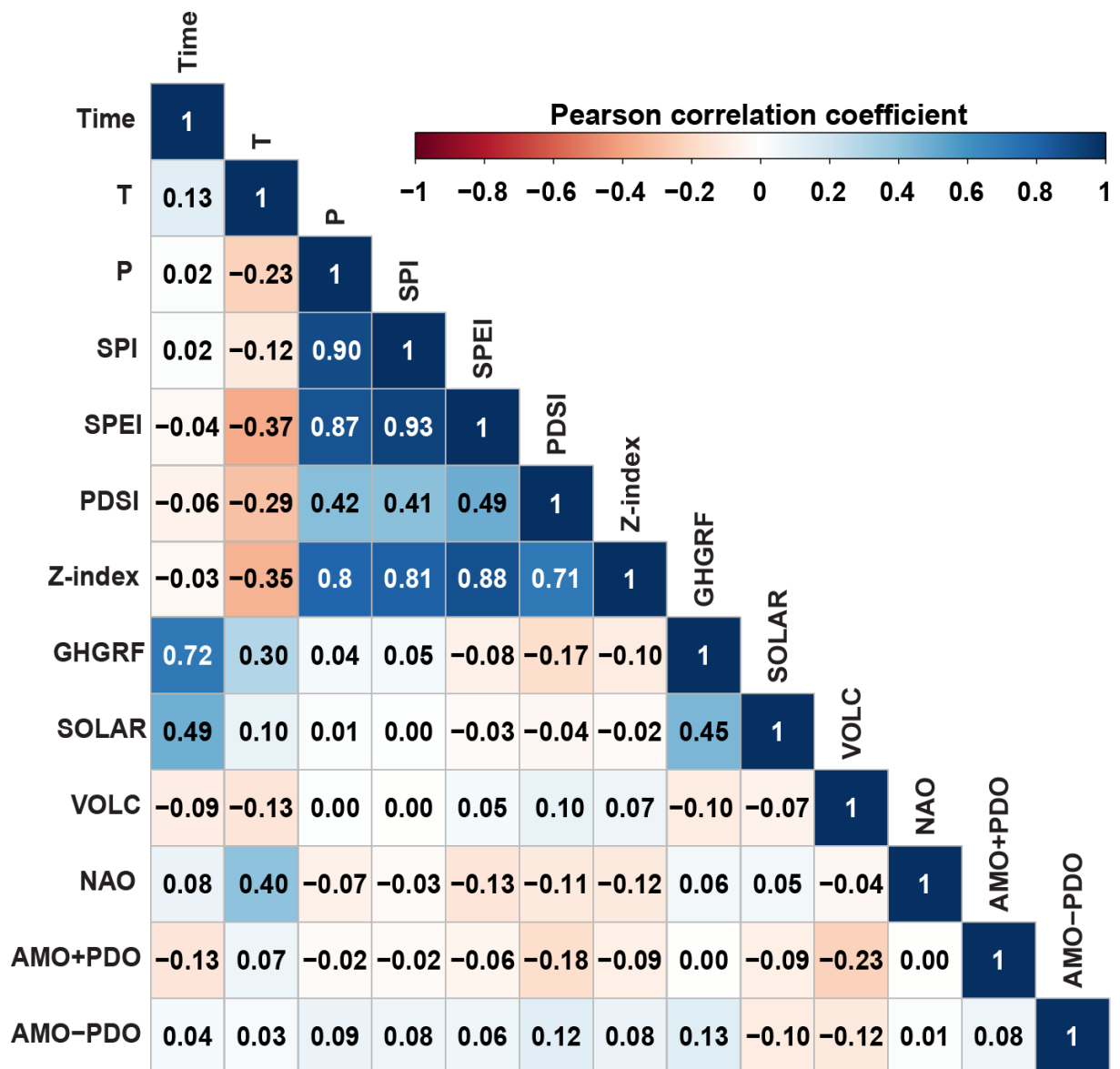
Figure S1. Pairwise Pearson correlation coefficients between individual targets and explanatory variables in seasonal time steps (see Fig. 2 for correlations in annual time steps).
