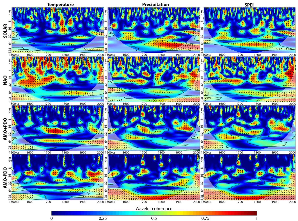
Figure S2. Wavelet coherence between series of temperature, precipitation or SPEI and explanatory variables with prominent oscillatory components (all seasons). Arrows show local phase shifts of the two series (only displayed for coherences in excess of 0.5); areas with statistically significant coherences are enclosed by black lines (95% confidence level).
