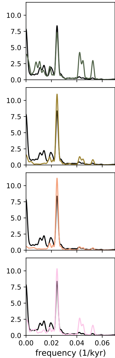
(c) Spectral analysis prior to the MPT
