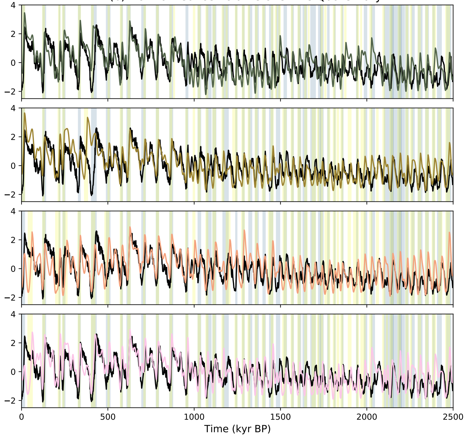
(b) Normalized ice volume over the Quaternary
