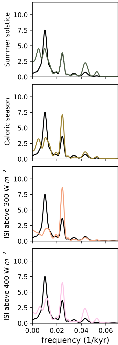
(a) Spectral analysis after the MPT
