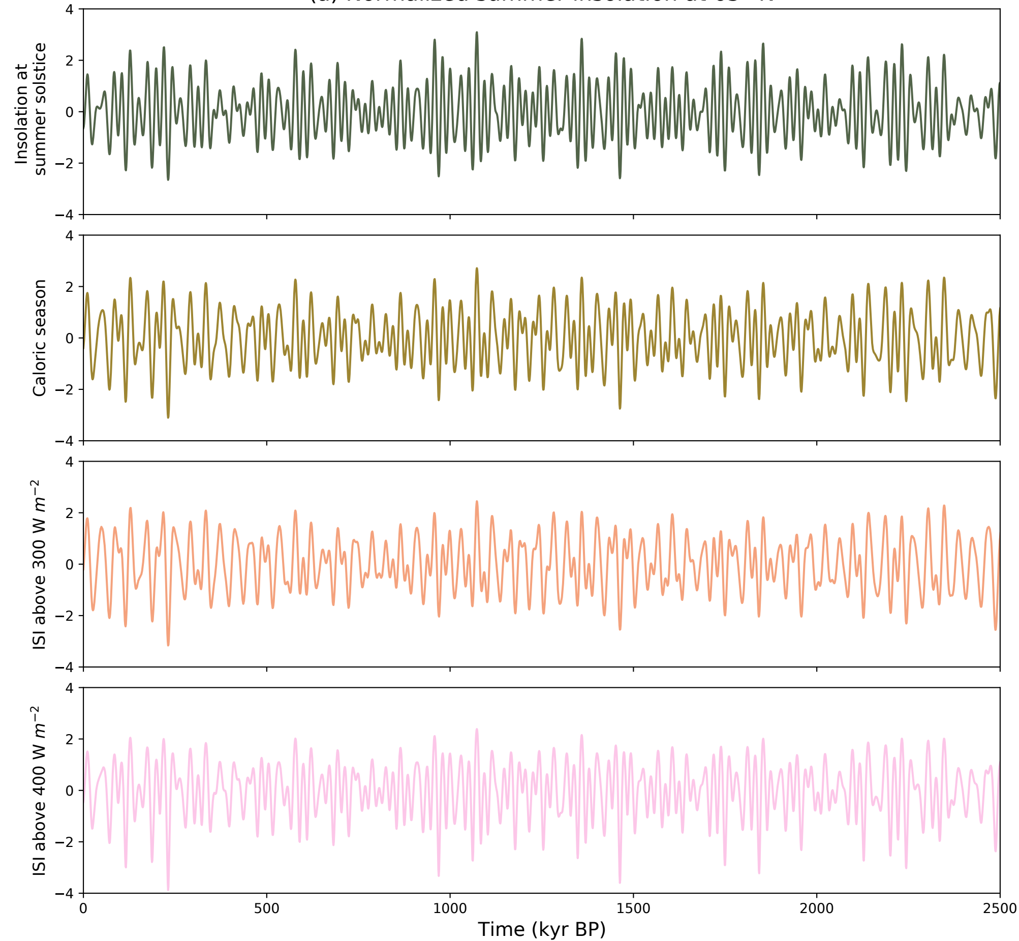
(a) Normalized summer insolation at 65° N
